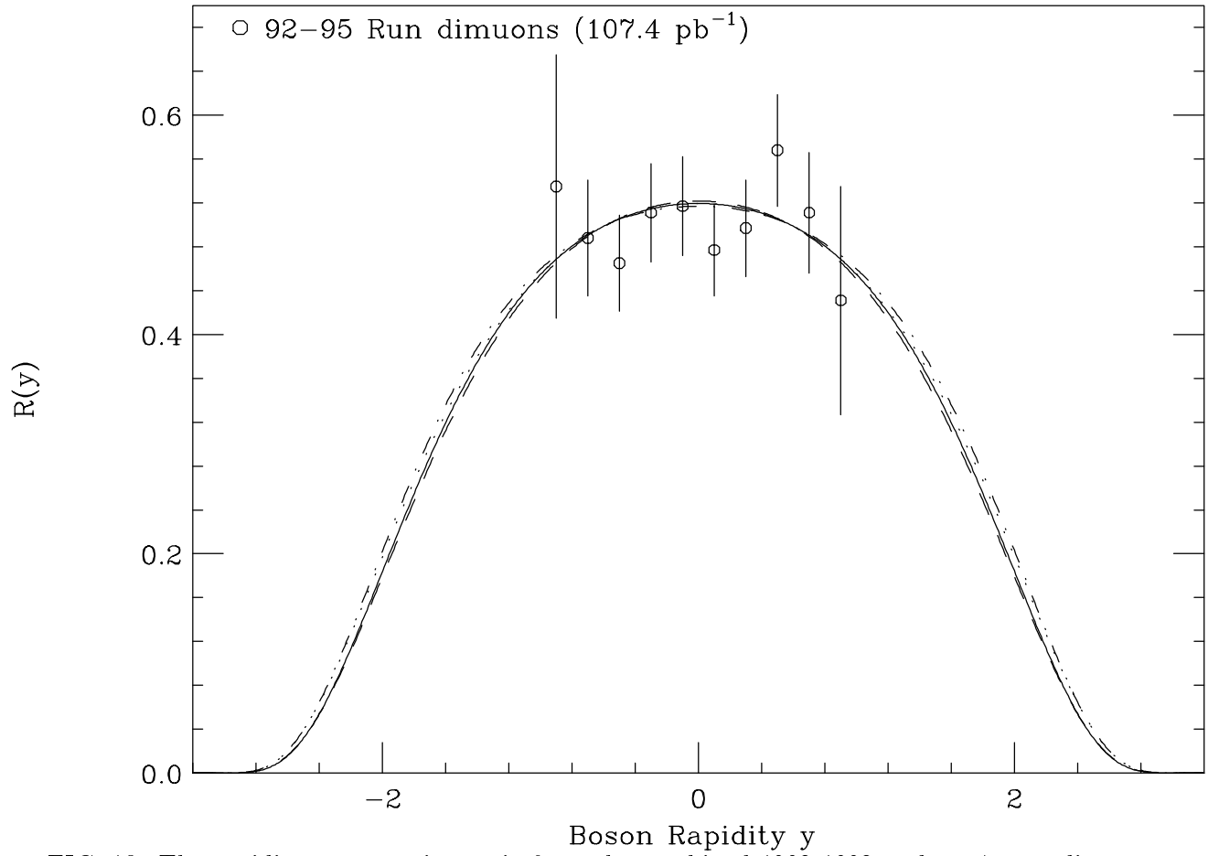
FIG. 10. The rapidity cross section ratio from the combined 1992-1993 and 1994-1995 dimuon data. The measurement is compared to leading order calculations with a K factor. The theoretical curves are calculated using the CTEQ-3L (dotted line), MRS-A (solid line), CTEQ-3M (dashed line), and MRS-D- ' (dot-dashed line) PDFs. The error includes only the statistical and the non-luminosity related systematic error.
