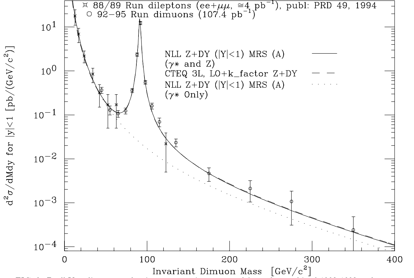
FIG. 8. Drell-Yan dimuon production cross section extracted from the combined 1992-1993 and 1994-1995 data. The solid line is the NLO QCD prediction. The dashed line is the LO QCD prediction with a K factor to account for higher order effects. The dotted line is the NLO QCD prediction without the contribution from Z^0 exchange.
