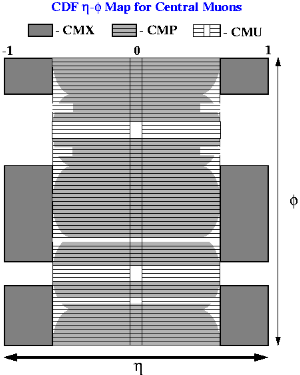
FIG. 2. The CDF Level 2 trigger coverage in \eta - \phi space for muons in the region of pseudo-rapidity |\eta| \leq 1 .
