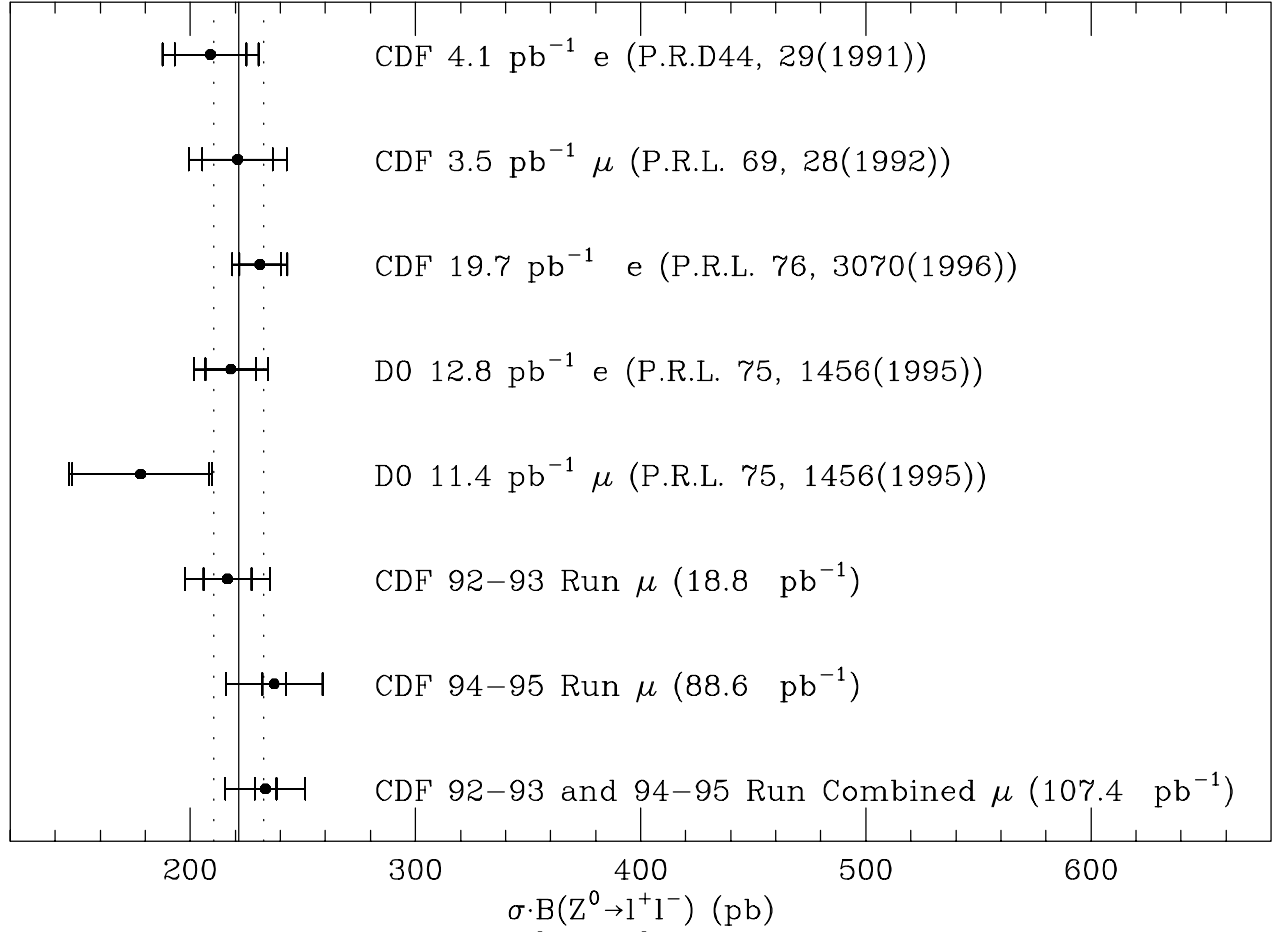
FIG. 7. Comparison of measured \sigma(Z^0) \cdot \mathbf{B}(Z^0 \rightarrow \mu^+ \mu^-) to predictions (solid line) using the next-to-next-to-leading calculation with the MRS-A parton distribution functions. The dotted lines are the theoretical uncertainty of \pm 5\% . Also shown are earlier measurements from CDF and D0. The inner error bar is the combined statistical and systematic uncertainty and the outer error bar includes the luminosity uncertainty.
