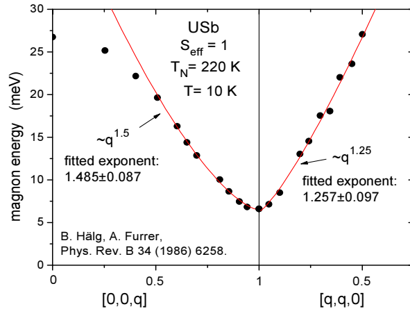
Figure 2. Magnon dispersions of antiferromagnetic USb measured at T=10 K along two crystallographic directions [11]. Along cube edge dispersion of the Goldstone bosons is \sim q^{1.5} while along face diagonal \sim q^{1.25} dispersion holds. The \sim q^{1.25} dispersion is consistent with T^2 dependence observed below T_{CO}=105 K for the magnetic order parameter (see text).
