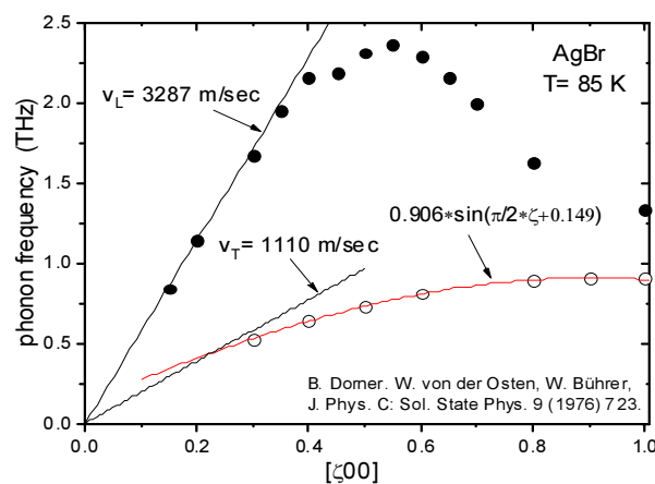
Figure 7. Dispersions of the acoustic phonons with longitudinal and transverse polarization of AgBr [18]. For longitudinal polarization the dispersion of the acoustic phonons agrees with the dispersion of the Debye bosons (sound waves) up to \sim 2 THz ( \sim 96 K). For transverse polarization interaction with Debye bosons necessitates a phase shift in the argument of the sine function.
