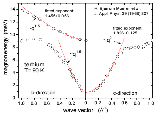
Figure 3. Magnon dispersions of terbium along hexagonal c-axis and transverse to c-axis (along b-direction) [13]. Assuming integer moment of J=6 according to electronic configuration of ^7F_6 of the Tb^{3+} ion, \sim q^2 dispersion is typical for the isotropic boson field but \sim q^{1.5} dispersion for the one-dimensional boson field in magnets with integer spin.
