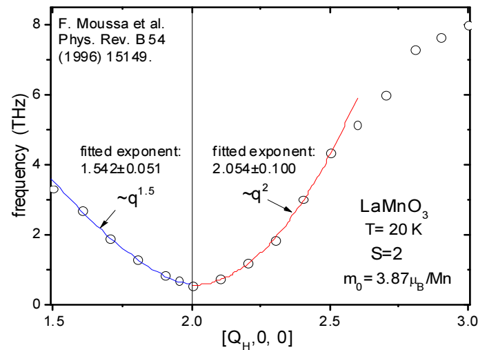
Figure 6. Magnon dispersions of orthorhombic \text{LaMnO}_3 with integer spin of S=2 [16]. The dispersion \sim q^2 is attributed to the isotropic boson field in magnets with integer spin. The dispersion \sim q^{1.5} belongs to the one-dimensional boson field.
