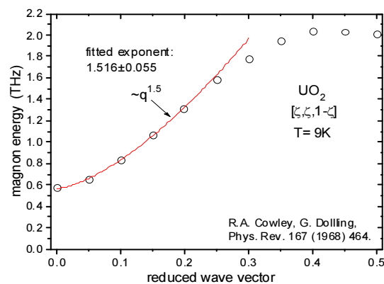
Figure 4. Magnon dispersions of nominally cubic UO_2 along body diagonal [15]. The observed \sim q^{1.5} dispersion is that of the one-dimensional boson field in magnets with integer spin ( S=1 ). This UO_2 sample was not perfectly cubic.
