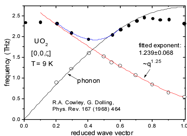
Figure 5. Magnon dispersions of UO_2 along cube edge revealing \sim q^{1.25} dispersion [15]. This dispersion is attributed to the anisotropic 3D boson field in magnets with integer spin ( S=1 ).
