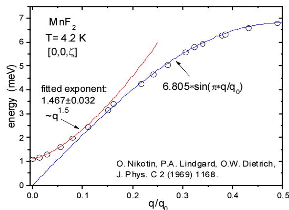
Figure 1. Functional crossover in the magnon dispersion curve of \text{MnF}_2 along tetragonal c -axis [8]. For small wave vector values magnon dispersion is given by gap value plus q^{1.5} power function. The q^{1.5} dispersion is that of the one-dimensional Goldstone boson field in magnets with half-integer spin ( S=5/2 ). For larger wave vector values magnon dispersion is excellently described by sine function of wave vector.
