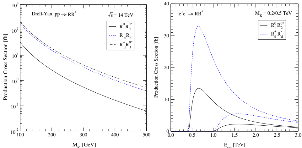
Fig. 2. Left: Drell–Yan production of the neutral/charged R -Higgs boson pairs, R_1^0 R_2^{0*} , R_d^+ R_d^- and R_d^+ R_1^{0*} , at the LHC ( \sqrt{s} = 14 TeV). The cross-sections are plotted versus the averaged mass of the produced particles denoted generically by M_R ; Right: Production of the neutral and charged R -Higgs boson pairs R_1^0 R_2^{0*} and R_d^+ R_d^- at TeV e^+e^- colliders [ILC/CLIC]. Two values, 0.2 TeV and 0.5 TeV, are taken for the masses.
