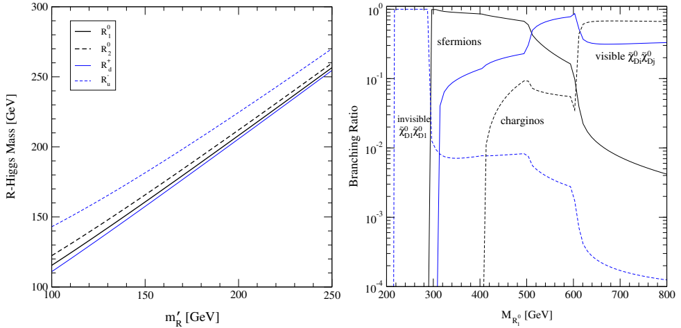
Fig. 1. Left: Masses of the two neutral R_{1,2}^0 and the two charged R_{d,u}^\pm Higgs bosons for a common R -Higgs mass parameter m'_R = (m_{R_{d,u}}^2 + \mu_{d,u}^2)^{1/2} ; Right: Branching ratios for decays of the neutral R_1^0 -Higgs boson to sfermions, Dirac neutralinos and charginos for the SPS1a' parameter point (sfermion mixing removed).
