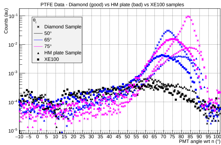
FIGURE 2.17: Resulting profiles of the measurements of the XENON100 sample [150] in comparison with the new steel tool milled "HM plate sample"(4 in table 2.1) and the "1st diamond"(3 in table 2.1). The rates are normalized with their beam normalization measurements (Gaussian fit). The positions of the specular peaks appear for the same incident angle at different angles. The diffuse component shows the same amplitude for all 3 samples.
