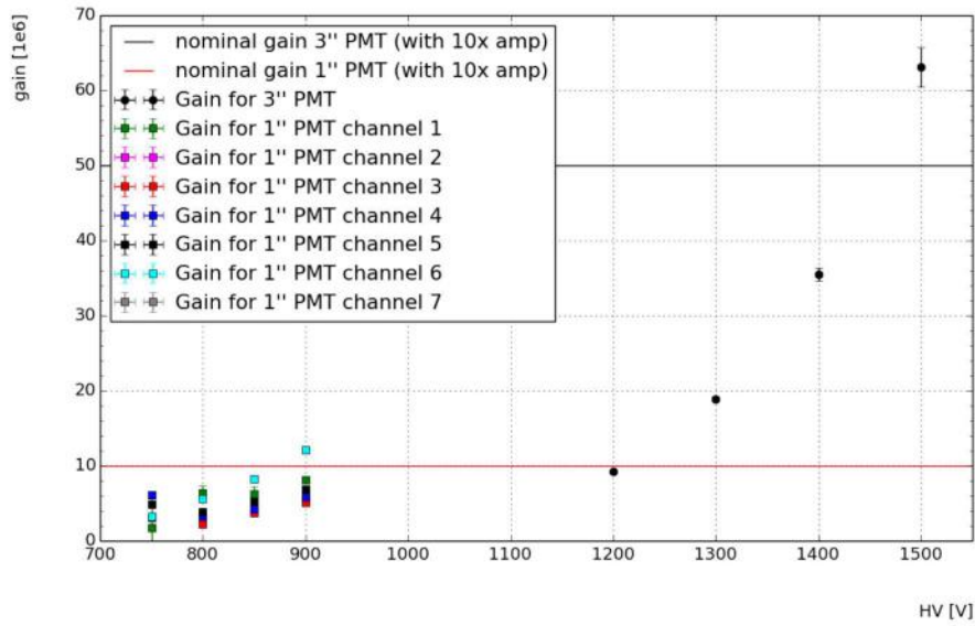
FIGURE 3.35: Gains as derived for all 1" and the 3" PMT in cold GXe or immersed in LXe as well as the nominal gains (shown 10 \times from the amplifier). The gains were determined with a 10 \times amplification, which is included in the values in the plot. The 3" PMT and the 1" PMT 6 show similar or higher gains than expected while the other small PMTs show lower gains than specified.
