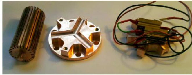
FIGURE 3.5: Photo of the cold finger, which sits in the inner cryostat. Left to right: slitted cold finger, cold finger top flange, top cap of the flange.
