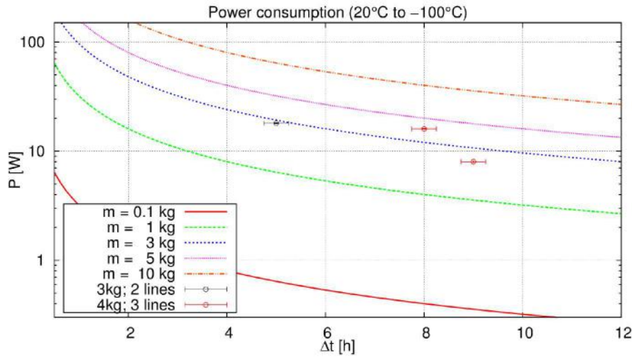
FIGURE 3.9: Theoretically necessary cooling power to cool various masses of pure LXe down to -100^\circ\text{C} as function of cool down time. The power necessary for the phase transition from gas to liquid was taken into account. Three measured cool downs are shown: 1st) for a run with reduced cooling power and 3 kg LXe (2 cold lines only) in black, 2nd) source run in April 2017 with 4 kg LXe and 3rd) from the low gain run cool down with 4 kg LXe in red lower point. The measurements match the expectations from the design.
