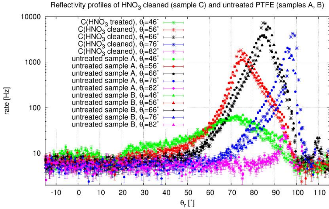
FIGURE 2.20: Raw reflection profiles of the 3 sampled systematic measurement. The untreated samples A&B were simply not cleaned with \text{HNO}_3 , ethanol and water according to [23] while sample C was cleaned so.
