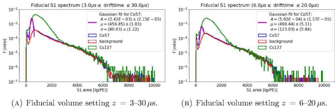
FIGURE 3.55: S1 area and Co57 122keV line fit for two example fiducial volume settings. The full absorption peak shrinks with decreasing fiducial volume. Table 3.7 summarizes the result for all tested fiducial volumes.
