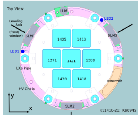
FIGURE 3.25: Sketch of the top view on the TPC with the top PMT array.
