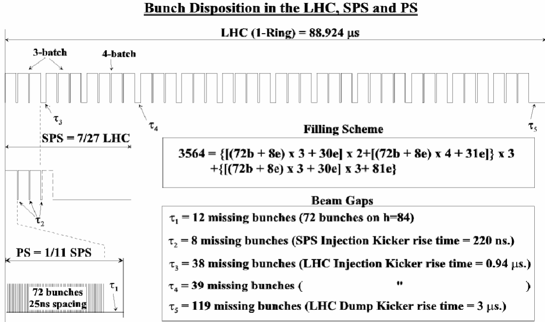
Figure 1.3: Reference filling pattern of the LHC.
