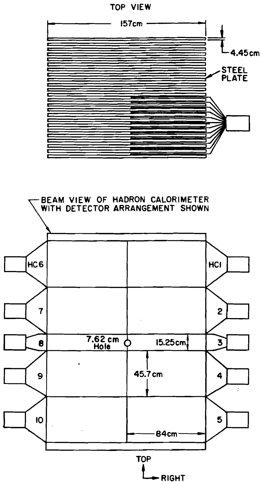
Figure II.12: Hadron Calorimeter
