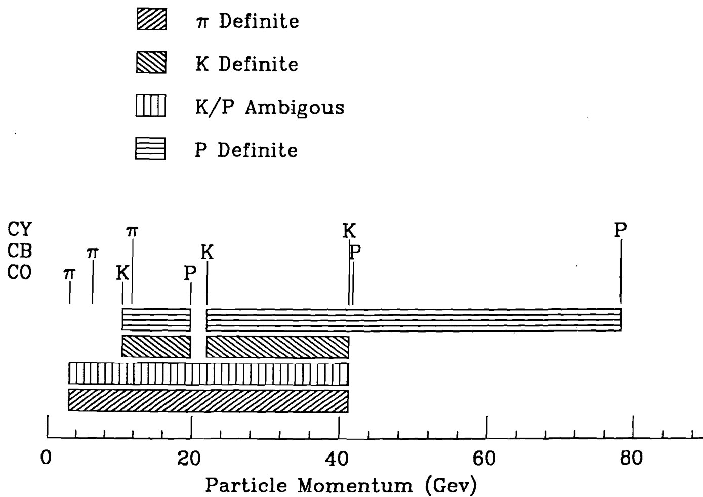
Figure III.1: Čerenkov Identification Ranges, LOGIC The shaded areas show the momentum ranges where \pi_{def} , K_{def} , K/P_{amb} , and P_{def} identifications are possible using the algorithm, LOGIC.
