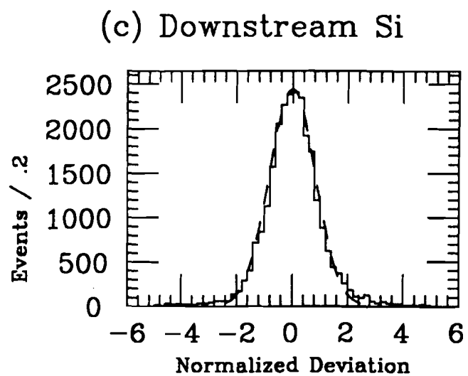
Figure D.1: The observed error in Z_\nu is compared to a unit Gaussian, (a) and (b), and .82 times a unit Gaussian, (c) and (d).
