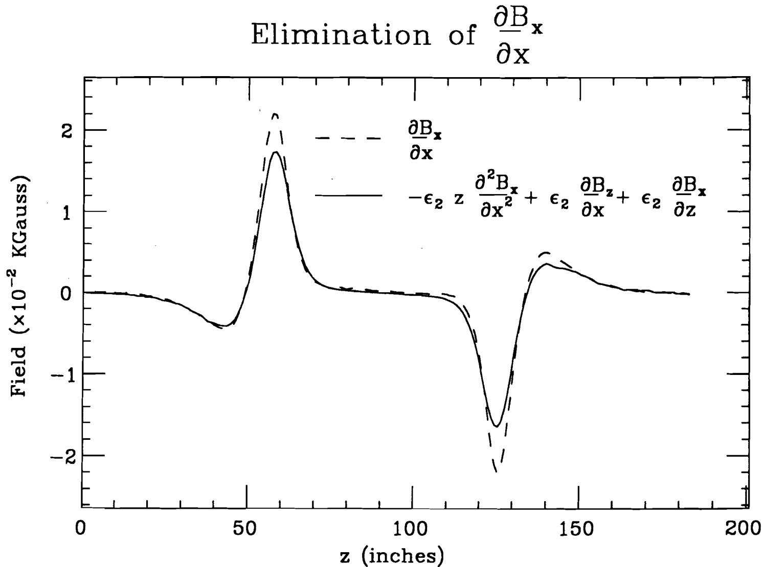
Figure A.8: Elimination of \frac{\partial B_x}{\partial x}
