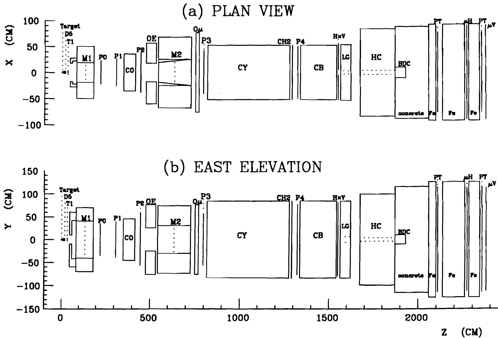
Figure II.2: E400 Spectrometer
