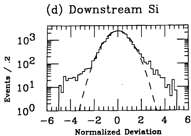
Figure D.1: The observed error in Z_\nu is compared to a unit Gaussian, (a) and (b), and .82 times a unit Gaussian, (c) and (d).
