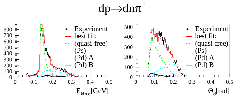
Fig. 3. Deuteron energy and angular distributions for dp \rightarrow dn\pi^+ at T_d = 558 MeV corresponding to \eta = 0.85
