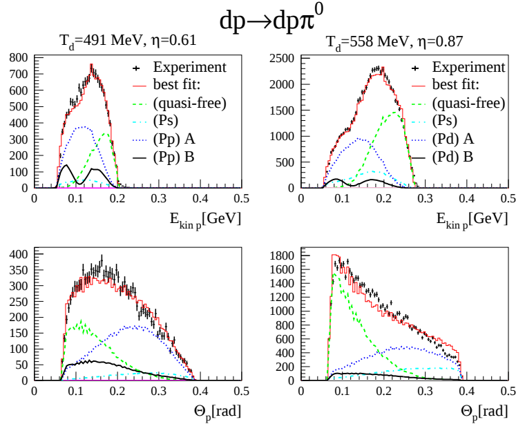
Fig. 2. Proton energy and angular distributions in comparison with different model calculations. The left column shows distributions for dp \rightarrow dp\pi^0 at T_d = 491 MeV and the right column at T_d = 558 MeV. The separate contributions to the best fit are also shown.
