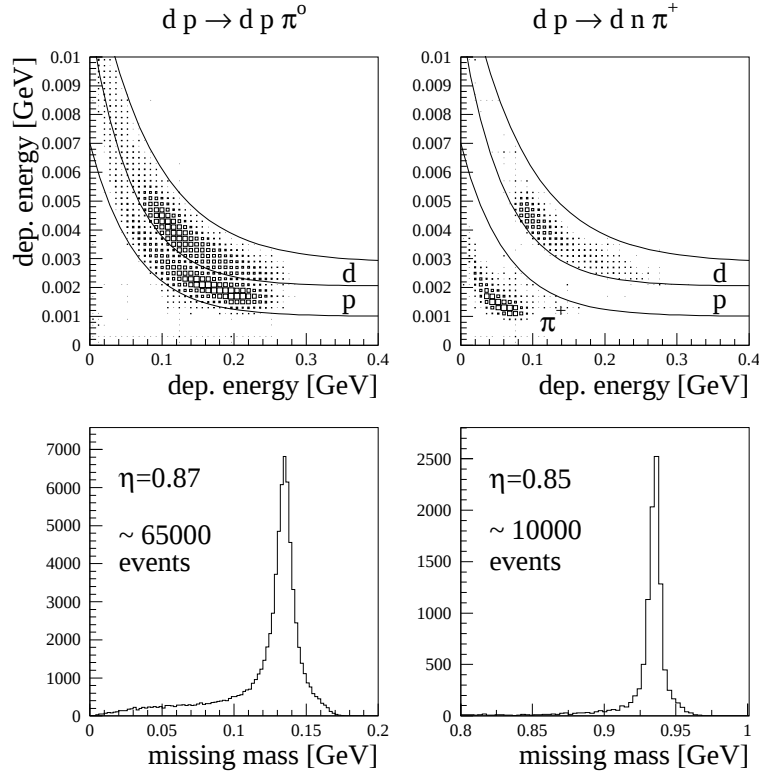
Fig.1. \Delta E versus E plots and missing-mass distributions for selected events at T_d = 558 MeV.
