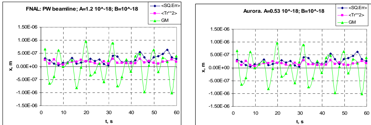
Figure 3. Beam steering with GM for FNAL sites: PW beamline and Aurora (100 m underground mine).
