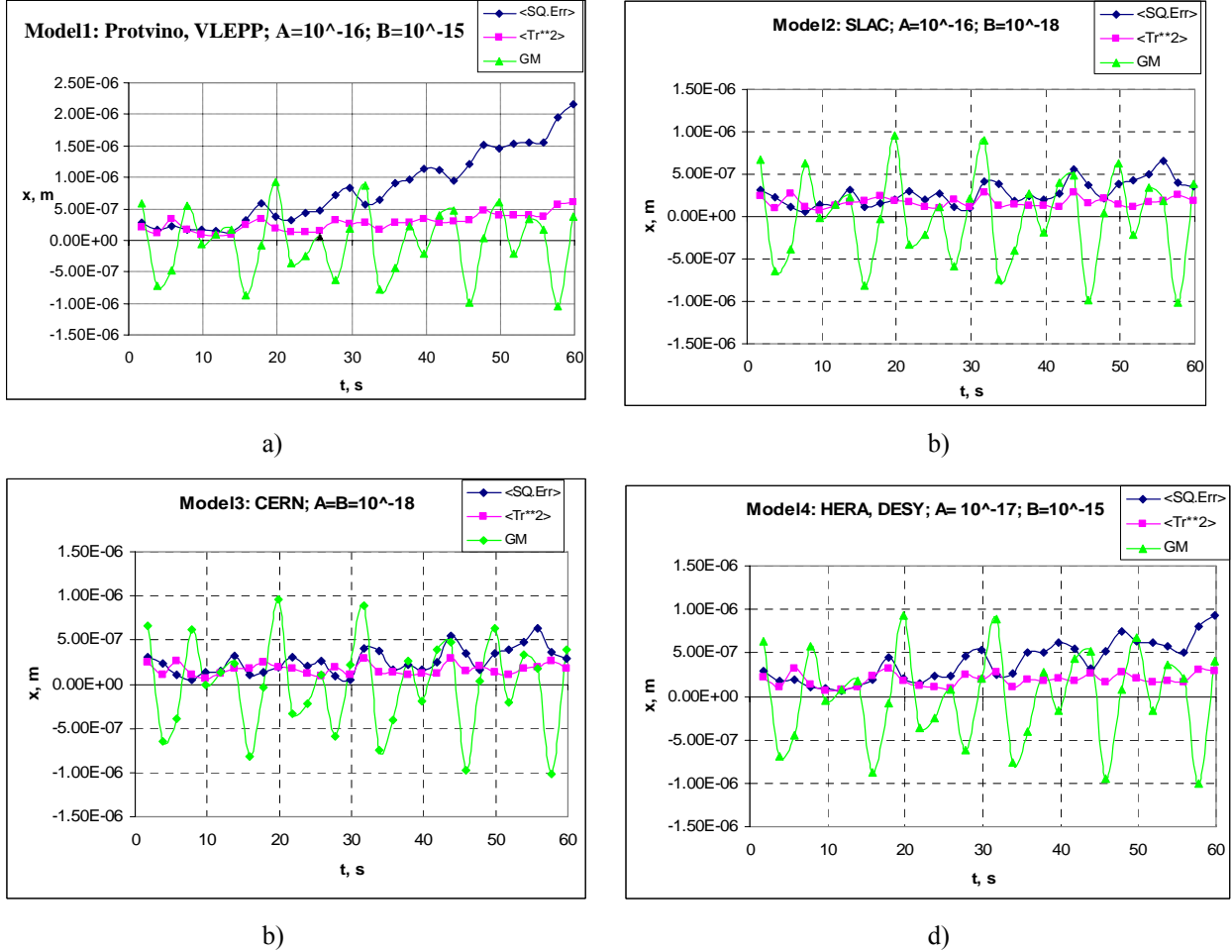
Figure 1. Beam steering with GM for different sites: a) Protvino; b) SLAC; c) CERN d) DESY. Green lines represent the GM at some particular point of the structure; blue lines correspond to the averaged misalignment over all elements; red lines show beam steering - averaged trajectory offset.
