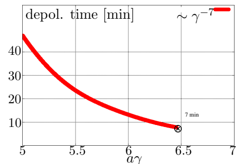
(b) Simulated depolarising time versus a\gamma where a = 0.00115965 is the gyromagnetic anomaly of the electron and \gamma is the Lorentz factor.
