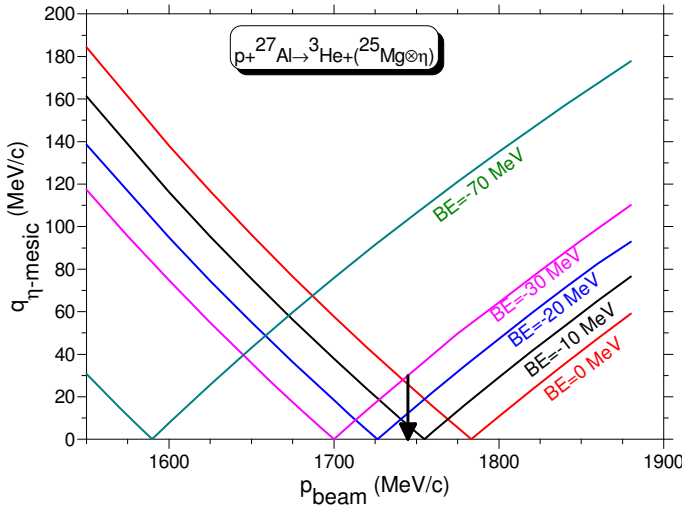
Fig. 8. Momentum transfer to the \eta mesic system as function of the beam momentum for the deuteron transfer reaction. The curves show the relation for different binding energies. The arrow shows the presently used beam momentum.
