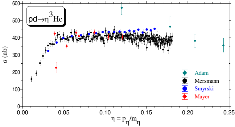
Fig. 1. Excitation function for the reaction pd \rightarrow \eta^3\text{He} in the threshold region as function of the dimensionless \eta momentum \eta = p_\eta/m_\eta .
