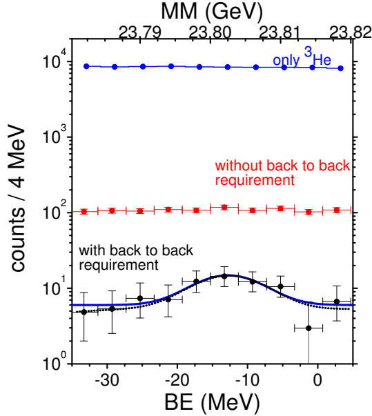
Fig. 11. Missing-mass spectra as measured with the magnetic spectrograph. The upper abscissa is the missing mass, while the lower is the binding energy of a bound system ^{25}\text{Mg} \otimes \eta (see the text).
