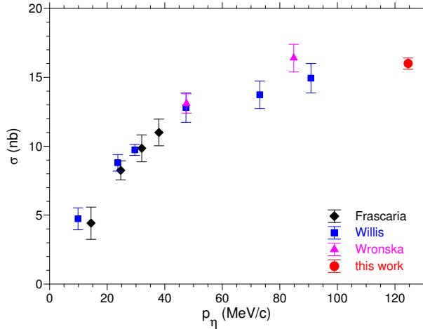
Fig. 3. Excitation function for the total cross section for the dd \rightarrow \alpha \eta reaction. Only statistical errors are shown.
