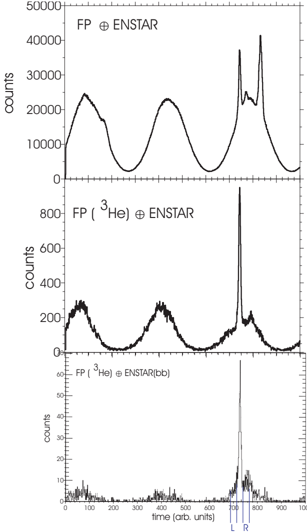
Fig. 9. The measured time-of-flight (TOF) in the focal plane of Big Karl under different boundary conditions indicated next to the appropriate spectrum.
