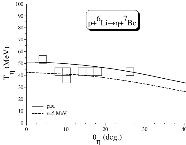
Fig. 4. The events for the indicated reaction obtained at SATURNE [27]. The solid curve is the kinematical curve for the {}^7\text{Be} ground state, while the dashed curve is the one for an excitation of 5 MeV.
