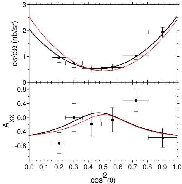
Fig. 2. Upper panel: Differential cross section for the dd \rightarrow \alpha\eta reaction. Lower panel: Analyzing power A_{xx} . The solid curves represent a fit with four partial waves; the dotted curves with invariant amplitudes.
