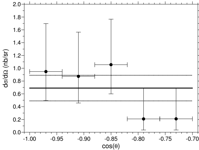
Fig. 5. Angular distribution of reconstructed \eta mesons [28].
