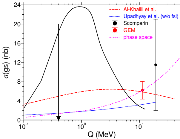
Fig. 6. Excitation function for the p^6\text{Li} \rightarrow \eta^7\text{Be}(\text{g.s.}) reaction. The two data points are from Refs. [27] and [28]. The dashed curve is the Al-Khalili et al. model, the dash-dotted phase space behavior, both normalized to the GEM data point. The solid and the dotted curves are calculations [30] with and without final state interactions. The arrow indicated the region where only the ground state is involved in the reaction.
