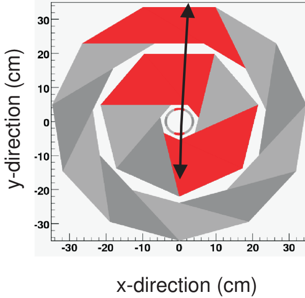
Fig. 10. Cross section of the ENSTAR detector. The arrow up indicated a pion punching through all three layers of the detector, while the arrow down indicates the associated proton being stopped in the middle layer.
