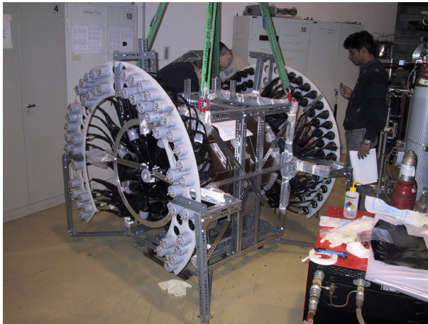
Fig. 7. The ENSTAR detector during assembling.
