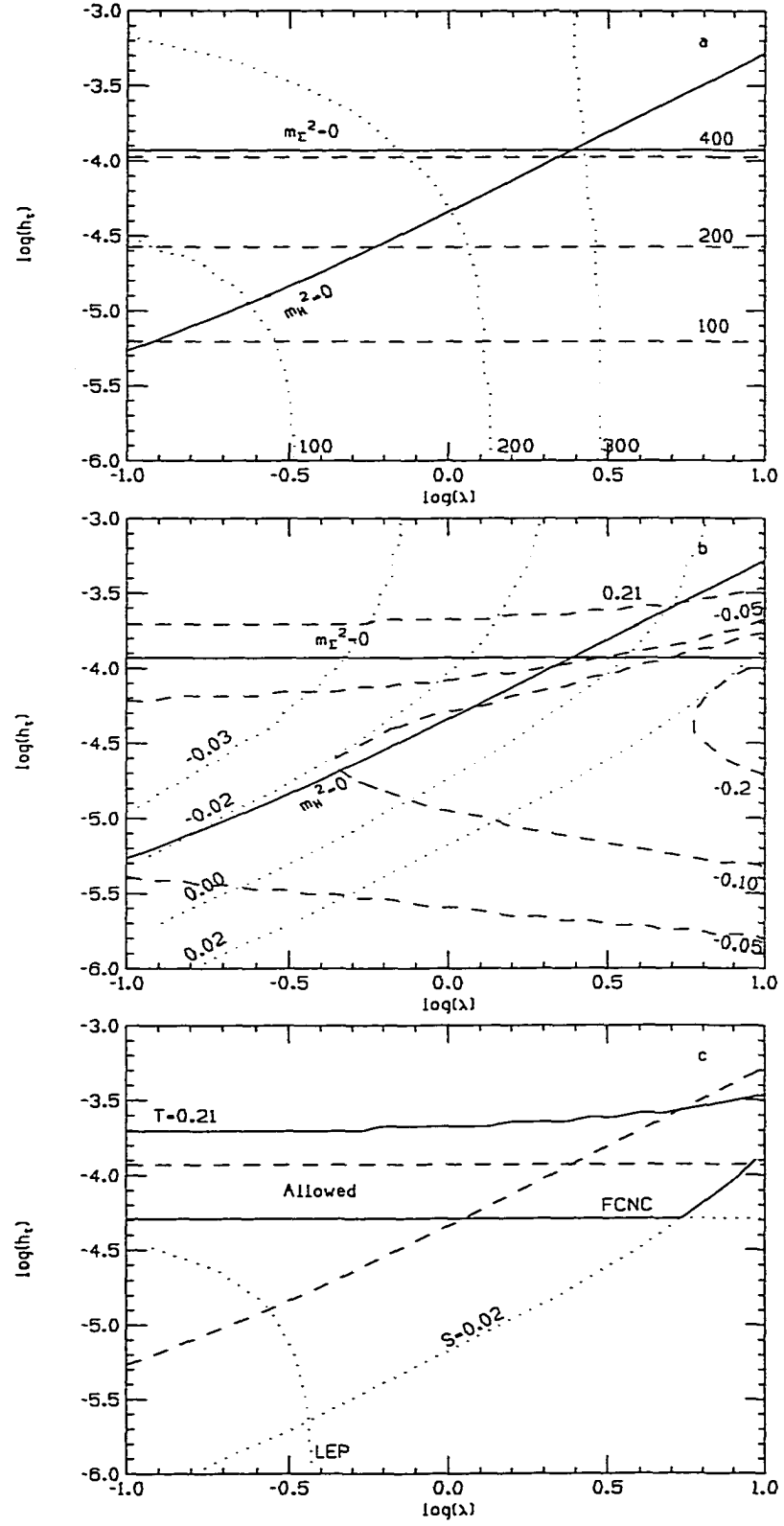
Figure 3.2 Same as Fig. 3.1, with \Lambda = 100 TeV.
