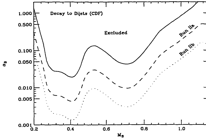
Figure 5.1 Bound on \alpha_B from the cross section times branching fraction to dijets. The solid line corresponds to the bound obtained from Run I with a Luminosity of 106 \text{ pb}^{-1} . The dashed line corresponds to a luminosity of 2 \text{ fb}^{-1} for Run IIa and the dotted line to a luminosity of 20 \text{ fb}^{-1} for Run IIb.
