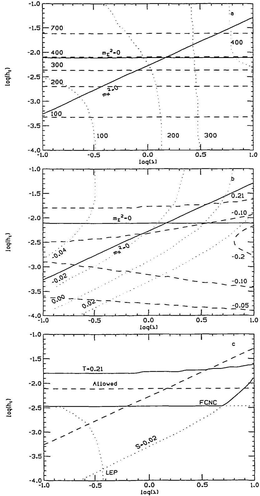
Figure 3.1 Minimal model, \Lambda = 10 TeV. (a) Neutral (dashed) and charged (dotted) mass contours, units of GeV, (b) S (dotted) and T (dashed) parameter contours, (c) Exclusion regions.
