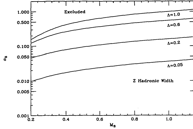
Figure 5.4 Bound obtained from the contribution of the first 1000 KK modes to the Z hadronic width.
