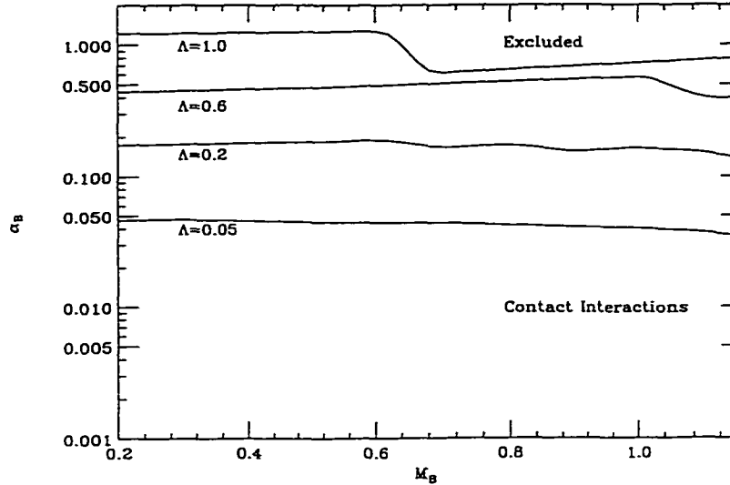
Figure 5.3 Bounds obtained from the contribution of KK modes heavier than 1.15 TeV to contact interactions for several values of \Lambda .
