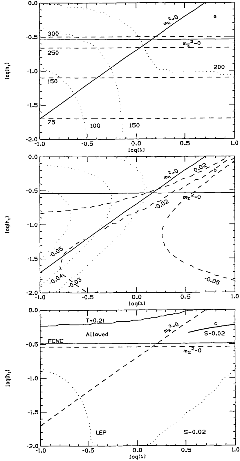
Figure 3.3 General model, m_{H\Sigma}^2 = (400 \text{ GeV})^2 , \lambda_0 = 1 . Notation is the same as in Figs. 3.1 and 3.2.
