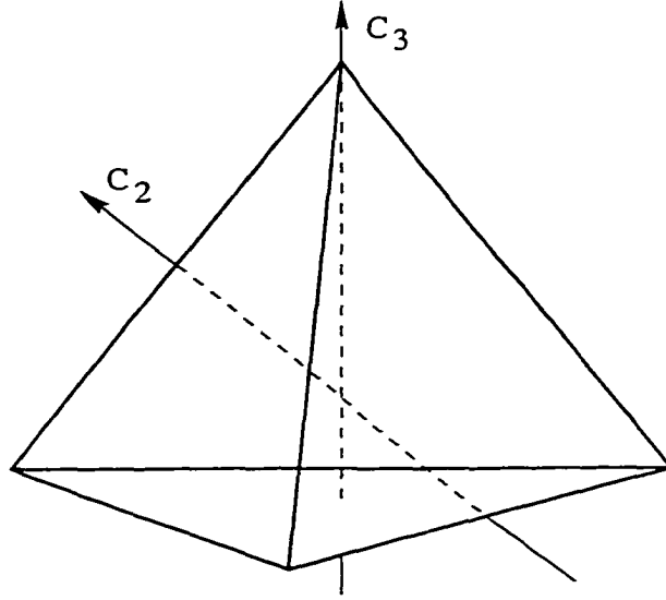
Figure 2.1 Geometrical illustration of the group T' or T . The rotations C_2 and C_3 generate all other rotations in each group.
