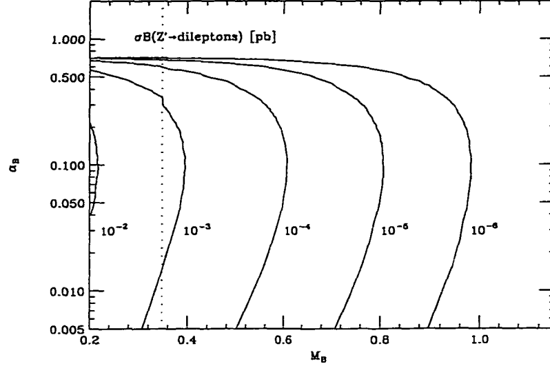
Figure 5.2 Contours of constant cross section times branching fraction to dileptons. The dotted line shows the threshold M_B = 2m_{top} .
