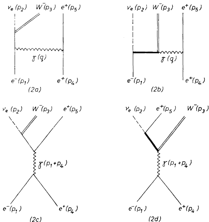
Fig. 2. Feynman diagrams contributing to the process (2)
