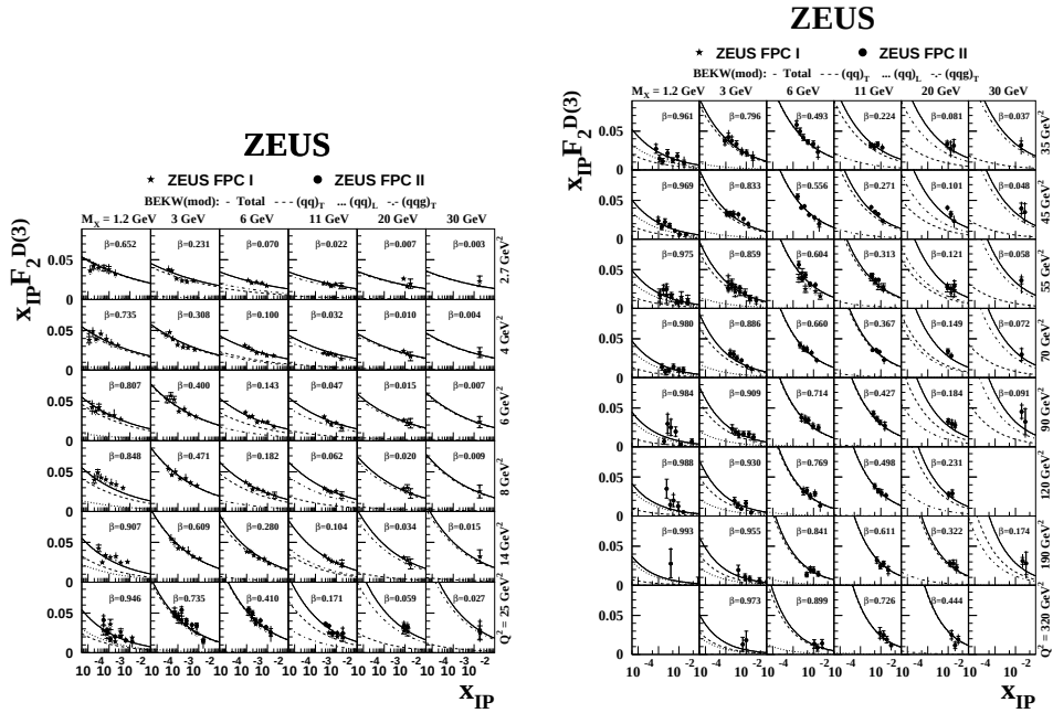
Fig. 30. ZEUS results for x_P F_2^{D(3)} from the \ln M_x^2 -method as a function of x_P at various \beta -values for Q^2 -values from 2.7 \text{GeV}^2 to 25 \text{GeV}^2 (left) and from 35 \text{GeV}^2 to 320 \text{GeV}^2 (right). The lines are the result of a BEKW fit (see text). The solid line is the sum of all contributions, the dashed line is the transverse q\bar{q} contribution, the dotted line is the longitudinal q\bar{q} contribution, and the dashed-dotted line is the q\bar{q}g contribution.
