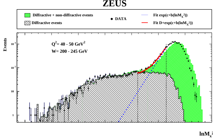
Fig. 23. A measured \ln M_x^2 distribution. Also shown are MC simulations of non-diffractive events (cross hatched) and of diffractive events (hatched). The analytic form of the distribution is fitted to the data between the two vertical lines and the fitted slope of the non-diffractive part is shown as a dotted line.
