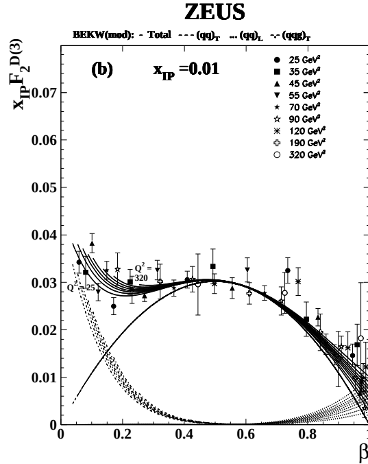
Fig. 31. ZEUS results for x_P F_2^{D(3)} from the \ln M_x^2 -method as a function of \beta at x_P = 0.01 for Q^2 values from 25 \text{GeV}^2 to 320 \text{GeV}^2 . The data are compared to the results of the BEKW(mod) fit showing separately the different fit contributions.
