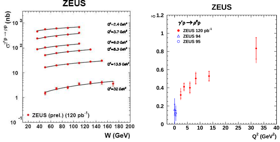
Fig. 12. Left: The W dependence of DIS \rho -production for different values of Q^2 . Right: The slope \delta of the W dependence of DIS \rho -production.
