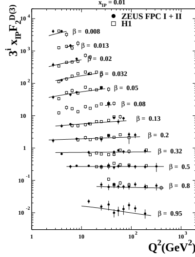
Fig. 32. Comparison of the ZEUS results from the \ln M_x^2 -method with the H1 results from the LRG method. Shown are x_P F_2^{D(3)} values as functions of Q^2 for different \beta values at x_P = 0.01 multiplied by powers of 3 for better visibility. The curves show the results of the BEKW(mod) fit to the ZEUS data.
