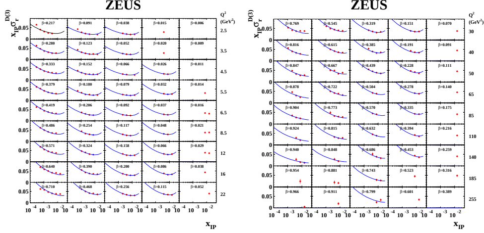
Fig. 28. Result for inclusive diffraction from ZEUS from the LRG method as a function of x_{1P} for various \beta -values and for Q^2 values from 2.5 GeV 2 to 255 GeV 2 . The lines are the result of a Regge fit.
