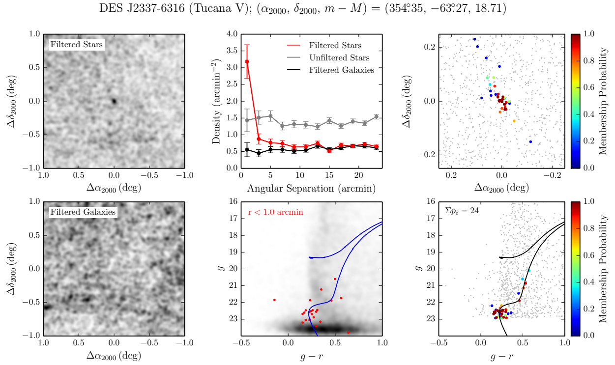
Fig. 12.— Analogous to Figure 6 but for DES J2337–6316 (Tucana V).
