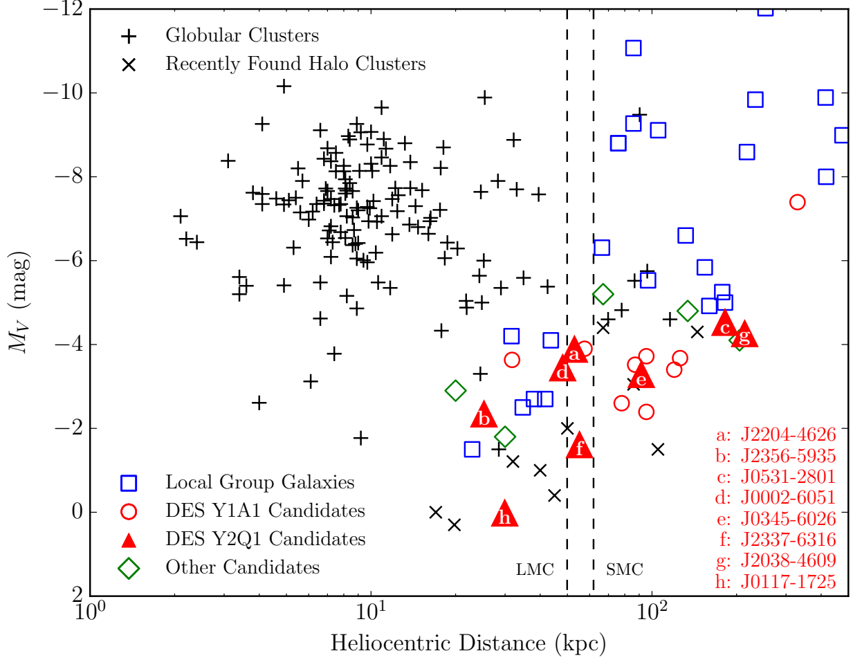
Fig. 5.— DES satellite galaxy candidates (red circles and triangles) have comparable luminosities to known Local Group galaxies (blue squares; McConnachie 2012) and other newly discovered galaxy candidates (green diamonds), but are typically found at larger distances. Dashed lines indicate the heliocentric distances of the LMC and SMC. Globular clusters (black “+” symbols, Harris 1996) and outer halo star clusters (“x” symbols) have been detected at comparable luminosities and distances due to their more compact nature. The constituents of each source class can be found in Figure 4.
