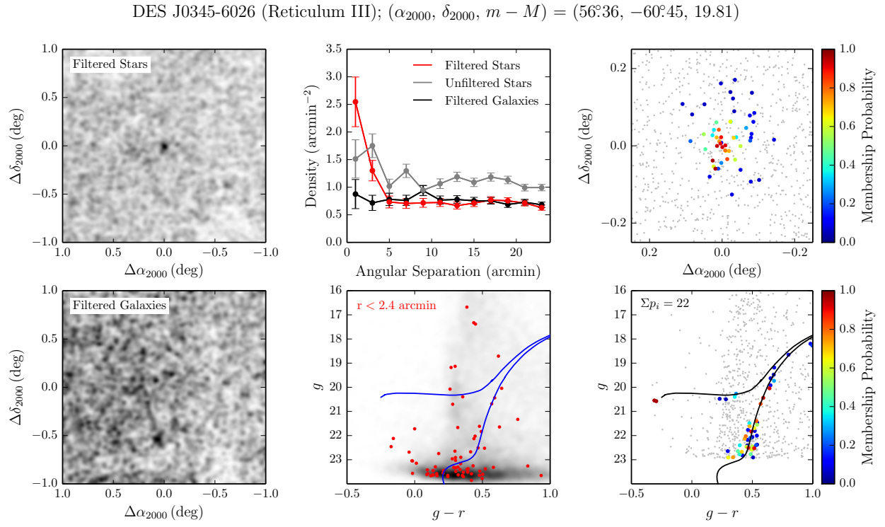
Fig. 11.— Analogous to Figure 6 but for DES J0345–6026 (Reticulum III).
