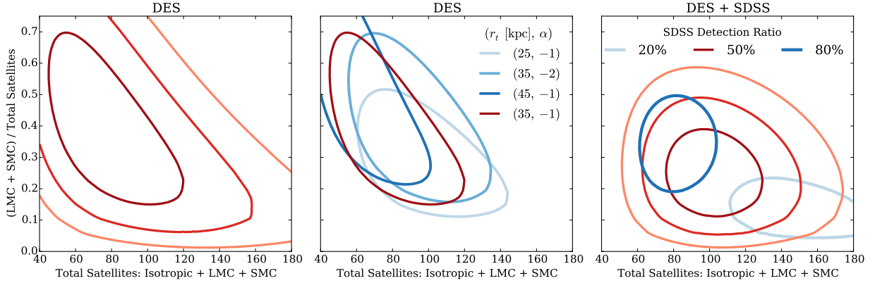
Fig. 16.— Maximum-likelihood fit to the spatial distribution of satellites for a model including isotropic, LMC, and SMC components (Section 6.3). The horizontal axis represents the total number of satellites detectable at DES Y2Q1 depth integrated over the entire sky (not including the classical dwarf galaxies and detection inefficiency near the Galactic plane). The vertical axis represents the fraction of these satellites associated with the Magellanic Clouds. Left : The 1\sigma , 2\sigma , and 3\sigma likelihood contours when considering only DES data. Center : 1\sigma contours for different values of the LMC and SMC truncation radius ( r_t ) and the slope of the radial profile ( \alpha ). Right : Contours of the likelihood function when SDSS observations are included. Red contours ( 1\sigma , 2\sigma , 3\sigma ) assume that 50% of the satellites discovered in DES would have been detected if they were located in the SDSS footprint. This value matches the estimated detection efficiency from Table 4. We show the sensitivity of our results to the SDSS/DES detection ratio with the dark blue contour (80% detection ratio) and the light blue contour (20% detection ratio).
