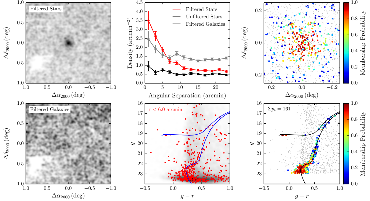
Fig. 6.— Stellar density and color-magnitude diagrams for DES J2204–4626 (Grus II). Top left: Spatial distribution of stellar objects with g < 24 mag that pass the isochrone filter (see text). The field of view is 2^{\circ} \times 2^{\circ} centered on the candidate and the stellar distribution has been smoothed by a Gaussian kernel with standard deviation 1''.2 . Top center: Radial distribution of objects with g - r < 1 mag and g < 24 mag: stars passing the isochrone filter (red), stars excluded from the isochrone filter (gray), and galaxies passing the isochrone filter (black). Top right: Spatial distribution of stars with high membership probabilities within a 0.5^{\circ} \times 0.5^{\circ} field of view. Small gray points indicate stars with membership probability less than 5%. Bottom left: Same as top left panel, but for probable galaxies that pass the isochrone filter. Bottom center: The color-magnitude distribution of stars within 0.1^{\circ} of the centroid are indicated with individual points. The density of the field within an annulus from radii of 0.5^{\circ} to 1.0^{\circ} is represented by the background two-dimensional histogram in grayscale. The blue curve shows the best-fit isochrone as described in Table 1 and Table 2. Bottom right: Color-magnitude distribution of high membership probability stars.
