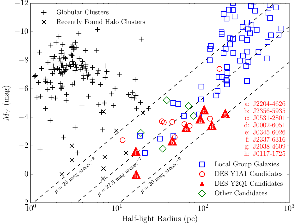
Fig. 4.— Local Group galaxies (McConnachie 2012) and globular clusters (Harris 1996, 2010 edition) occupy distinct regions in the plane of physical half-light radius (azimuthally averaged) and absolute magnitude. The majority of DES satellite candidates (red triangles and circles) are more consistent with the locus of Local Group galaxies (blue squares) than with the population of Galactic globular clusters (black “+”). Other recently reported dwarf galaxy candidates (green diamonds) include Hydra II (Martin et al. 2015), Triangulum II (Laevens et al. 2015a), Pegasus III (Kim et al. 2015a), Draco II and Sagittarius II (Laevens et al. 2015b). Several outer halo star clusters and systems of ambiguous classification are indicated with “x” symbols: Kposov 1 and Kposov 2 (Kposov et al. 2007; Paust et al. 2014), Segue 3 (Belokurov et al. 2010; Fadelly et al. 2011; Ortolani et al. 2013), Muñoz 1 (Muñoz et al. 2012), Balbinot 1 (Balbinot et al. 2013), Laevens 1 (Laevens et al. 2014; Belokurov et al. 2014), Laevens 3 (Laevens et al. 2015b), Kim 1 and Kim 2 (Kim & Jerjen 2015a; Kim et al. 2015b), and DES 1 (Luque et al. 2015). Dashed lines indicate contours of constant surface brightness at \mu = \{25, 27.5, 30\} \text{ mag arcsec}^{-2} .
