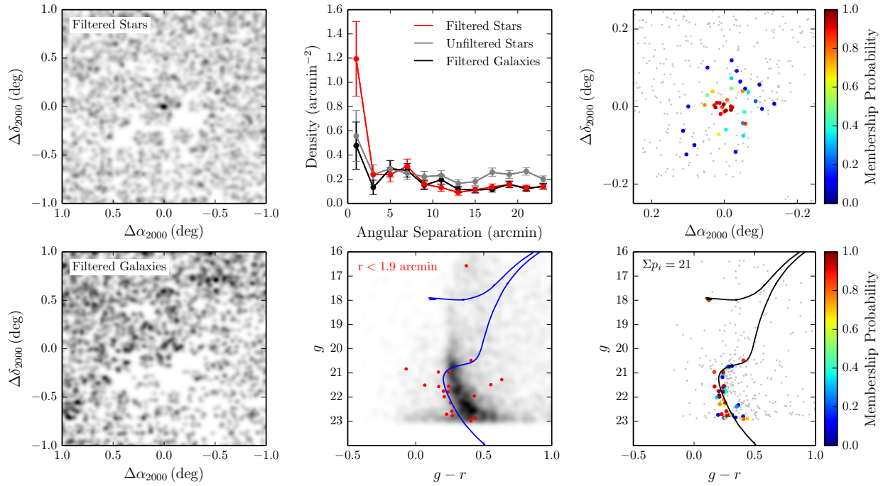
Fig. 14.— Analogous to Figure 6 but for DES J0117–1725 (Cetus II). Note that the magnitude threshold for the smoothed counts maps and radial profiles has been raised to g < 23 mag due to incomplete coverage in this region.
