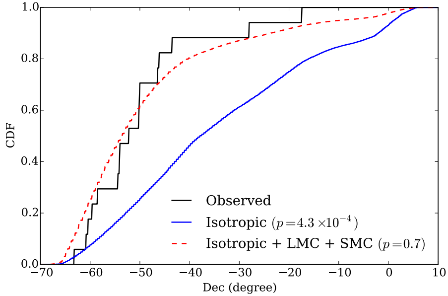
Fig. 15.— The cumulative distribution functions of declination values for the seventeen observed satellites in the DES footprint (black), a uniform distribution given the shape of DES footprint (blue), and the best-fit model for a uniform distribution and Magellanic Cloud components (red dashed). See Section 6.3.
