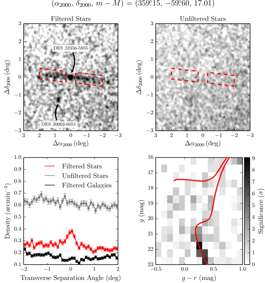
Fig. 8.— Possible tidal tails around DES J2356–5935 (Tucana III). Top left : Spatial distribution of stellar objects with g < 23 mag that pass the same isochrone filter as applied to visualize DES J2356–5935 (Figure 7). Red boxes highlight the positions of the tidal tails. Top right : Spatial distribution of stellar objects with g - r < 1 mag and g < 23 mag not passing the isochrone filter. Bottom left : Average density profiles transverse to the tidal tail axis: stars passing the isochrone filter (red), other unfiltered stars (gray), and galaxies passing the isochrone filter (black). For the density calculation, the range of included angles parallel to the tidal tails is \pm 2^{\circ}.0 , excluding the region within 0^{\circ}.3 of DES J2356–5935. Bottom right : Binned significance diagram representing the Poisson probability of detecting the observed number of stars within 0^{\circ}.2 of the tidal tail axis (excluding the region within 0^{\circ}.3 of DES J2356–5935) for each bin of the color-magnitude space given the local field density.
