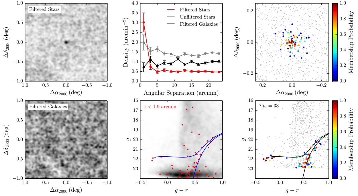
Fig. 9.— Analogous to Figure 6 but for DES J0531–2801 (Columba I).
