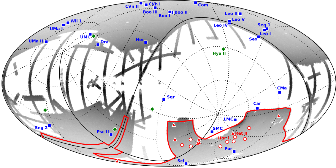
Fig. 1.— Locations of the eight new dwarf galaxy candidates reported here (red triangles) along with nine previously reported dwarf galaxy candidates in the DES footprint (red circles; Bechtol et al. 2015; Koposov et al. 2015a; Kim & Jerjen 2015b), five recently discovered dwarf galaxy candidates located outside the DES footprint (green diamonds; Laevens et al. 2015a; Martin et al. 2015; Kim et al. 2015a; Laevens et al. 2015b), and twenty-seven Milky Way satellite galaxies known prior to 2015 (blue squares; McConnachie 2012). Systems that have been confirmed as satellite galaxies are individually labeled. The figure is shown in Galactic coordinates (Mollweide projection) with the coordinate grid marking the equatorial coordinate system (solid lines for the equator and zero meridian). The gray scale indicates the logarithmic density of stars with r < 22 from SDSS and DES. The two-year coverage of DES is \sim 5000 \text{ deg}^2 and nearly fills the planned DES footprint (outlined in red). For comparison, the Pan-STARRS 1 3\pi survey covers the region of sky with \delta_{2000} > -30^\circ (Laevens et al. 2015b).
