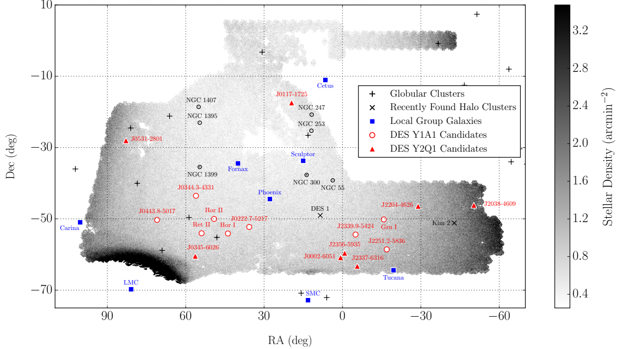
Fig. 3.— Cartesian projection of the density of stars observed in both g - and r -bands with g < 23 and g - r < 1 over the DES Y2Q1 footprint ( \sim 5000 \text{ deg}^2 ). Globular clusters are marked with “+” symbols (Harris 1996, 2010 edition), two faint outer halo clusters are marked with “x” symbols (Kim et al. 2015b; Luque et al. 2015), Local Group galaxies known prior to DES are marked with blue squares (McConnachie 2012), dwarf galaxy candidates discovered in Y1 DES data are marked with red outlined circles, while the Y2 stellar systems are marked with red triangles. The periphery of the LMC can be seen in the southeast corner of the footprint, while the Galactic stellar disk can be seen on the eastern and western edges.
