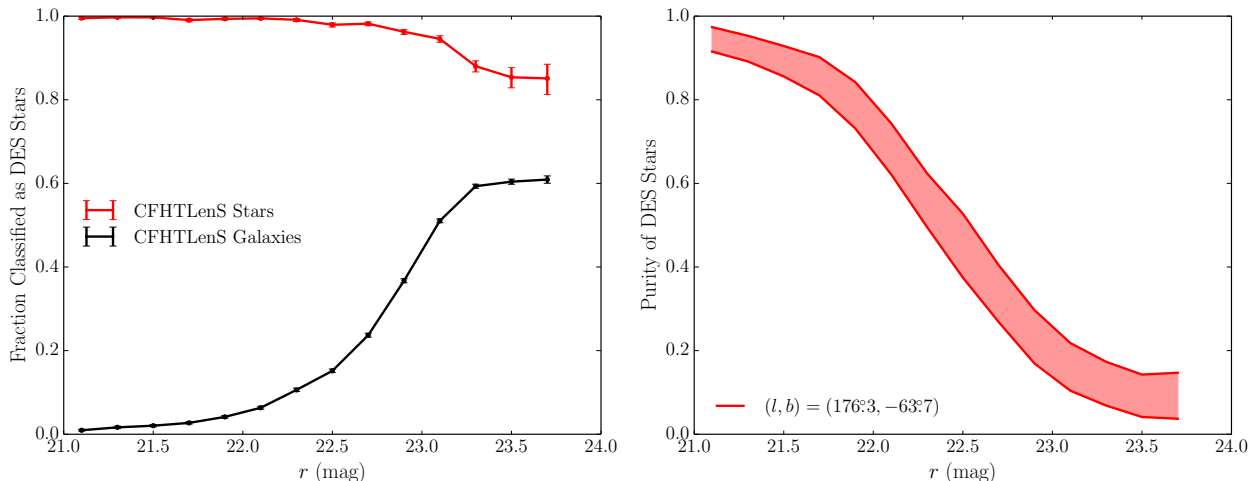
Fig. 2.— Performance of the morphological stellar classification based on |wavg\_spread\_model\_r| < 0.003 + spreaderr\_model\_r was evaluated by comparing against deeper CFHTLenS imaging (Section 2.2). Left : Fraction of CFHTLenS-classified stars and galaxies that pass our DES stellar selection criteria. Right : Stellar purity evaluated in a typical high-Galactic latitude field centered at Galactic coordinates (l, b) = (176^{\circ}3, -63^{\circ}7) . The shaded region represents the uncertainty associated with objects that are not confidently classified as either stars or galaxies with CFHTLenS. If a large fraction of these ambiguous objects are true stars, the inferred stellar purity for DES is near the upper bound of the indicated range.
