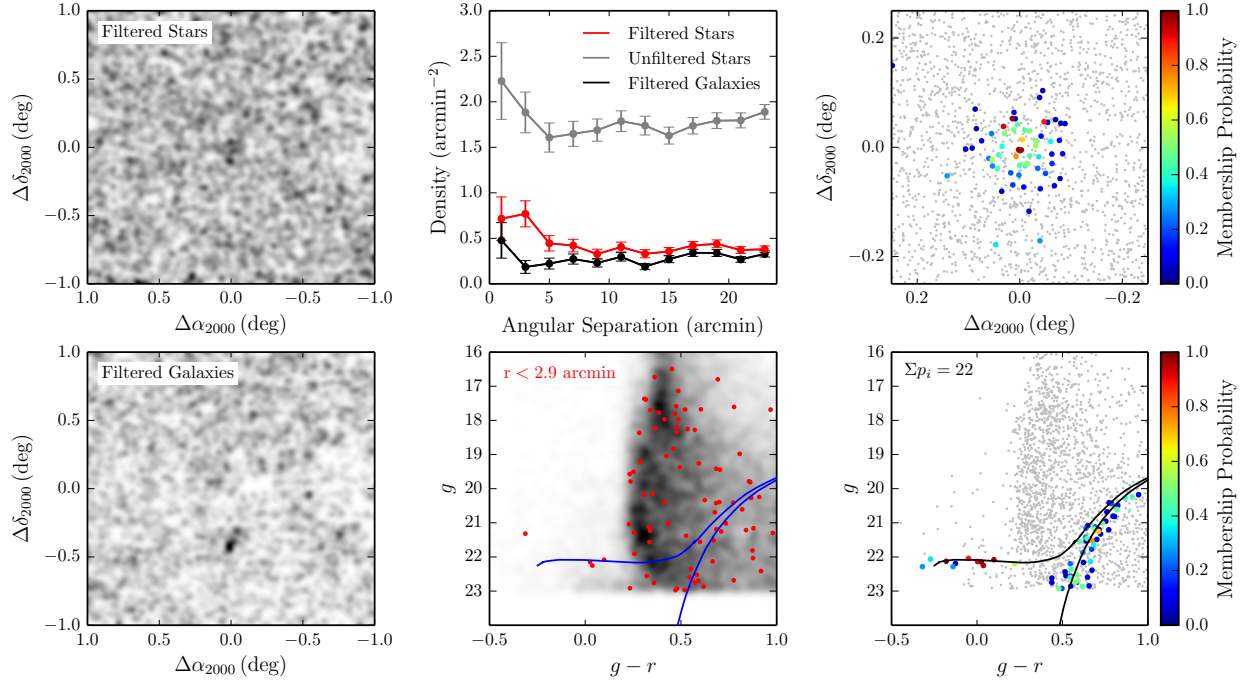
Fig. 13.— Analogous to Figure 6 but for DES J2038–4609 (Indus II). Note that the magnitude threshold for the smoothed counts maps and radial profiles has been raised to g < 23 mag due to non-uniform imaging depth in this region. DES J2038–4609 is detected primarily by a cluster of potential BHB members.
