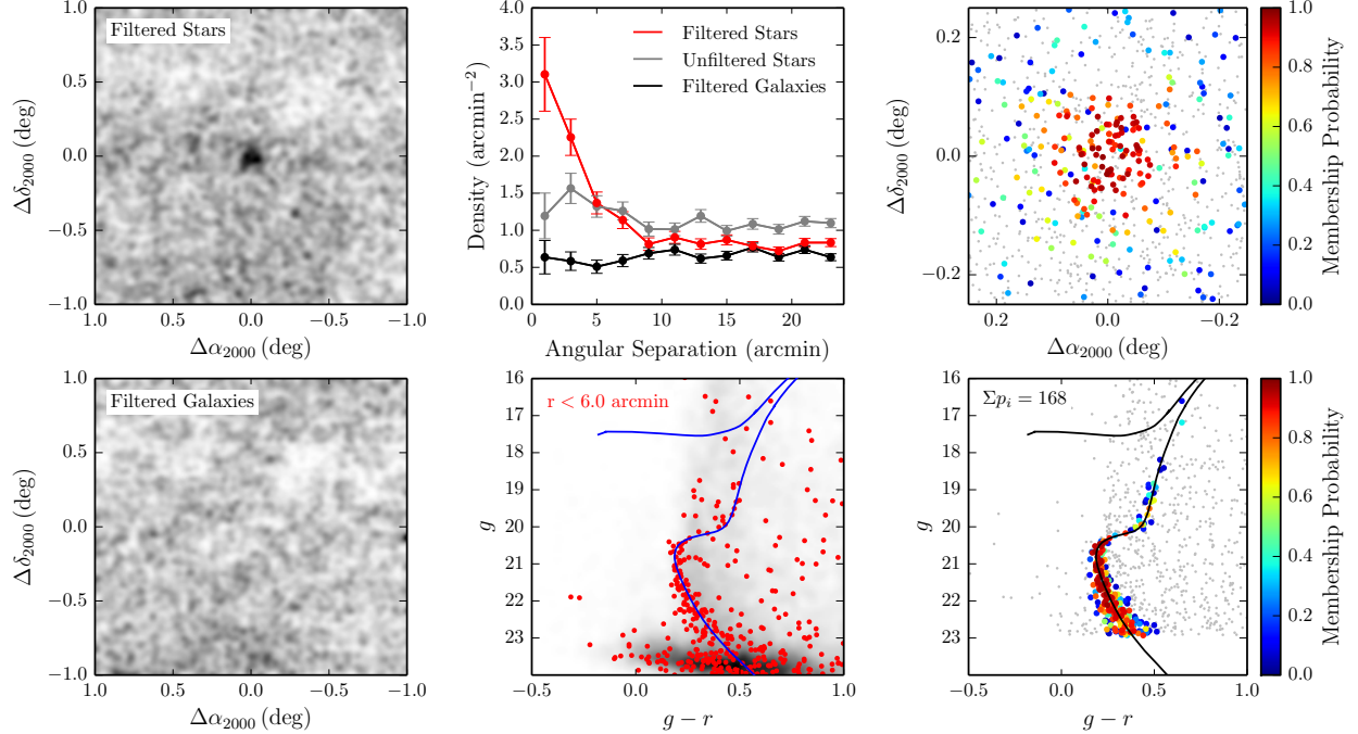
Fig. 7.— Analogous to Figure 6 but for DES J2356–5935 (Tucana III).
