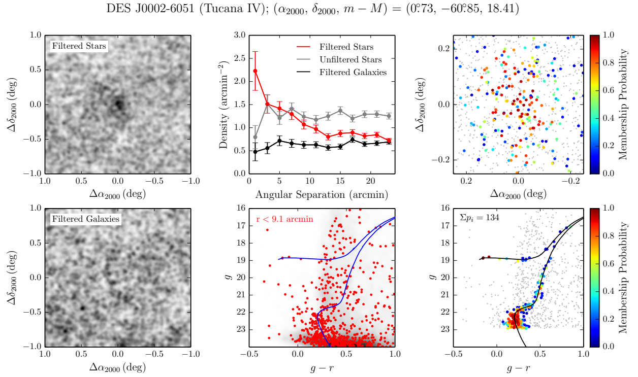
Fig. 10.— Analogous to Figure 6 but for DES J0002–6051 (Tucana IV).
