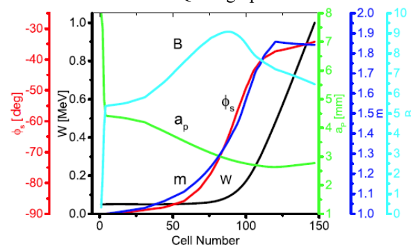
Figure 1: RFQ design parameters after optimization.
