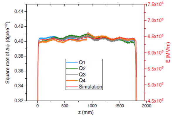
Figure 3: Measured and simulated electric field distributions after tuning.
