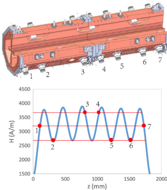
Figure 2: Positions of tuners relative to (top) the coupling windows and (bottom) the magnetic field distribution.
