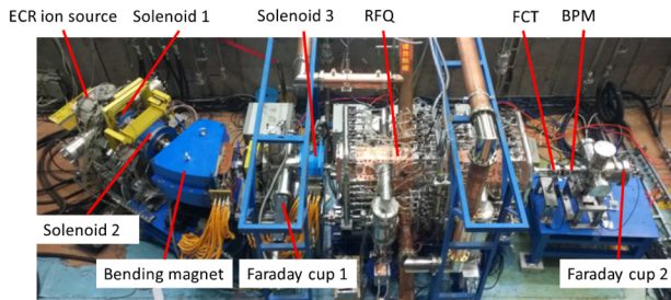
Figure 5: Overview of the RFQ test area.
