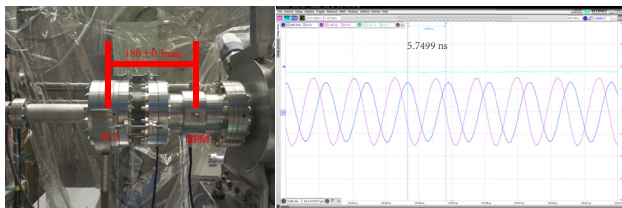
Figure 6: Measured distance and beam signals detected by the FCT and BPM (the FCT signal is blue, the BPM signal is pink).
