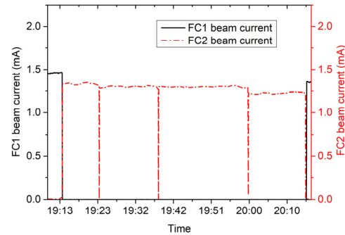
Figure 7: Change of FC1 and FC2 beam current during one hour of CW operation.
