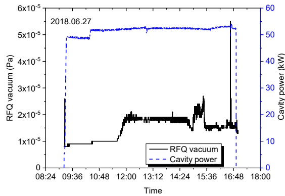
Figure 4: Uninterrupted (no-spark) operations at CW power of 50 kW recorded over 7 hours.
