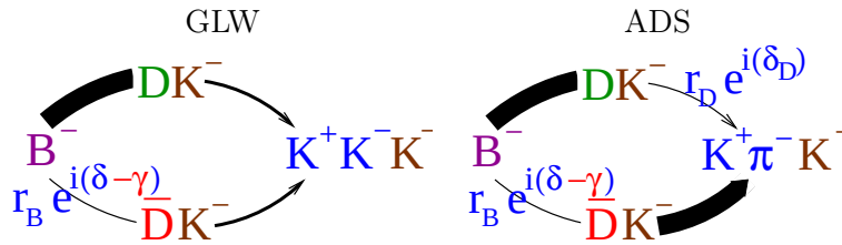
Fig. 1. CKM phases manifest themselves in interfering decay paths to the same final states. The differences of GLW vs ADS are explained in the text.
