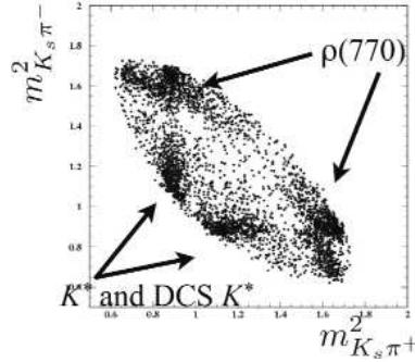
Fig. 2. Dalitz Plot for D \rightarrow K_s \pi^+ \pi^- from generator-level study at LHCb. The most important resonances are pointed out, but more than 15 subresonances contribute to the decay.
