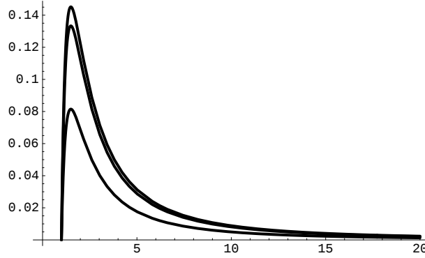
Fig. 4. This graph shows \frac{4M^2}{L^2}V^2 of the massless particle as a function of y = r/(2M) for \varepsilon = 0.1 . Top to bottom the curves are for \varepsilon_0 = 0.02 , \varepsilon_0 = 0.1 , and \varepsilon_0 = 0.45 .
