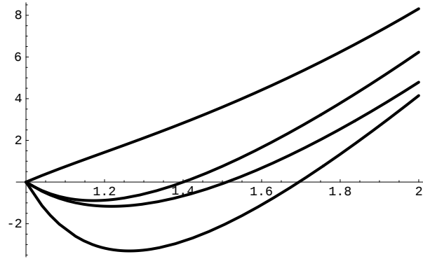
Fig. 1. The effective mass \mu as a function of y = r/2M . Top to bottom the curves are for \xi = 1/3 , \xi = 1/6 (Page approximation), \xi = 1/6 (our approximation), and \xi = 0 . The effective mass for the nonconformal coupling is evaluated within the framework of the Anderson et al. model.
