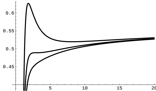
Fig. 5. The effective potential V^2 of a massive particle as a function of r/2M for \varepsilon = 0.1 and \varepsilon_0 = 0.45 . Top to bottom the curves are for l = 3 , l = l_{\text{crit}} = 3.466 , and l = 4.5 . At the point of inflexion the last stable circular orbit occur.
