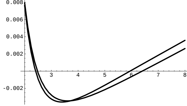
Fig. 7. This graph shows the rescaled fractional trace anomaly of the scalar field in the corrected spacetime as a function of r/M . \pi\Delta/\varepsilon evaluated for the solution of the back reaction equations with the source term given by the improved approximation of the stress energy tensor is the line shifted to the right with respect to the one which has been determined with the aid of the Page approximation
