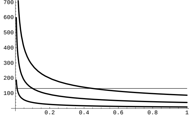
Fig. 2. The maximal radius of the spherical box y_{\max} = R_{\max}/2M as a function of \varepsilon . Top to bottom, the curves are for \varepsilon_0 = 0.45, 0.1, 0.01 . The horizontal line refers to a simplified case of \varepsilon = \varepsilon_0 .
