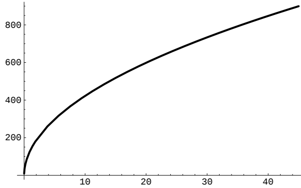
Fig. 3. The maximal radius of the spherical box y_{\max} = R_{\max}/2M as a function of \varepsilon_0/\varepsilon .
