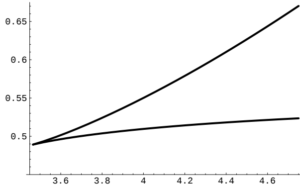
Fig. 6. This graph shows local extrema of the effective potential V^2 as a function of the reduced angular momentum l .
