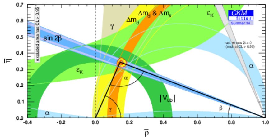
Figure 2.2: Status of measurements of sides and angles of the Unitary Triangle given by Eq. 2.15. Ref. [23].
