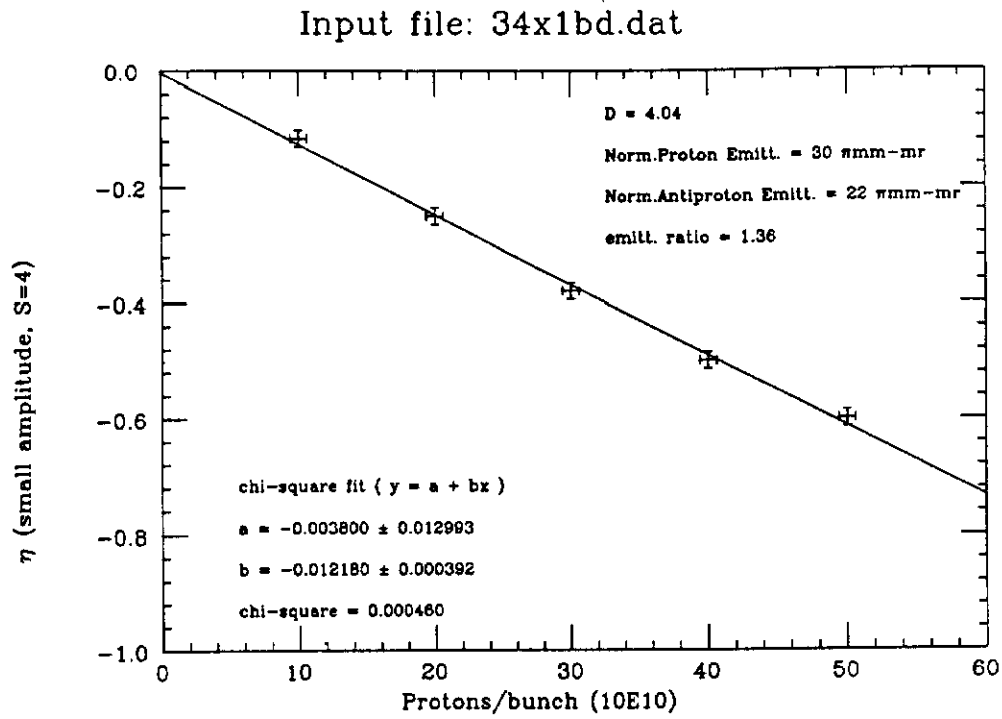
Figure 15: The strength of nonlinearity increases linearly with bunch intensity.
