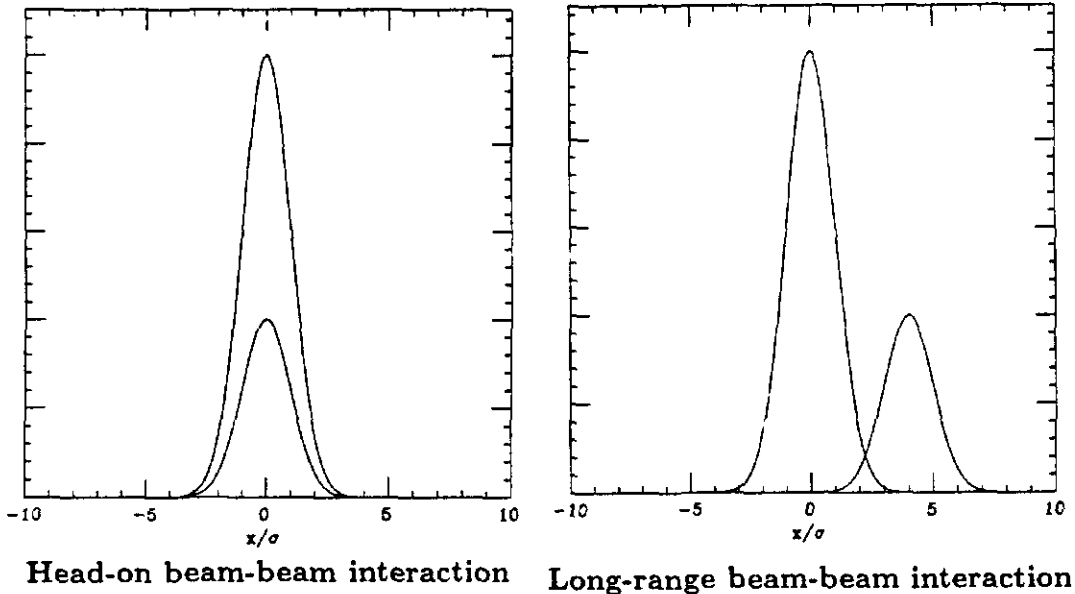
Figure 1: Transverse profiles for source and probe bunches.
