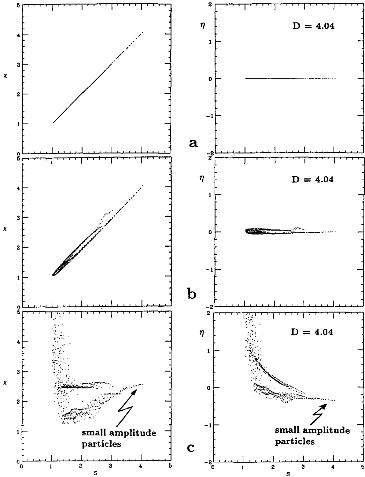
Figure 7: \chi - S diagrams (left) and \eta - S diagrams (right) for the Collider Run with the Main Injector. a) no beam-beam interactions b) only head-on interactions c) 2 head-on, 66 long-range interactions. Note that the nonzero value of |\eta| is caused mostly by long-range interactions. Head-on interactions contribute very little.
