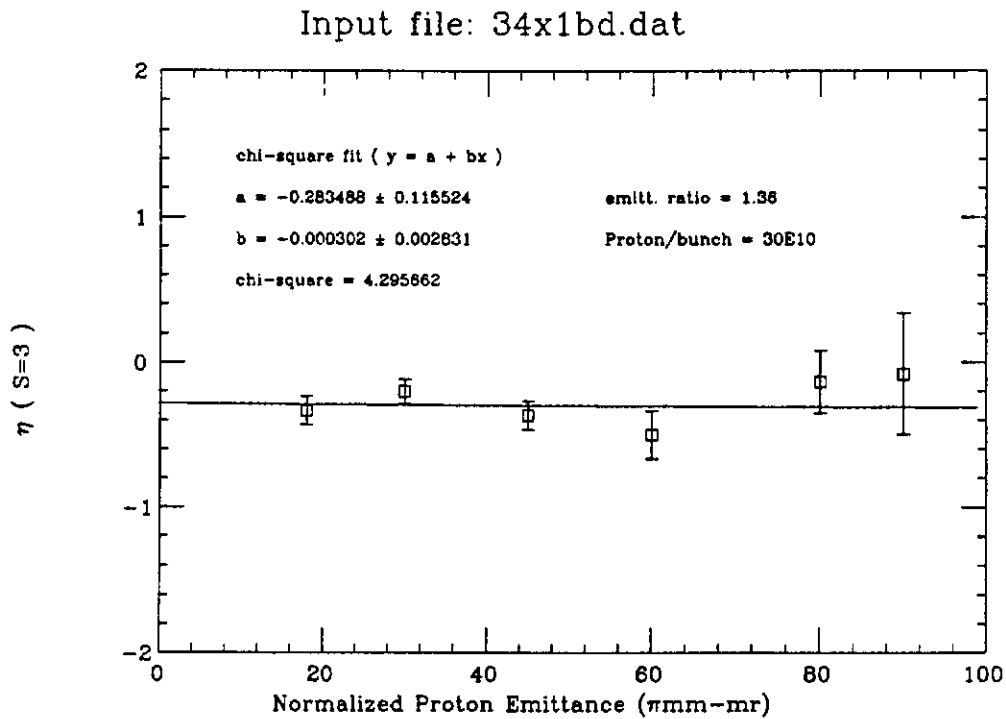
Figure 16: The strength of nonlinearity does not depend on the emittance to first order. The size of error bars, however, increase with emittance, indicating a second or higher order effect.
