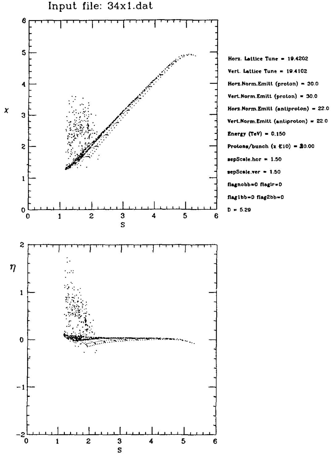
Figure 5: Another demonstration of the nonlinearity in the region 1 < S < 2 . These plots are for the 34x1.dat lattice which has only long-range interactions. Since the number of interactions per turn is larger than that of Fig.(4), the normalized deviation \eta is more pronounced when 1 < S < 2 .
