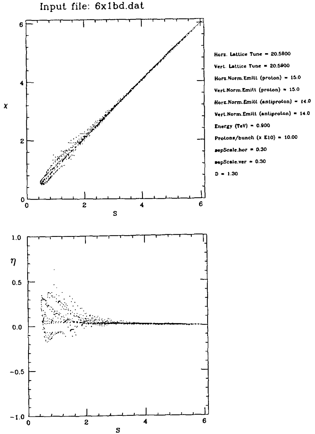
Figure 4: Diagrams showing the effect of nonlinearity for 1 < S < 2 . In a perfectly linear system these plots would be straight lines. Normalized deviation of S from its initial value as the particle circulates around the ring is caused by nonlinearity due to beam-beam interactions. The diagram has been generated from a mesh of amplitudes.
