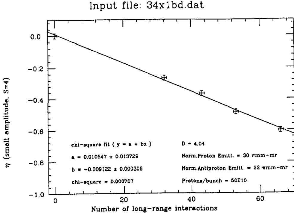
Figure 17: The strength of nonlinearity increases linearly with the number of long-range interactions.
