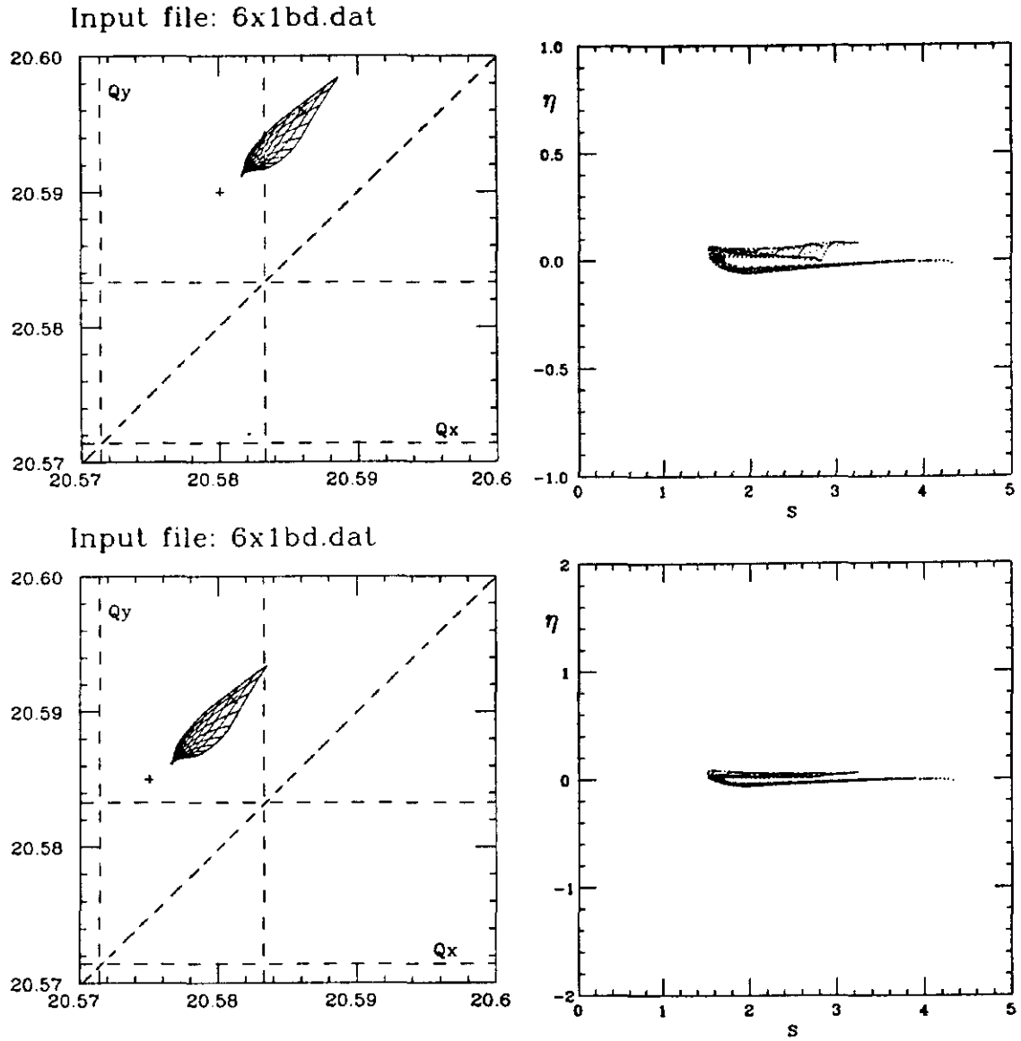
Figure 12: Comparison of working points for the 1992 Collider Run. The working point is indicated by a ' + ' sign on the tuneshift-footprint diagrams. ( \nu_x = 20.5750 , \nu_y = 20.5850 ) is recommended as the optimum working point.
