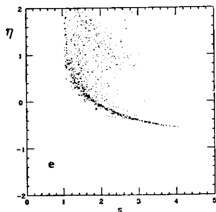
Figure 14: \eta - S Diagrams for the Collider Run with the Main Injector with different bunch intensities. a) N_p = 10 \times 10^{10} b) N_p = 20 \times 10^{10} c) N_p = 30 \times 10^{10} d) N_p = 40 \times 10^{10} e) N_p = 50 \times 10^{10} . The structure in c) is caused by the 5 th order resonance. Note that the absolute value of \eta for small amplitude particles is increasing with N_p
