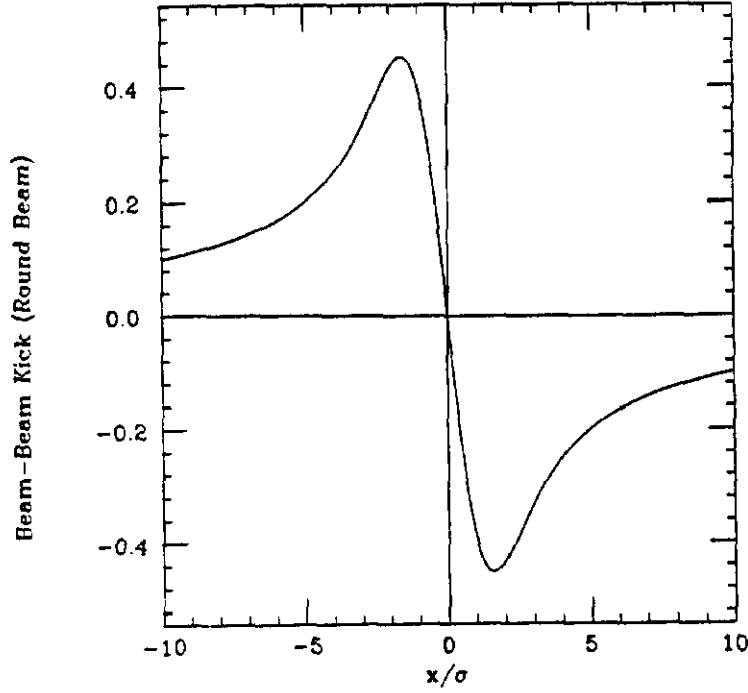
Figure 2: The kick experienced by an oppositely charged probe particle as it passes by a round gaussian source bunch.
