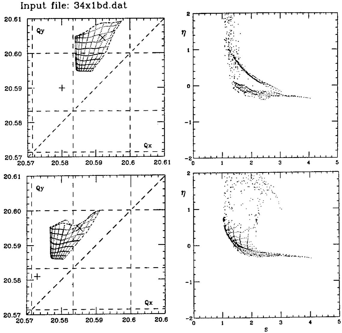
Figure 13: Comparison of working points for the Collider Run with the Main Injector. The working point in the upper diagram is not recommended due to the proximity of the 5 th order resonance. We suggest ( \nu_x = 20.5730 , \nu_y = 20.5810 ) as the optimum working point. In this case, however, the tuneshift-footprint is too close to the coupling resonance. Given the size of the footprint this is unavoidable. Reducing the footprint area by increasing the separator voltages would help the situation.
