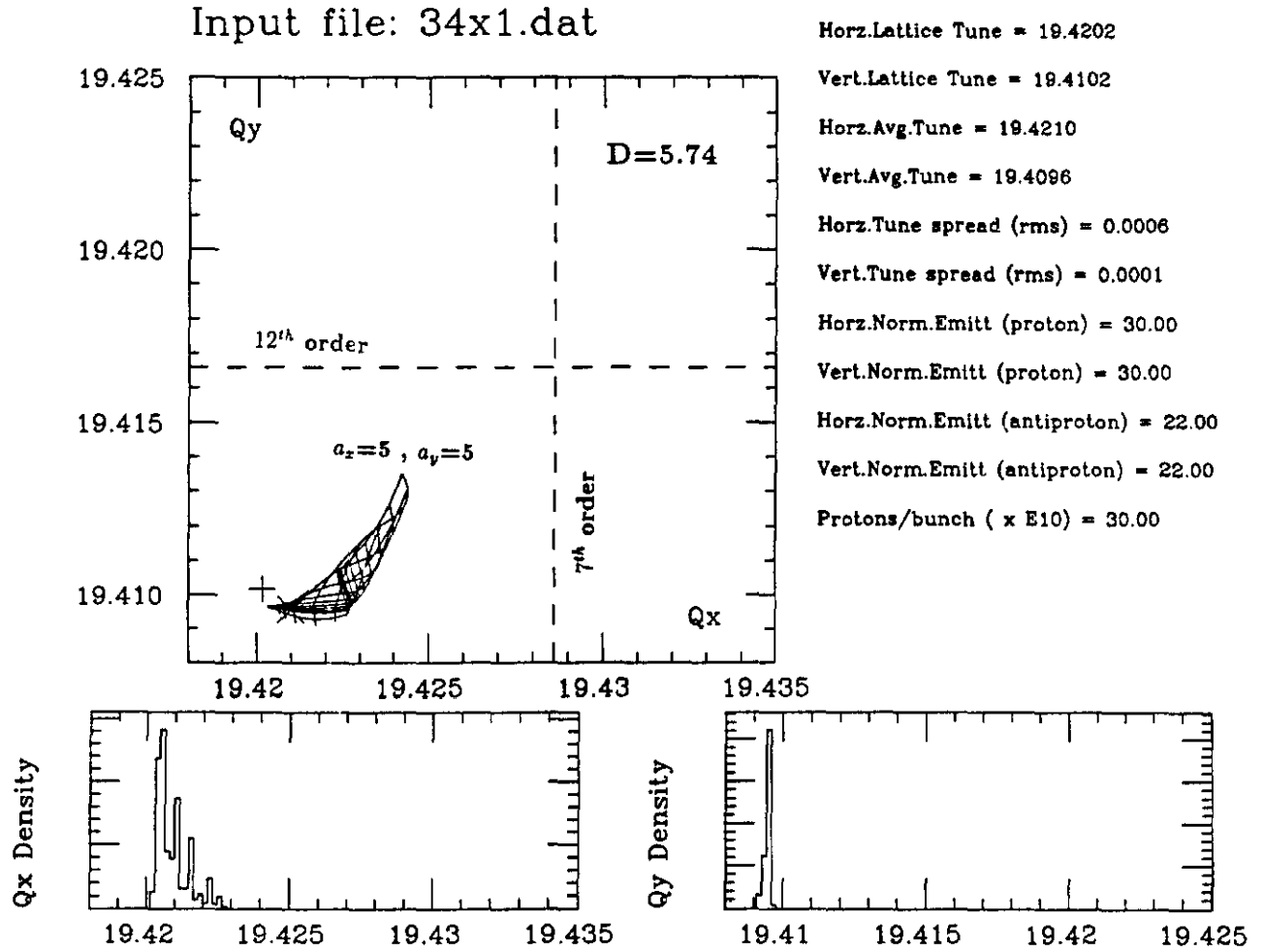
Figure 11: Tuneshift-footprint for the 34x1.dat lattice when D is increased from 4.80 to 5.74. The size of the footprint area is reduced by a factor of 3. The average tune shift is also reduced by a factor of 3.
