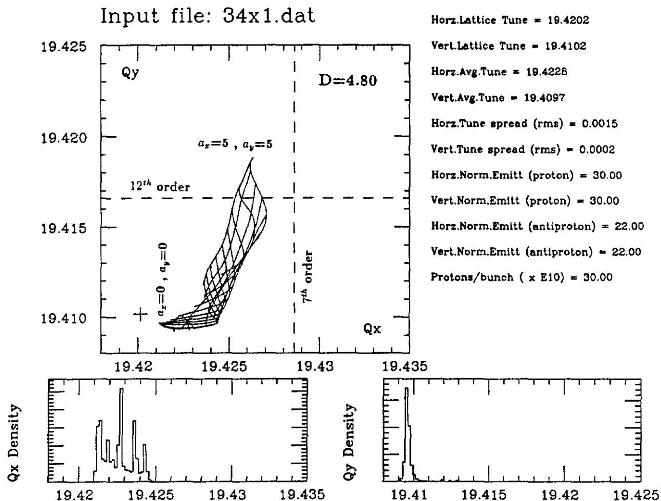
Figure 10: Tuneshift-footprint for the 34x1.dat lattice. All beam-crossings involve long-range interactions. The overall footprint area (tune spread) due to long-range interactions cannot be ignored.
