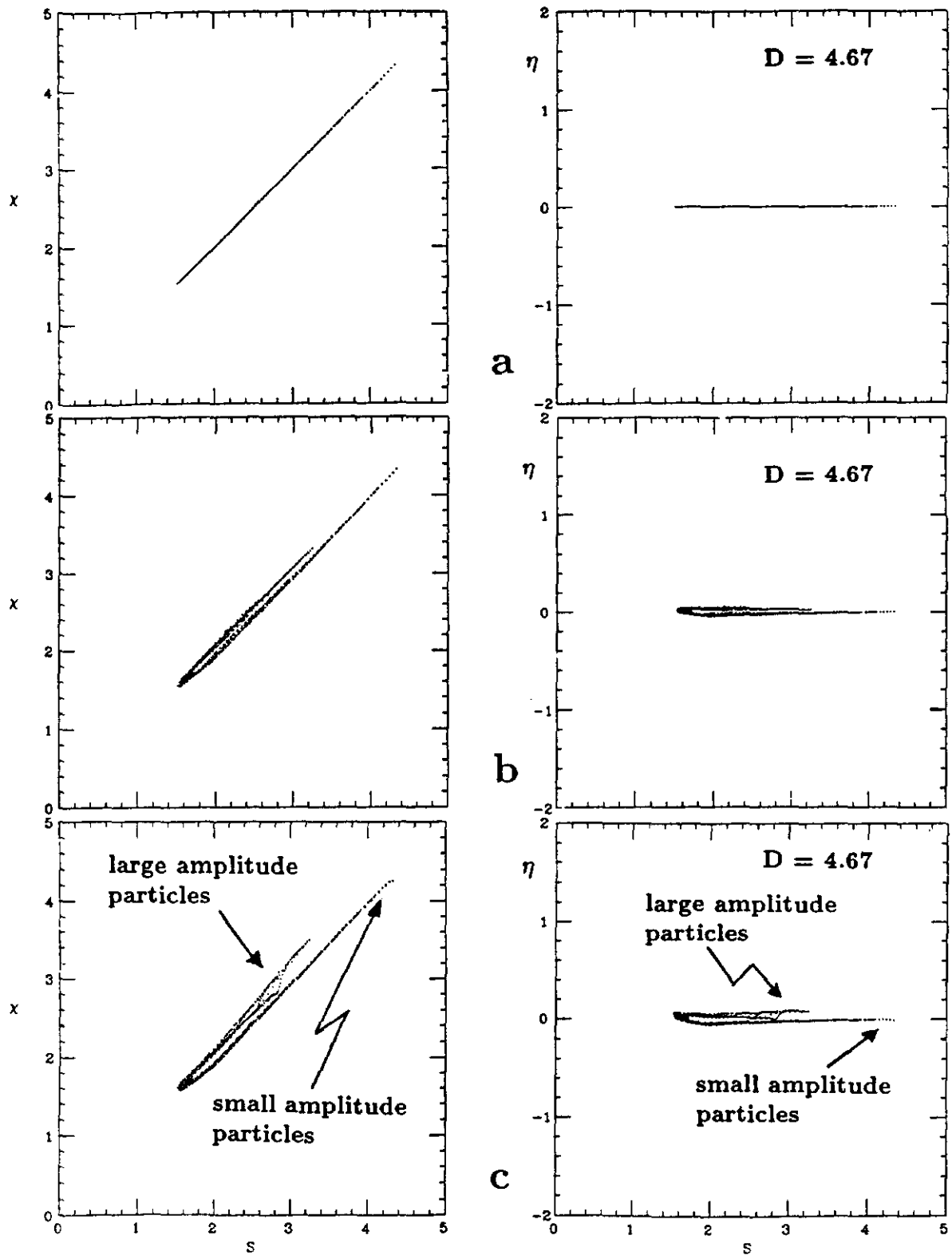
Figure 6: \chi - S Diagrams for the 1992 Collider Run. a) no beam-beam interactions b) only head-on interactions c) 2 head-on, 10 long-range interactions. In the 1992 Collider Run, long-range interactions will not be an issue since the difference between b) and c) is small.
