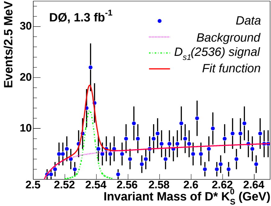
Figure 5.19: Invariant mass of D^*K_S^0 . Shown is the result of the fit of the D^*K_S^0 mass with an exponential plus polynomial function with a threshold cutoff at M(D^*) + M(K_S^0) to model the background and a double Gaussian with the same means to model the signal. The total number of D_{s1}(2536) candidates in the peak is 46.3 \pm 9.5(\text{stat.}) .
