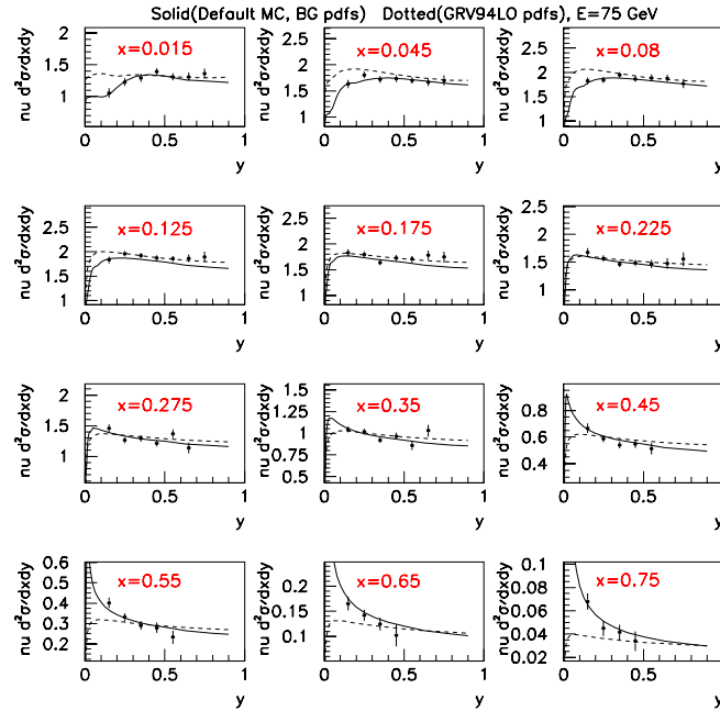
Figure 5.47: LO cross section prediction using GRV94LO (dotted curve) versus default BGPAP (solid curve) compared to CCFR data at E_\nu = 75 GeV.
