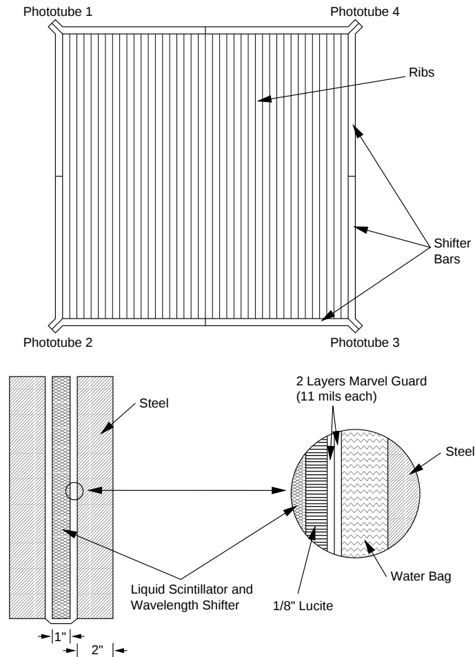
Figure 3.12: Front and side views of a NuTeV scintillation counter.
