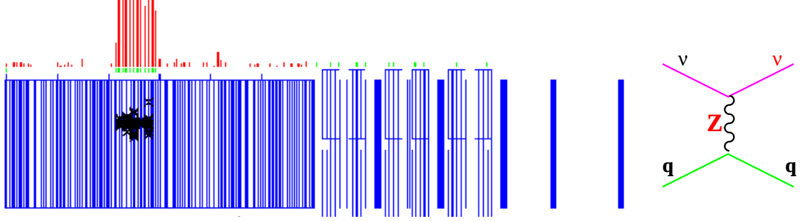
Figure 4.6: A typical NC event in the NuTeV detector.
