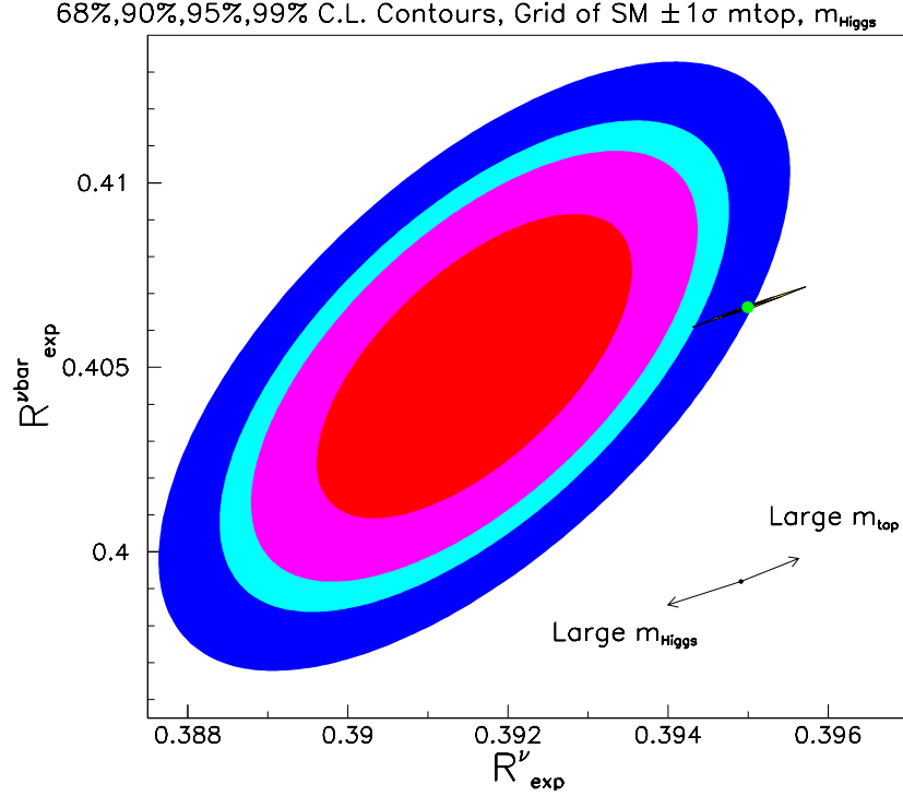
Figure 8.3: Experimental constraint on R_{\text{exp}}^\nu and R_{\text{exp}}^{\bar{\nu}} . Ellipses indicate the allowed regions at 68%, 90%, 95% and 99% confidence levels. The standard model expectation is indicated by the small dot; the “wings” indicate how the standard model prediction would shift for \pm 1\sigma variations in M_{\text{top}} and M_{\text{Higgs}} . The large arrows indicate the direction of increasing M_{\text{top}} and M_{\text{Higgs}} .
