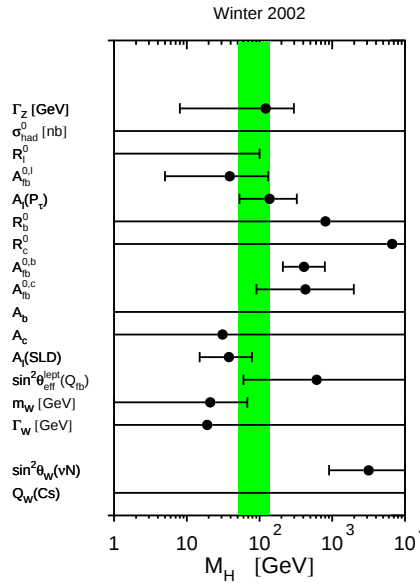
Figure 8.10: Sensitivity of the precision electroweak data to M_{\text{Higgs}} . Most of the data is consistent with a low M_{\text{Higgs}} , except for A_{FB}^{0,b} and NuTeV \sin^2 \theta_W . The NuTeV result favors large M_{\text{Higgs}} , but not with sufficient precision to pull the overall fit. Plot courtesy of LEPEWWG [73].
