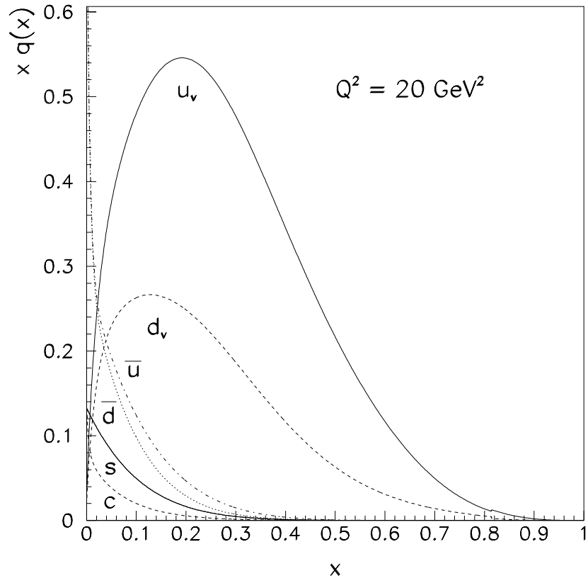
Figure 5.9: Parameterization of the BGP model parton distribution functions, x q(x) , plotted as a function of x at Q^2 = 20 \text{ GeV}^2 . The area underneath each curve represents the total momentum fraction carried by each constituent.
