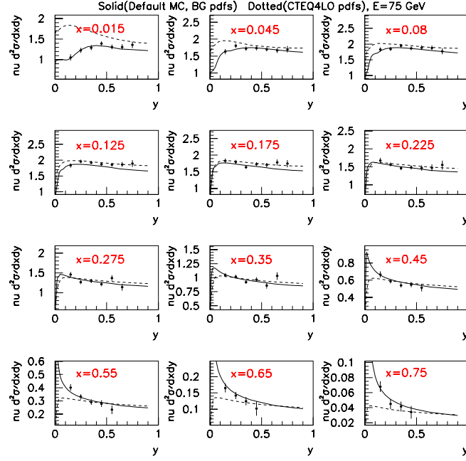
Figure 5.46: LO cross section prediction using CTEQ4LO (dotted curve) versus default BGPAP (solid curve) compared to CCFR data at E_\nu = 75 GeV.
