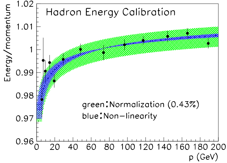
Figure 3.17: Hadron energy response as a function of testbeam momentum for testbeam hadron data ranging in energy from 4.8 to 190 GeV. The larger band reflects the overall 0.43% uncertainty in the hadron energy scale. The narrow inner curve is the result of a fit to Groom’s parameterization [27] with e/h = 1.079 \pm 0.011 , where e is the detector response to electrons and h is the response to hadrons.
