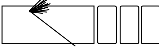
Figure 5.64: Illustration of a long event near the edge of the detector. The shower leaks out the side of the detector.
