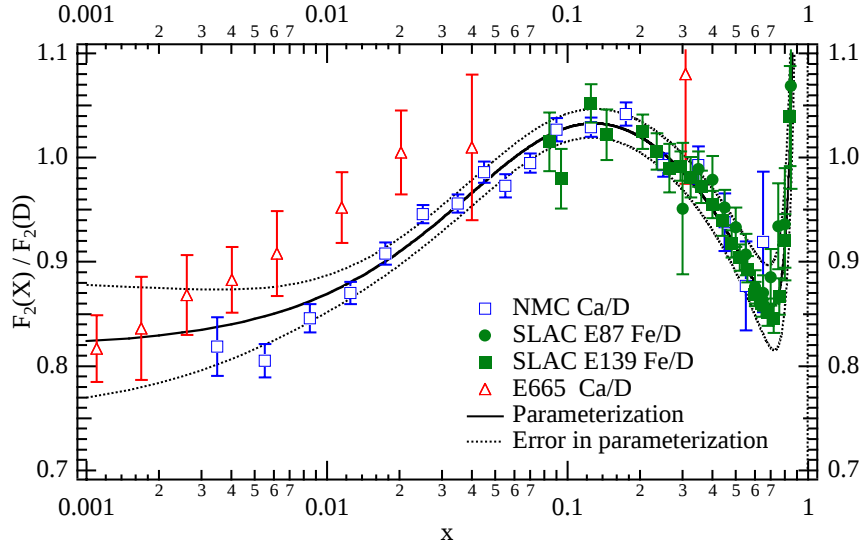
Figure 5.45: The ratio of F_2 on heavy nuclei to F_2 on deuterium as measured from charged lepton scattering data (SLAC [55], NMC [56], E665 [57]). The data is parametrized by the functional form: F_2(N)/F_2(D) = 1.0963 - 0.36427x - 0.27805 \exp^{-21.936x} + 2.7715x^{14.417} [58].
