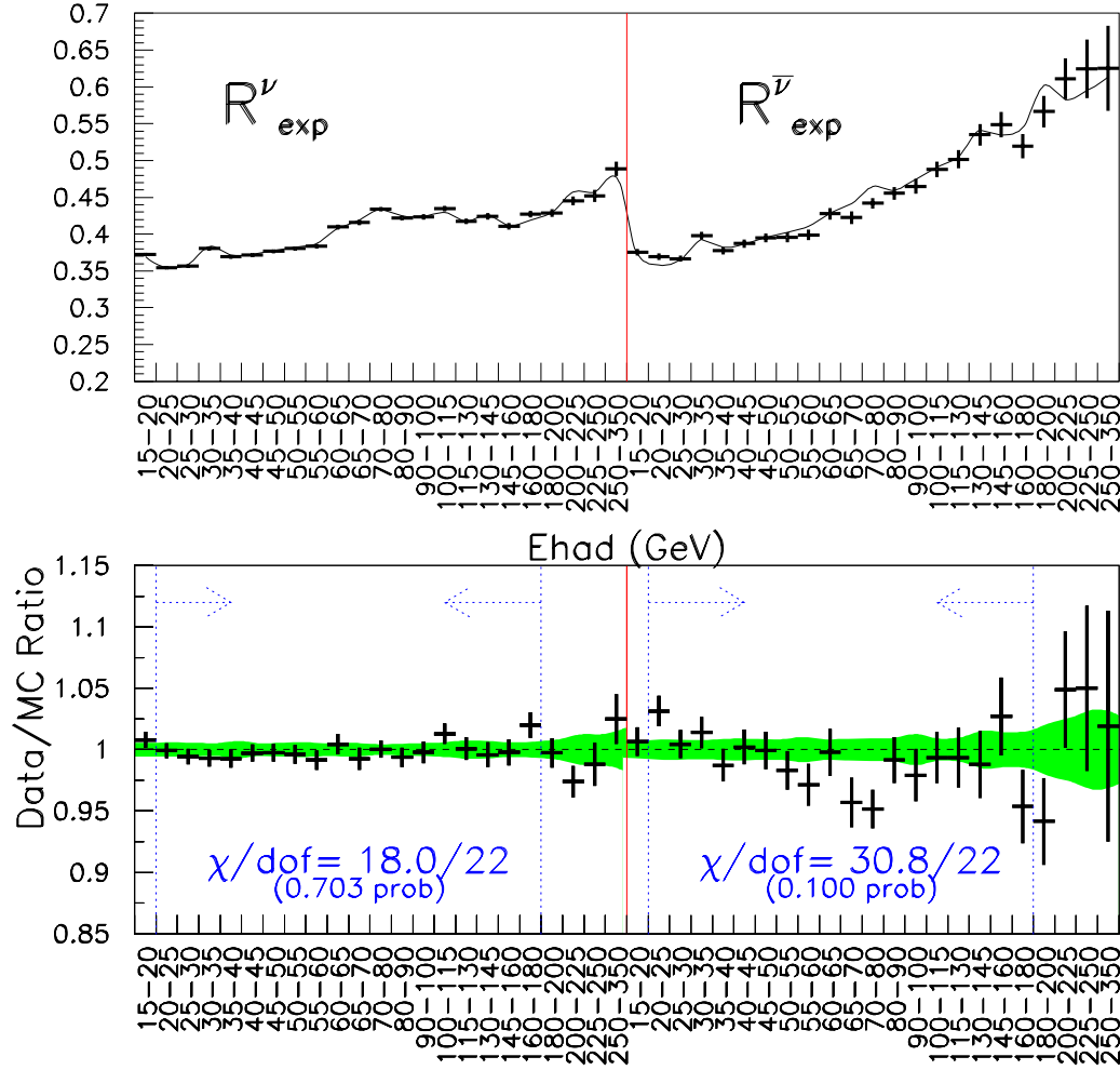
Figure 6.15: R_{\text{exp}} distributions in data and Monte Carlo as a function of E_{\text{had}} . The band on the bottom data/MC ratio plot indicates the \pm 1 \sigma systematic uncertainty. The arrows indicate the range of data included in the final analysis, namely 20 \leq E_{\text{had}} \leq 180 \text{ GeV} .
