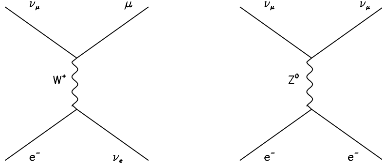
Figure 5.31: Diagrams depicting CC and NC \nu_\mu –electron scattering.
