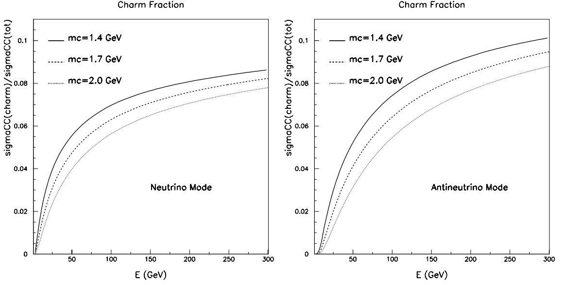
Figure 5.22: Effect of the slow rescaling model threshold suppression on the predicted charm fractions, \sigma_{CC}^{\text{charm}}/\sigma_{CC}^{\text{tot}} , shown over a varying range of m_c .
