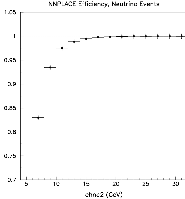
Figure 4.12: Efficiency of the longitudinal vertex finding algorithm as a function of hadron energy (variable ehnc2 ).
