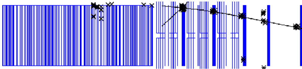
Figure 5.63: An event with significant lateral shower leakage out the side of the NuTeV detector. This event was recorded with E_{\text{had}}=17 GeV, \text{PLACE}=32 , V_x=40 inches, V_y=-4 inches, and a length of 8 counters.
