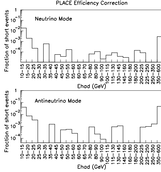
Figure 4.13: PLACE efficiency correction for short events as a function of E_{\text{had}} .
