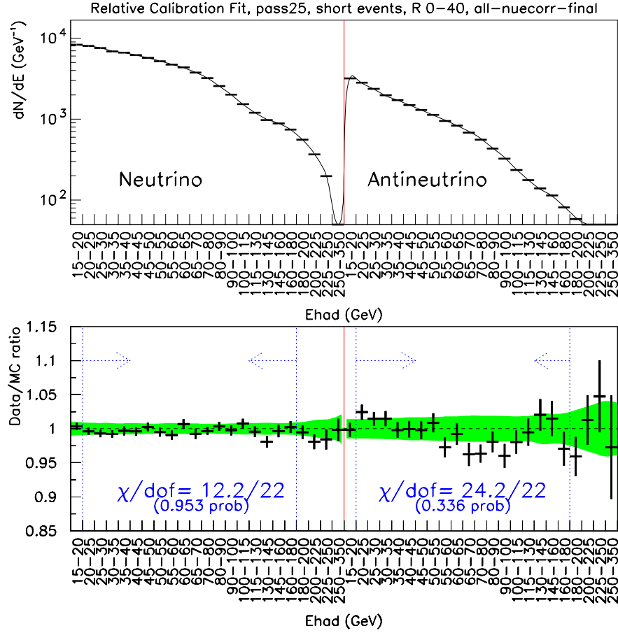
Figure 5.59: Short event E_{\text{had}} distributions after including the measurement of high energy \nu_e 's from the data. The bands display the \pm 1\sigma systematic uncertainty.
