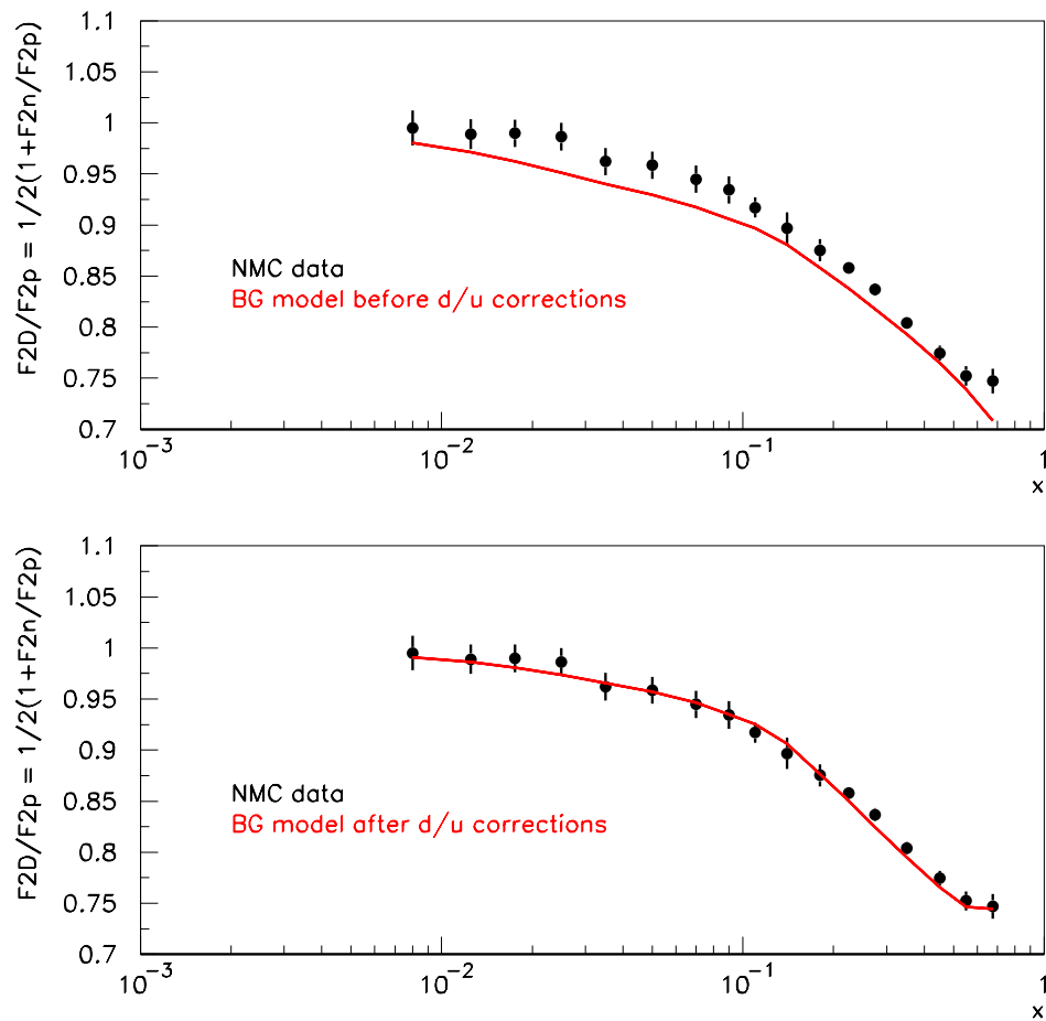
Figure 5.12: Comparison of BGPARG F_2^n/F_2^p model prediction to NMC data [37, 41] both before (top) and after (bottom) the d/u corrections have been applied to the sea and valence.
