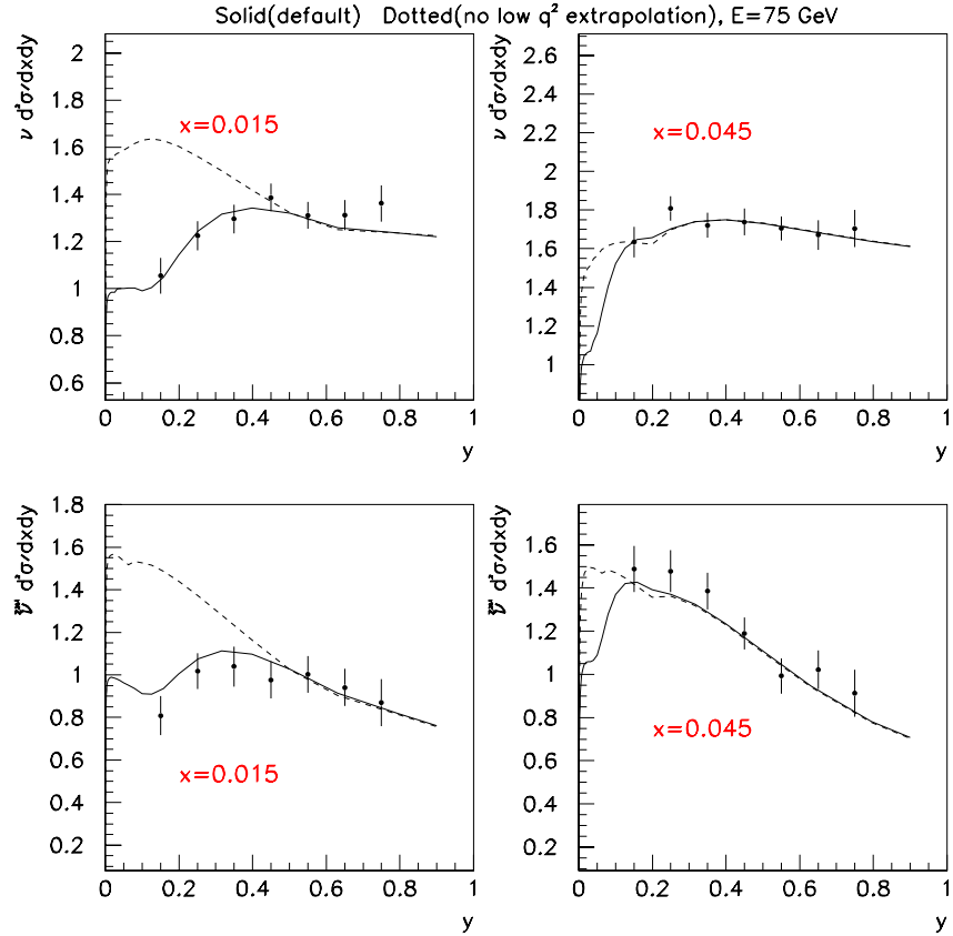
Figure 5.14: Improvement in the low x differential cross section model prediction after incorporating the GRV-based low Q^2 extension to the BGPAP PDFs. The plot displays CCFR neutrino (top) and antineutrino (bottom) cross section data at E_\nu = 75 \text{ GeV} . The dotted curve is the model prediction before the low Q^2 extrapolation, the solid curve is the result after adopting the low Q^2 extrapolation.
