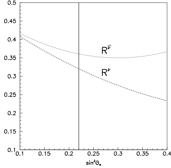
Figure 2.2: Dependence of R^\nu and R^{\bar{\nu}} on \sin^2 \theta_W assuming r = 1/3 . Over the region of interest, R^\nu has a larger slope than R^{\bar{\nu}} and as a result, roughly 30 times more sensitivity to \sin^2 \theta_W .
