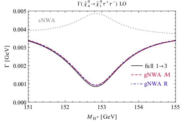
Figure 4: The 1→3 decay width of \tilde{\chi}_4^0 \rightarrow \tilde{\chi}_1^0 \tau^+ \tau^- at tree level with contributions from h, H including their interference (black) confronted with the NWA: sNWA without the interference term (gray, dotted), gNWA including the interference term based on on-shell matrix elements denoted by \mathcal{M} (red, dashed) and on the R-factor approximation denoted by R (blue, dash-dotted).
