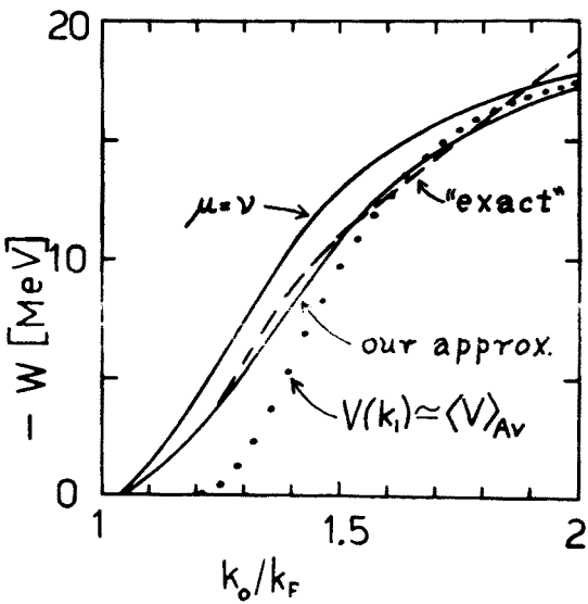
Fig. 2. Our results for W for the Reid hard core potential (at k_{F0} = 1.4 \text{ fm}^{-1} ), compared with the “exact” results of [6]
