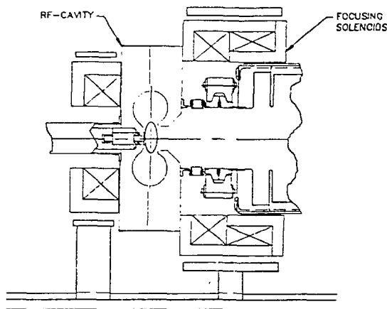
Figure 2: AWA photocathode electron source.
