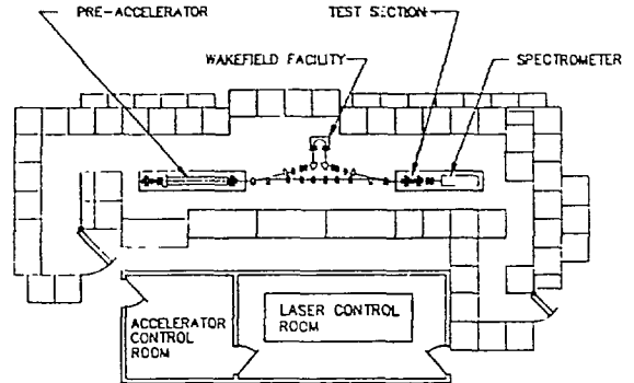
Figure 1: Plan view of Phase-I of the Argonne Wakefield Accelerator.
