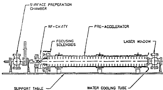
Figure 3: AWA photocathode gun and preaccelerator.
