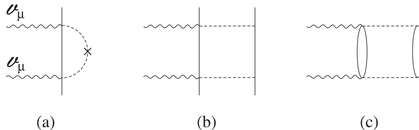
Fig. 1. Illustration of a mixing effect in the vector correlator (a) in the heat bath (denoted by a cross), (b) equivalent diagram in the nucleus with its translation (c) in many-body diagrams.
