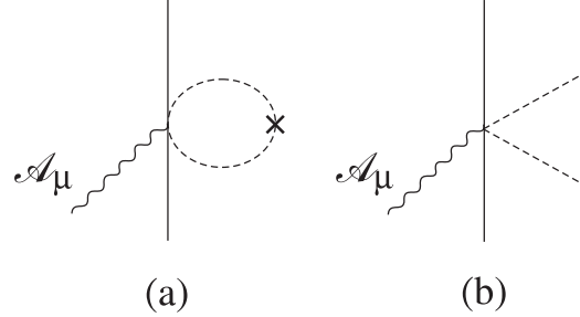
Fig. 2. Renormalization of the nucleonic axial coupling constant (a) — by a pion loop in the hot pion gas (the cross denotes the heat bath), (b) — by the virtual pion cloud in the nucleus.
