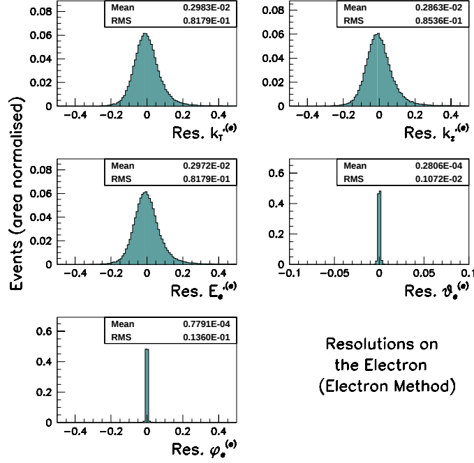
Figure 5.5: Resolutions of the laboratory frame positron's 4-momentum as reconstructed with the electron method (denoted "(e)"). ( k_T refers to the positron's transverse momentum). The angular variables were corrected as explained in the text (kinematic range defined in section 5.6.2).
