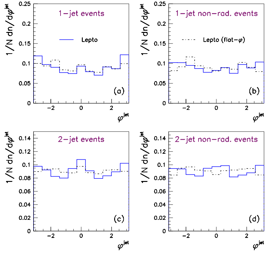
Figure 8.5: \phi^{\text{jet}} distributions at detector level obtained with Lepto and with the “flat- \phi ” Lepto: (a) 1-jet events, (b) 1-jet non-radiative events, (c) 2-jet events and (d) 2-jet non-radiative events.
