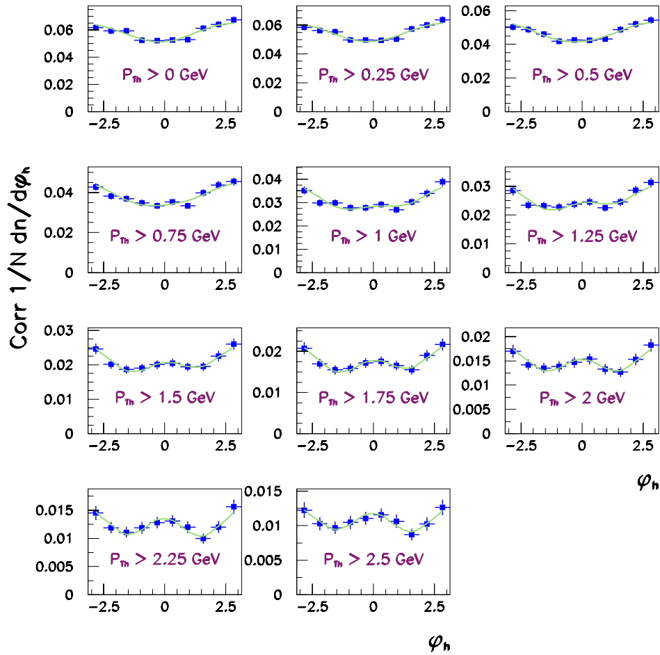
Figure 6.15: Bin-by-bin corrected \phi_h distributions in the HCM frame as a function of the minimum transverse momentum – P_{T^h} cut – of the tracks. The solid lines show the result of the fit of the distributions to the theoretical form of equation 6.7. The Ariadne MC was used to correct the data.
