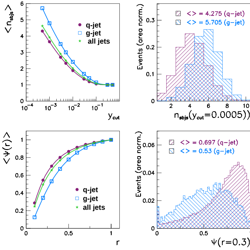
Figure 9.10: The subjet multiplicity n_{sbs} and integrated jet shape \Psi(r) for quark and gluon jets at hadron level: means and differential distributions for a specific value of y_{cut} and r , respectively.
