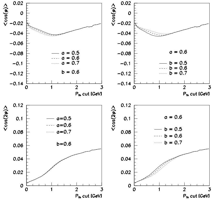
Figure 10.1: Theoretical calculations obtained with the program AZICAL for the moments \langle \cos \phi \rangle and \langle \cos 2\phi \rangle as a function of the P_{Th} cut on the hadrons. The distributions show the influence of the intrinsic parton k_T ( a parameter) and the hadronisation p_T ( b parameter) on the moments ( a and b are given in GeV).
