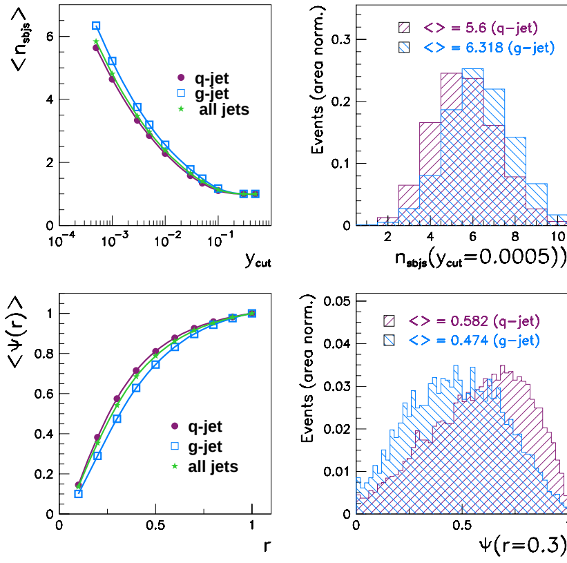
Figure 9.14: The subject multiplicity n_{sbs} and integrated jet shape \Psi(r) for quark and gluon jets at detector level: means and differential distributions for a specific value of y_{cut} and r , respectively.
