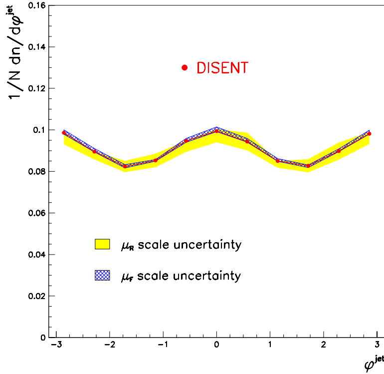
Figure 10.4: NLO QCD prediction obtained with DISENT for the \phi^{\text{jet}} distribution of dijet events. The solid (yellow) band represents the uncertainty on the renormalisation scale \mu_R , calculated using \mu_R = 2Q, Q/2 instead of the central value \mu_R = Q . The hatched (blue) band are represents the uncertainty on the factorisation scale \mu_F , calculated using \mu_F = 2Q, Q/2 instead of the central value \mu_F = Q .
