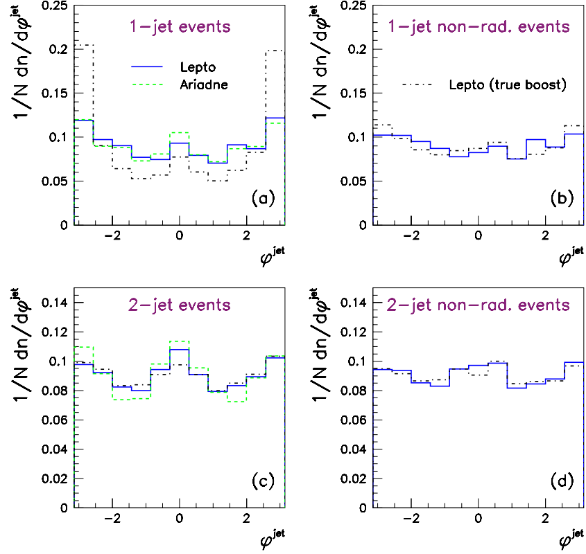
Figure 8.2: \phi^{jet} distributions at detector level obtained with Lepto and Ariadne: (a) 1-jet events, (b) 1-jet non-radiative events, (c) 2-jet events and (d) 2-jet non-radiative events. Distributions were also obtained with Lepto using the true components of the boost vector to boost the jets at detector level “(true boost)”.
