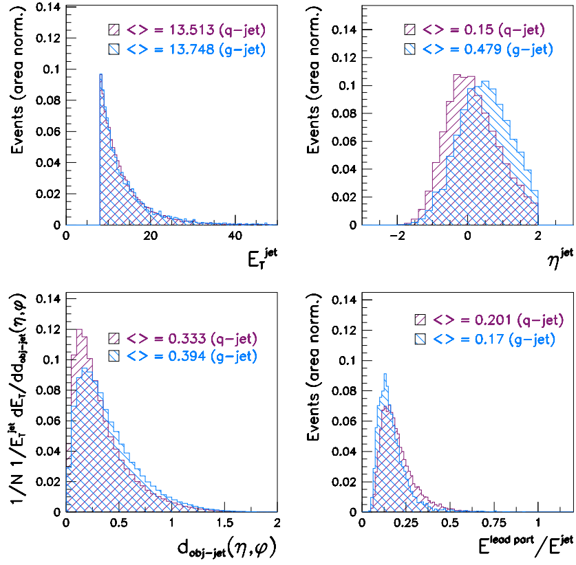
Figure 9.13: Some discriminating variables investigated at detector level: quark and gluon jet distributions of E_T^{\text{jet}} , \eta^{\text{jet}} , E_T differential distribution in the \eta - \phi distance of particles within a jet, and distribution of the fractional energy of the leading particle in the jet ( E^{\text{lead part}}/E^{\text{jet}} ). All variables were computed in the Breit frame.
