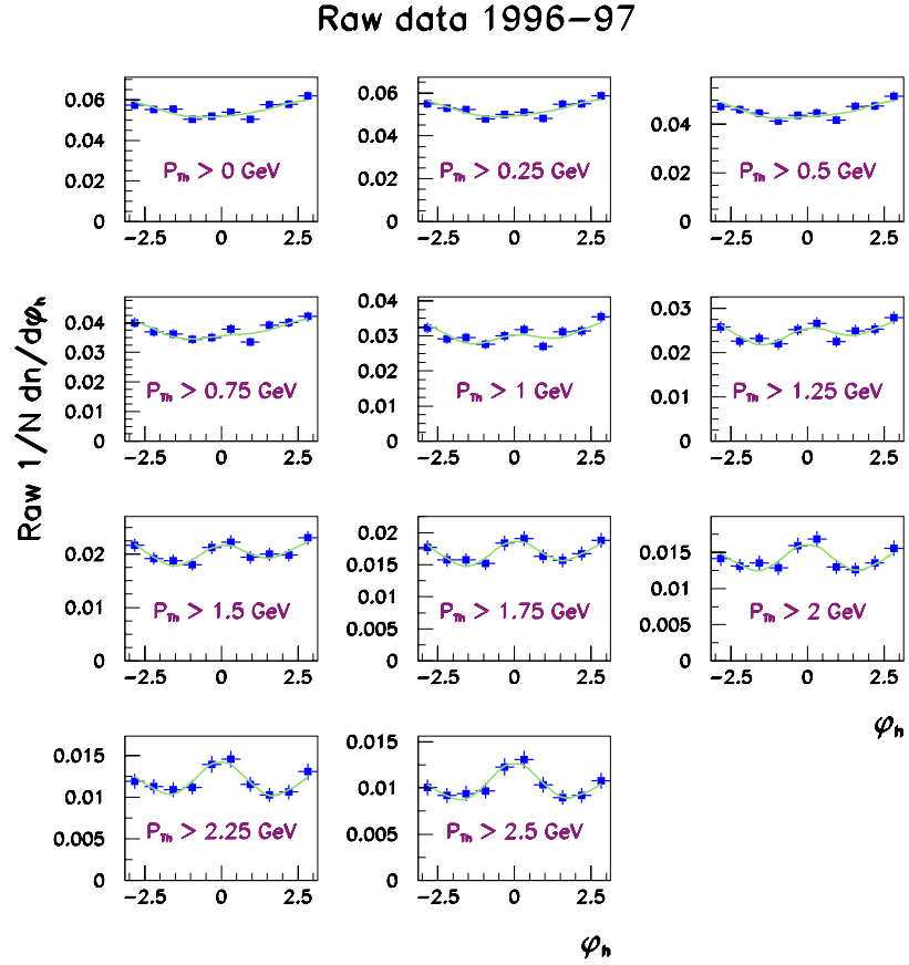
Figure 6.10: The uncorrected \phi_h distributions (raw data) in the HCM frame as a function of the minimal transverse momentum P_{Th} of the tracks. The lines are the result of a fit, and are merely to guide the eye (refer to the text for further details).
