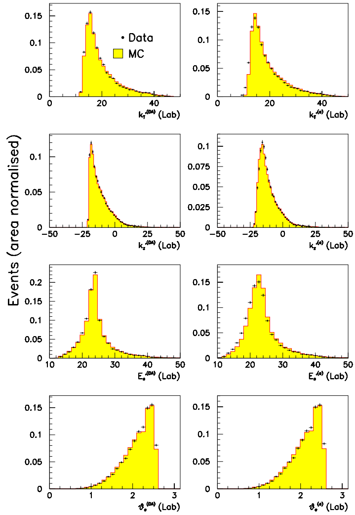
Figure 5.11: Comparisons between the data and Ariadne for the positron variables in the laboratory frame as reconstructed with the DA and electron methods.
