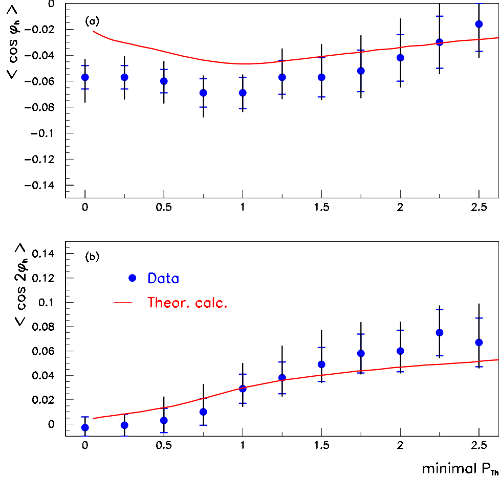
Figure 11.2: Evolution with the minimal transverse momentum P_{Tn} of the tracks of the \langle \cos \phi_h \rangle and \langle \cos 2\phi_h \rangle moments of the \phi_h distributions: comparison of data with QCD theoretical calculations performed with the AZICAL program.
