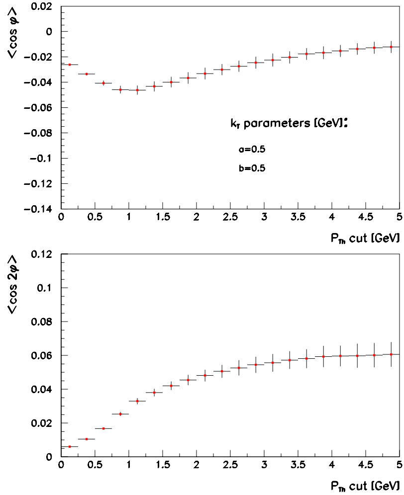
Figure 10.3: Theoretical calculations obtained with the program AZICAL for the moments \langle \cos \phi \rangle and \langle \cos 2\phi \rangle as a function of the P_{Th} cut on the hadrons. The error bars represent the numerical uncertainty in the calculations.
