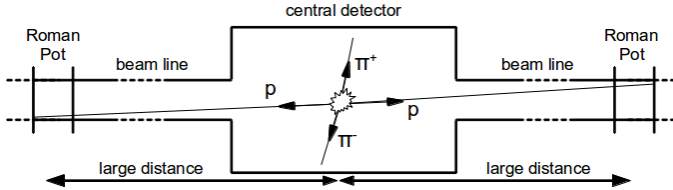
Fig. 2. The layout of the general experimental setup. Main detector in the center and forward proton taggers (Roman Pots).
