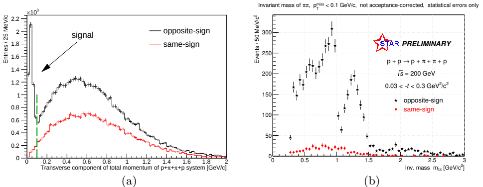
Fig. 4. (a) Transverse momentum ( \Delta p_T ) balance between centrally produced \pi\pi system and the outgoing protons detected in the Roman Pots; (b) Reconstructed, uncorrected mass distributions, dN/dt , for two charged pions in the inclusive central diffraction at \sqrt{s} = 200 GeV. Asterisk points are for neutral states and solid circles (grey/red) represent charged states. Errors are statistical only.
