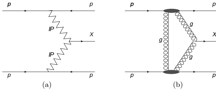
Fig. 1. (a) Central Production diagram in DPE; and (b) pQCDPicture.
