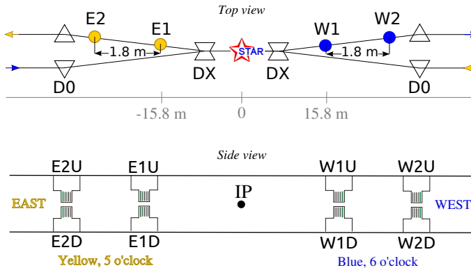
Fig. 3. The layout of the RPs with the STAR detector (not to scale). The Roman Pot setup at STAR for measuring forward protons with high- t . Two sets of RPs will be positioned between DX and D0 magnets, at 15.8 m and 17.6 m from the IP. Top and side view are shown.
