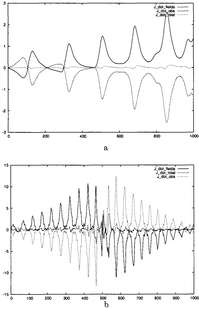
Figure 5.14: Plots of the time derivative of the total angular momentum, \dot{J}_{tot} and its components \dot{l}_{fields} and \dot{l}_{obs} as a function of time for a two different systems: a) d=6 skyrmion configuration with b=2 for \Gamma=0.25 and b) d=5 skyrmion configuration with b=2 for \Gamma=-0.5
