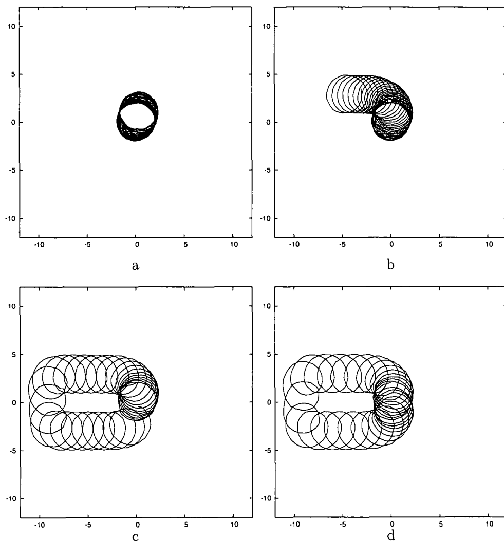
Figure 5.8: Plots of the trajectories for the upper skyrmions in a system with an asymmetric potential hole of width b = 2 with d = 4 for various values of \Gamma : a) \Gamma = -0.1 , b) \Gamma = -0.2 , c) \Gamma = -0.4 and d) \Gamma = -0.5 , where the horizontal axis represents the x coordinate and the vertical axis the y coordinate.
