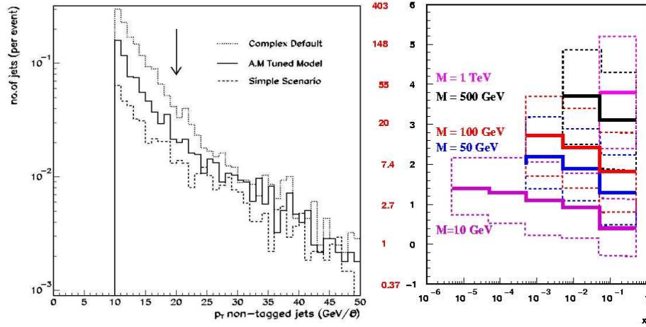
Fig. 4. Left: Number of central jets per event in an analysis of H \rightarrow WW^* \rightarrow 2l for different models/assumptions of the underlying event. The study was performed with ATLFast. Right: The k_T from QCD evolution for different values of the mass of a produced system M in gg \rightarrow M .
