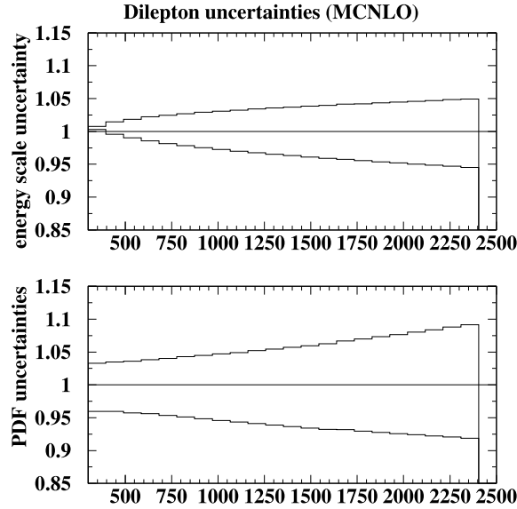
Fig. 1. Dilepton production uncertainty bands, arising from the NLO scale dependence (top), and from structure functions (bottom), as a function of the dilepton invariant mass ( \text{GeV}/c ).
