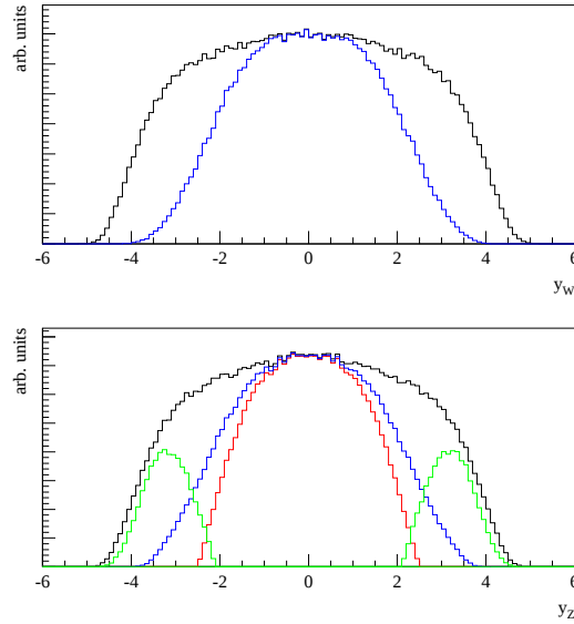
Fig. 7. Top: full rapidity range covered by W production (outer histogram), and the range covered after selections ( cf. Section 2). Bottom: full rapidity range covered by Z production (outer histogram); the range covered when requiring two leptons within \eta < 2.5 (inner histogram); when allowing for one forward electron, \eta < 4.9 (intermediate histogram); finally, the two symmetric histograms at high rapidity show the LHCb acceptance.
