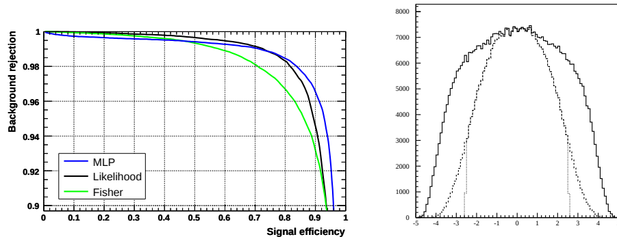
Fig. 4. Left: performance of electron identification in the ATLAS forward calorimeter [7]. Right: Z rapidity acceptance when both electrons have |\eta| < 2.5 (inner histogram); when one electron has |\eta| < 2.5 , and the other has |\eta| < 4.9 (intermediate histogram); and the full distribution (outer histogram).
