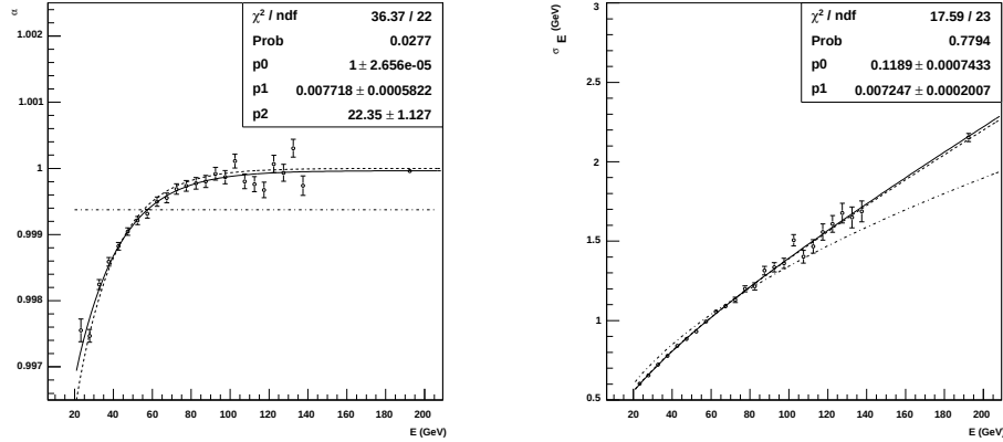
Fig. 9. Measurement of scale (left) and resolution (right) as a function of the lepton energy, in Z boson decays [10].
