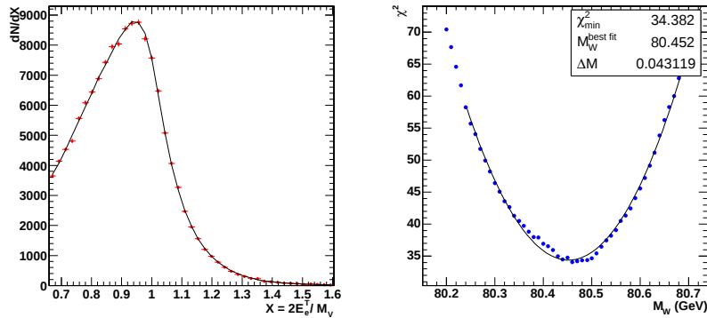
Fig. 5. Left: an example lepton p_T distribution. The falling edge at p_T \sim m_W/2 reflects the W boson mass. Right: \chi^2 graph resulting from the comparison of the distribution on the right with a series of “template” distributions of the same variable, obtained by varying the W mass.
