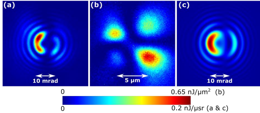
FIG. 4: Color online. (a) COTR angular distribution pattern for shot with vertical dark band due to interference of two beamlets. (b) y-polarized NF image on same shot, showing two double-lobed patterns. (c) COTRI image reconstructed from two-beamlet model. Color legend applies to all panels.
