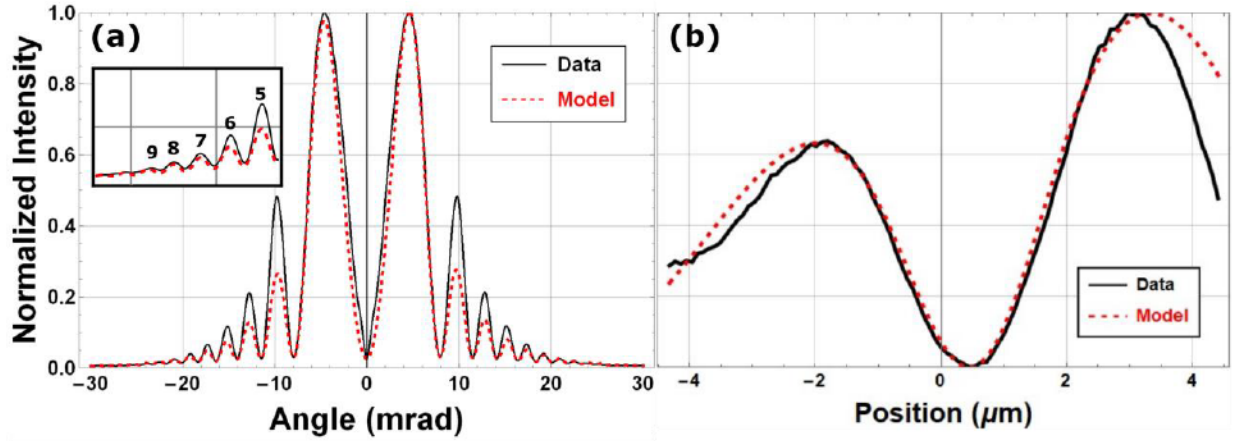
FIG. 3: Color online. (a) Azimuthally averaged COTRI fringes vs. \theta from Fig. 1d (solid black curve). See Supplementary Material for description of averaging procedure. Inset: outermost fringes magnified. Dotted red curve: analytical COTRI model using s_q = 0.33 mrad, and \sigma_x = 2.75 \mu\text{m} and 6.6 \mu\text{m} at foils 1 and 2, respectively. (b) x -projection of NF image in Fig. 1c from same shot (solid black curve), with COTR model using \sigma_x = 2.75 - \mu\text{m} (dotted red curve).
