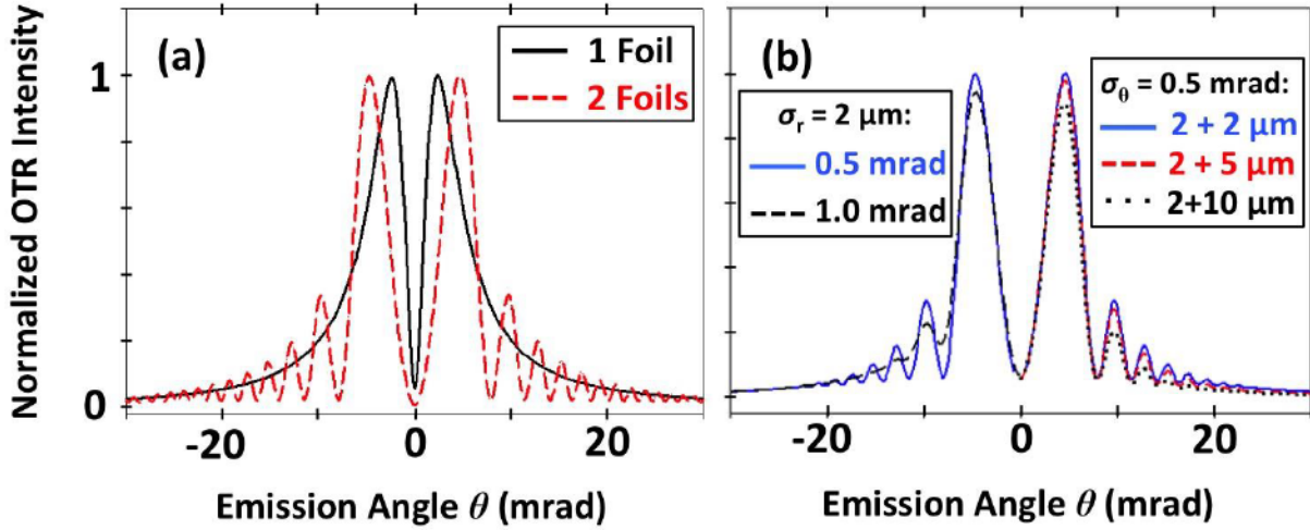
FIG. 2. Color online. (a) Analytical calculations of angular distributions of OTR at \lambda = 633 \pm 5 nm generated by 200 MeV electron bunch with divergence \sigma_\theta = 0.2 mrad: in one foil (solid black curve) and in a two-foil interferometer with L = 18.5 mm and beam radius s_r^{(1)} = s_r^{(2)} = 2 \mu\text{m} at both foils 1 and 2 (dashed red). (b) Calculated dependence of COTRI fringe visibility on \sigma_\theta and \sigma_r . \theta < 0 : beam-divergence effect for \sigma_\theta = 0.5 mrad (solid blue curve) and 1.0 mrad (dashed black) for s_r^{(1)} = s_r^{(2)} = 2 \mu\text{m} . \theta > 0 : effect of expanding s_r^{(2)} for fixed s_r^{(1)} = 2 \mu\text{m} , \sigma_\theta = 0.5 -mrad, with curves labeled s_r^{(1)} + s_r^{(2)} \mu\text{m} in legend.
