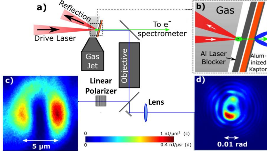
FIG. 1: Color online. (a) Schematic setup showing path of LPA drive laser pulse (red), gas jet, OTR foil, Si mirror, and OTR imaging-detection configuration. (b) Detail of gas jet exit, showing e -bunch, drive laser path, blocking foil and aluminized Kapton OTR foil. (c) NF data at 600 nm, imaged from Kapton foil to CCD through linear polarizer, showing two point-spread function lobes. (d) FF data at 633 nm for same shot, recorded with compound lens (microscope objective + single-element lens) and no polarization analyzer, showing interference fringes. Angular resolution: 0.35 \pm 0.05 mrad/pixel, or \sim 6 pixels/fringe at eighth fringe. Color legend applies to (c) and (d).
