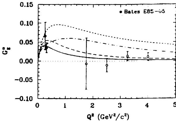
Fig. 2. Recently reported values of G_E^n : quasielastic {}^2\text{H}(\vec{e}, e'\vec{n}) reaction (shaded circle), exclusive {}^3\text{He}(\vec{e}, e'n) by Meyerhoff et al. [27] (shaded square), and the inclusive quasielastic {}^2\text{H}(e, e') results of Lung et al. [28] (open circles). The parameterizations are from the work of Galster et al. [29] G_E^n = -\tau\mu_n(1 + 5.6\tau)^{-1} (long dashes), Platchkov et al. [1] where the Paris potential fit is shown (solid), the Gari-Krumpelmann VMD-PQCD model 3 (dash-dot) and the parameterization G_E^n = -\tau G_M^n (short dashes) where F_{1n} = 0 .
