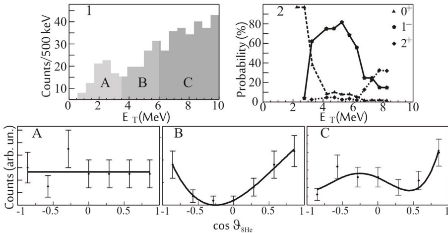
Fig. 1. The 2n transfer reaction ^3\text{H}(^8\text{He}, p)^{10}\text{He} as studied in Refs. [19, 20]. (1) Missing mass spectrum obtained for the ^{10}\text{He} nucleus; (2) Squared amplitudes of coherent s -, p -, d -wave contributions deduced from the angular distributions of ^8\text{He} appearing at the ^{10}\text{He} decay. The lower three panels show these angular distributions averaged over the energy ranges marked A, B, and C in panel 1.
