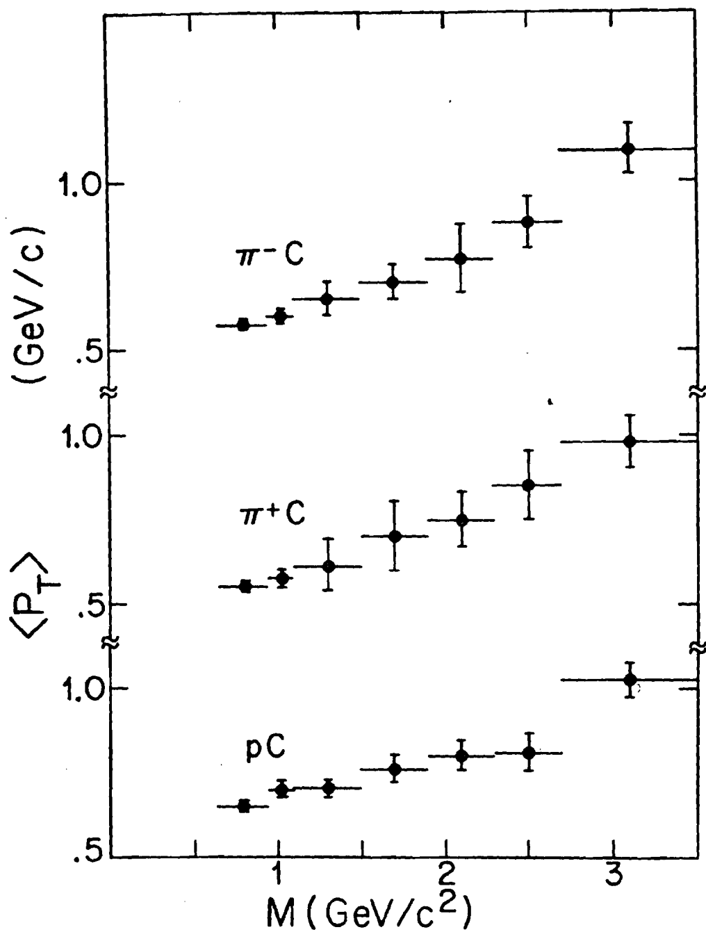
FIGURE 5-32. PLOTS OF \langle P_T \rangle VERSUS MASS FOR \pi^+ , \pi^- AND PROTONS INCIDENT ON CARBON.
