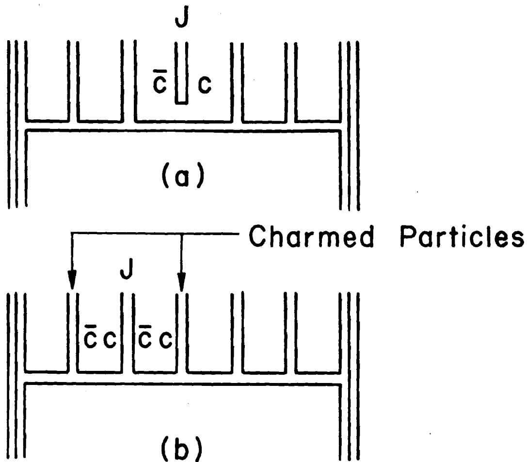
FIGURE 1-1. TWO QUARK-LINE DIAGRAMS FOR J PRODUCTION. (A) THIS DIAGRAM IS NOT ALLOWED BY THE OZI RULE BECAUSE THERE IS A DISCONNECTED QUARK-LINE. (B) THIS IS AN OZI ALLOWED DIAGRAM. A PAIR OF CHARMED PARTICLES IS PRODUCED IN ASSOCIATION WITH THE J ALLOWING ALL QUARK-LINES TO BE CONNECTED.
