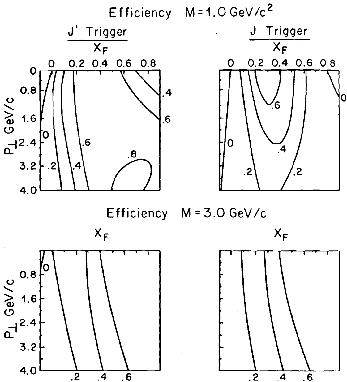
FIGURE 4-11. CONTOUR PLOTS OF EFFICIENCY AND DISTORTION VERSUS X_F AND P_{\perp} , USED TO CALCULATE E \frac{d^3\sigma}{dx_F dP_{\perp}^2}
