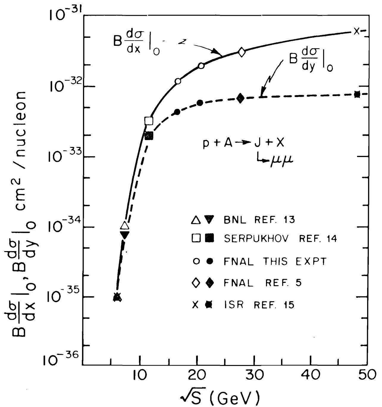
FIGURE 5-35. DEPENDENCE OF J PRODUCTION ON \sqrt{s} .
