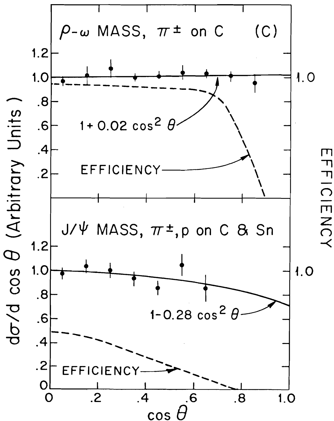
FIGURE 5-34. ANGULAR DISTRIBUTION OF J/\psi DECAY TO \mu^+ \mu^- IN THE HELICITY FRAME.
