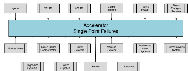
Figure 1: Single point failure diagram of the LANSCE accelerator.
