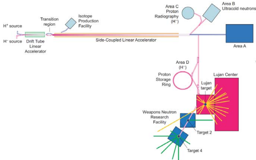
Figure 2: Graphical representation of the LANSCE accelerator.
