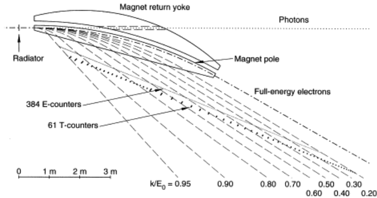
Figure 3.6: A schematic diagram of the Hall B tagger magnet and hodoscope. Dashed lines show the trajectories of recoil electrons associated with photons of given energies ( E_0 is the beam energy). The photon tagger detects recoil electrons with energies between 0.2 \times E_0 and 0.95 \times E_0 . E-counters cannot be seen individually because of their fine segmentation. Image source: [42].
