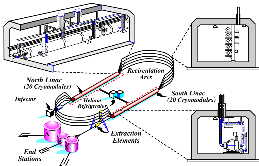
Figure 3.2: A schematic diagram of the Continuous Electron Beam Accelerator Facility. Shown in red are the LINACs composed of 168 (each) superconducting RF cavities grouped into 20 cryomodules. At top right is an exploded view of the recirculation arcs showing the five separate magnet assemblies for up to five beam passes. Experimental halls are shown at lower left. Image source: [40].
