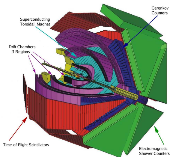
Figure 3.9: A schematic diagram of the CLAS detector. Detector subsystems are color-coded as follows: drift chambers shown in violet, toroidal magnet in light blue, TOF scintillators in red, Čerenkov detectors in dark blue, electromagnetic calorimeters in green. Image source: [38].
