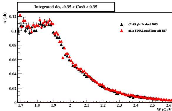
Figure 8.6: Shown above is a comparison of the differential cross section results from g1c (black) and this analysis (red) integrated over the range [-0.35, 0.35] . The g11a result includes the statistical start counter simulation as described in the text. Agreement between the two results is far better than that shown in Figure 8.2.
