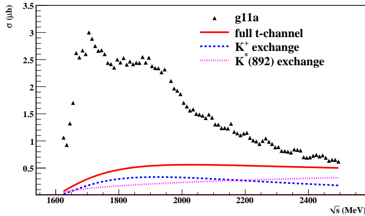
Figure 9.20: Shown above are comparisons of the total cross section (black) and projections of the alternate non-resonant model (red) and its component production mechanisms. Notice that this model has a very different contribution at low \sqrt{s} than the previous non-resonant model.
