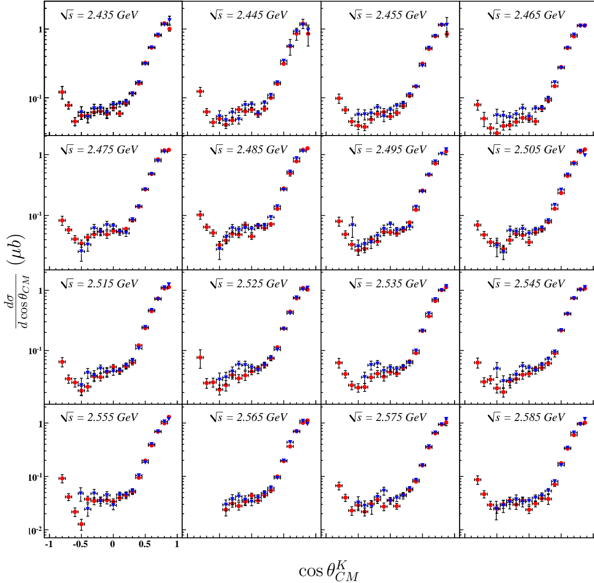
Figure 7.8: d\sigma/d\cos\theta_{CM}^K ( \mu\text{b} ) v. \cos\theta_{CM}^K : Differential cross section results for the energy range 2.43\text{ GeV} \leq \sqrt{s} < 2.59\text{ GeV} . Results from the three-track analysis are shown in blue (triangles), those of the two-track analysis in red (circles). All plots have the same \cos\theta_{CM}^K -axis range and vertical axis ranges are the same for the four plots in each row. Vertical axes are logarithmic scale.
