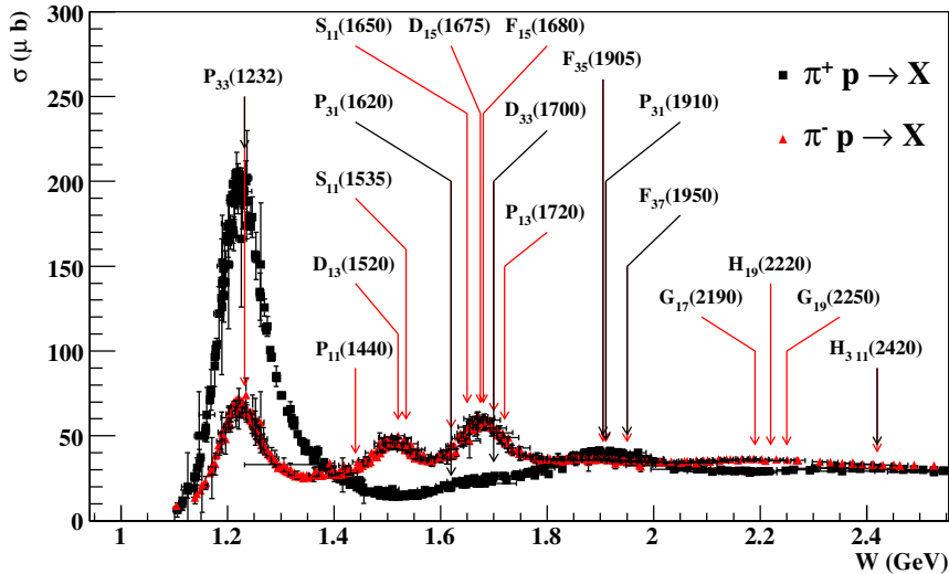
Figure 2.2: Shown above are the total cross sections from \pi p scattering experiments. The enhancements in \sigma are labeled with N^* states that are given a four-star (“existence is certain”) rating by the PDG [5]. (Image source: [4].)
