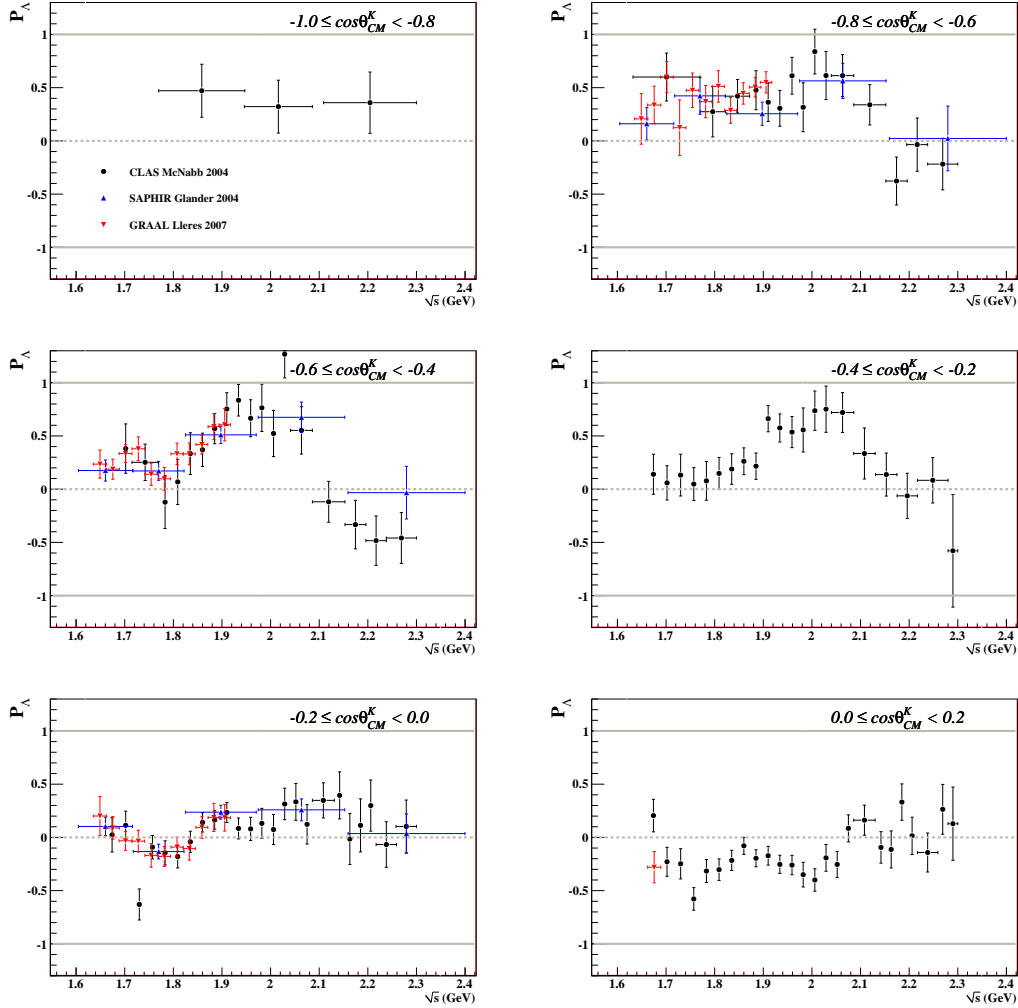
Figure 2.6: Shown above are P_\Lambda results from previous analyses of \gamma p \rightarrow K^+ \Lambda at backward and middle production angles. Each plot represents data in the 0.2-unit-wide \cos \theta_{CM}^K range indicated. Marker convention is given at top left and is the same for all plots.
