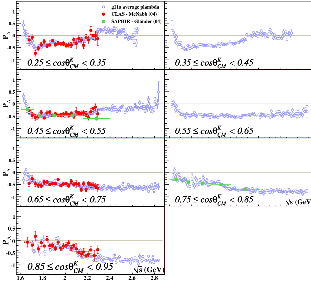
Figure 7.29: The plots above show \Lambda recoil polarization measurements from this analysis (blue), the previous CLAS (McNabb 2004) measurements (red), and the 2004 SAPHIR measurements (green) versus center-of-mass energy in bins of production angle. \cos \theta_{CM}^K ranges indicated on each plot indicate the g11a measurements plotted. Most of McNabb's measurements represent 0.2-wide \cos \theta_{CM}^K bins. SAPHIR's measurements represent roughly 30^\circ -wide angular bins. All error bars reflect statistical uncertainties only.
