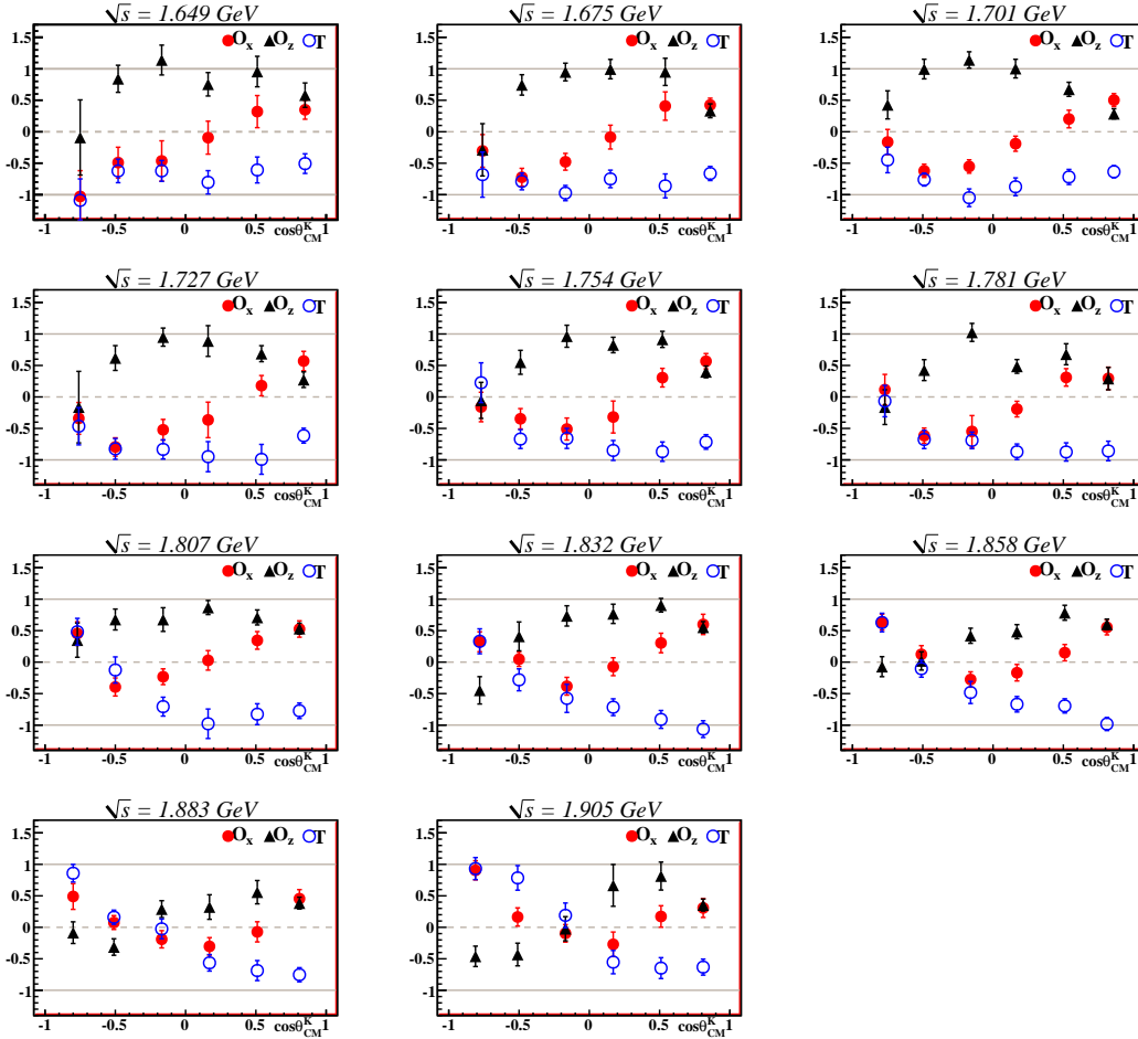
Figure 2.9: The plots above show the beam-recoil polarization transfer observable ( O_{x'} and O_{z'} ) and target asymmetry ( T ) results published by the GRAAL Collaboration in 2008 [23]. Each plot shows results at a fixed \sqrt{s} value (indicated above each plot) versus \cos\theta_{CM}^K . O_{x'} is shown in red circles, O_{z'} in black triangles, and T in open blue circles.
