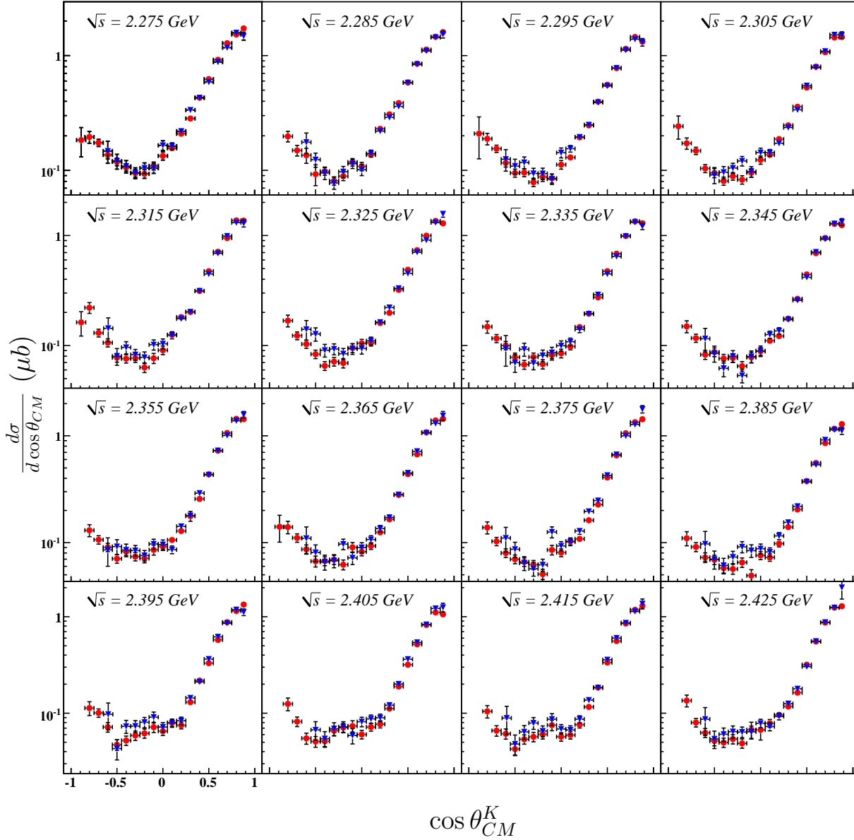
Figure 7.7: d\sigma/d\cos\theta_{CM}^K ( \mu\text{b} ) v. \cos\theta_{CM}^K : Differential cross section results for the energy range 2.27\text{ GeV} \leq \sqrt{s} < 2.43\text{ GeV} . Results from the three-track analysis are shown in blue (triangles), those of the two-track analysis in red (circles). All plots have the same \cos\theta_{CM}^K -axis range and vertical axis ranges are the same for the four plots in each row. Vertical axes are logarithmic scale.
