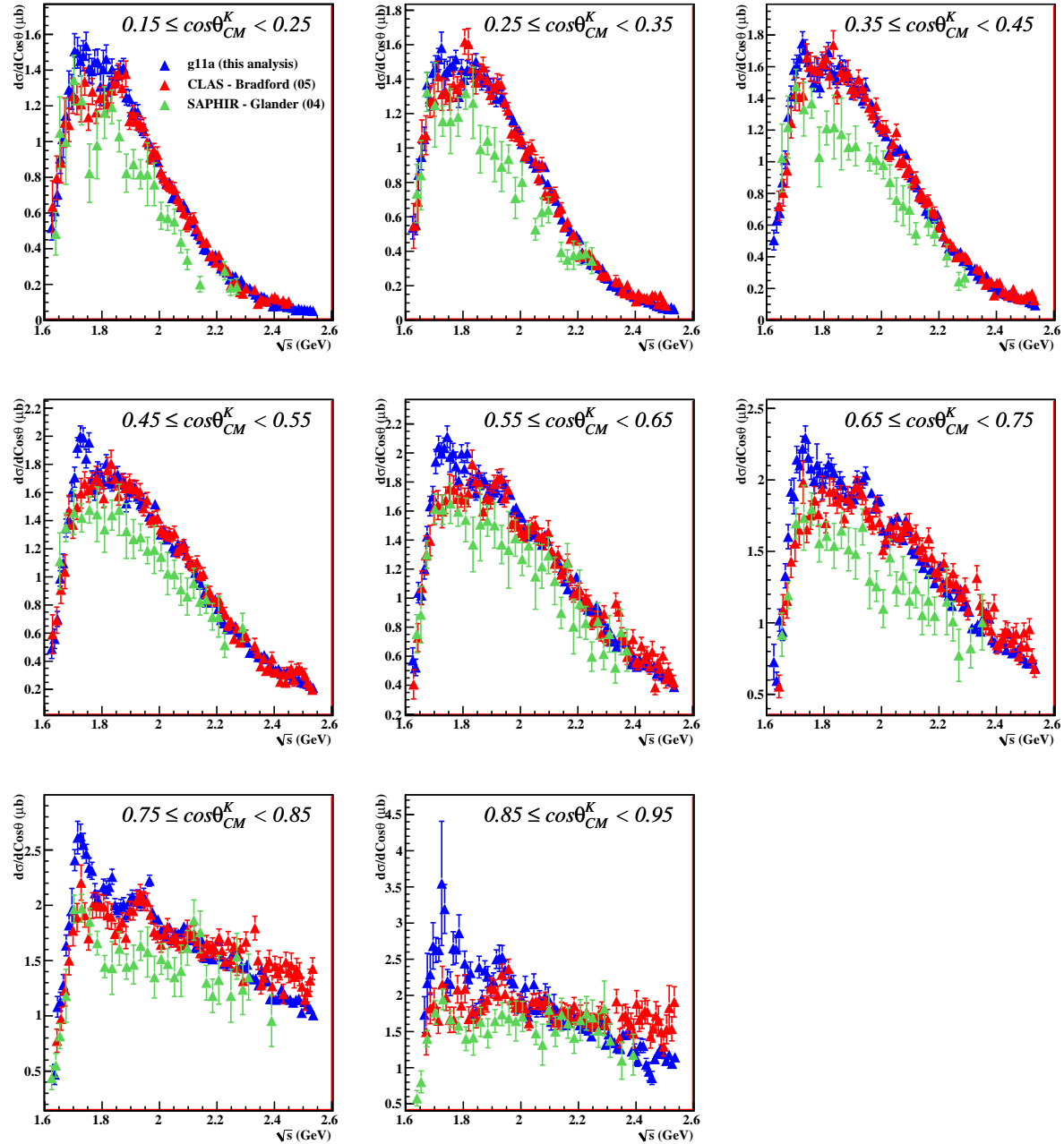
Figure 7.25: Comparison of d\sigma/d\cos\theta_{CM}^K measurements: SAPHIR 2004, CLAS g1c , g11a . The plots above show differential cross section measurements from the CLAS g1c (red), SAPHIR 2004 (green), and this analysis (blue) versus center-of-mass energy in bins of production angle.
