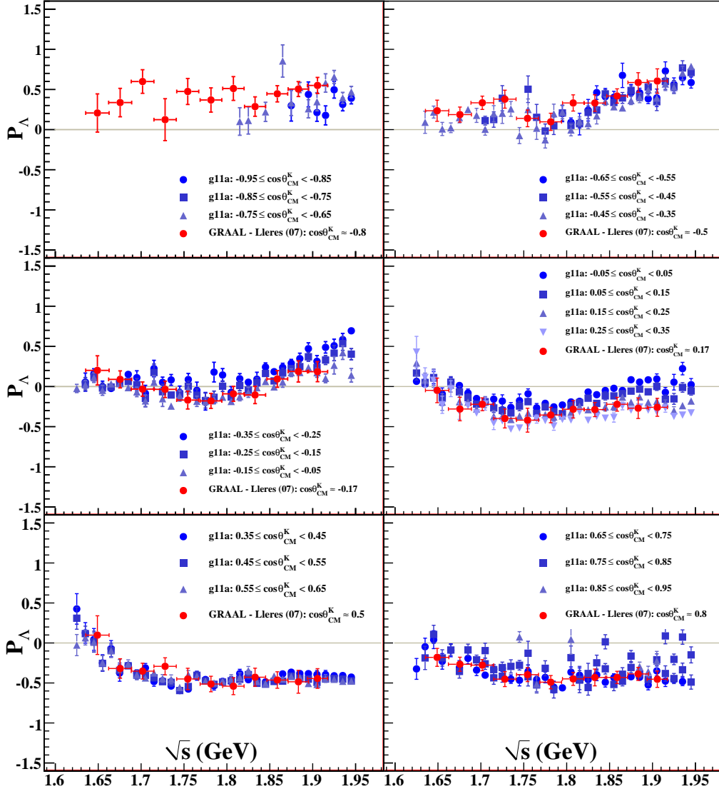
Figure 7.30: The plots above show \Lambda recoil polarization measurements from this analysis (blue shades) and the 2007 GRAAL measurements (red) versus center-of-mass energy in bins of production angle. \cos\theta_{CM}^K ranges for each result are indicated on each plot. Binning in production angle for the GRAAL results is \approx 20^\circ . All error bars reflect statistical uncertainties only.
