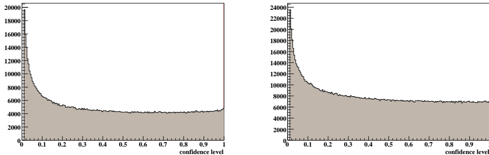
Figure 5.1: Shown above are confidence level distributions from a kinematic fit of \gamma p \rightarrow K^+ p \pi^- Monte Carlo events to the (a) \gamma p \rightarrow K^+ p \pi^- and (b) \gamma p \rightarrow K^+ p (\pi^-) hypotheses. Resolution for these events is the product of GPP smearing of timing signals and the empirical smearing algorithm for tracking signals.
