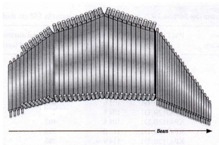
Figure 3.14: Diagram of the CLAS time-of-flight scintillators. Shown is one sector (one sixth of CLAS) of the TOF scintillator shell. Scintillator bars are instrumented with PMTs are each end. Image source: [52].
