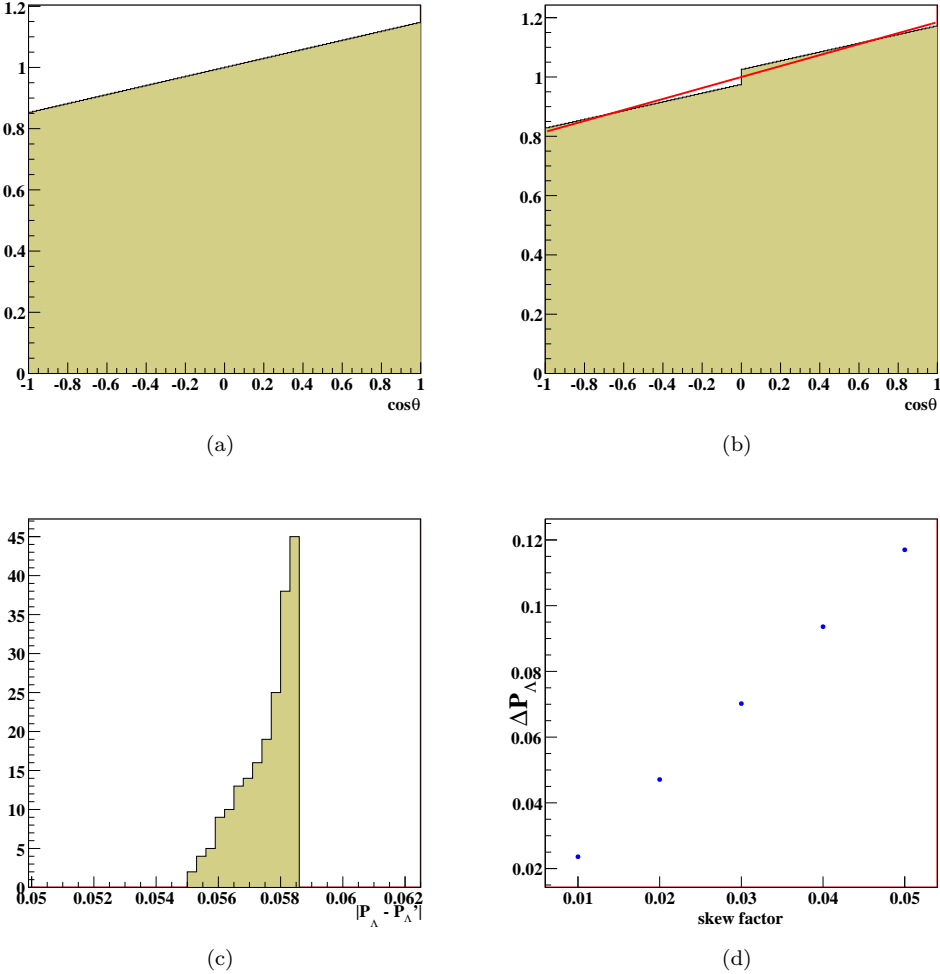
Figure 7.12: Plots showing steps in our estimation of acceptance uncertainty effect on P_\Lambda . Plot (a) shows an ideal \cos\theta distribution with slope P_\Lambda = 0.4 . Plot (b) shows the same distribution distorted by an uncertainty of 2.5%. Plot (c) shows the |P_\Lambda - P'_\Lambda| distribution as described in the text. Plot (d) shows the maximum difference in recoil polarizations, \Delta P_\Lambda , v. distribution skew factor (see text).
