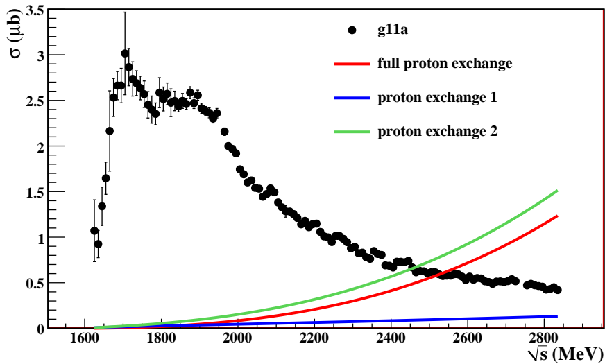
Figure 9.4: Shown above are intensities of the s -channel proton-exchange amplitudes with g_{K\Lambda N} = 9.0 . At low \sqrt{s} , the contribution to the cross section is negligible. At high \sqrt{s} , the contribution is roughly double the total cross section.
