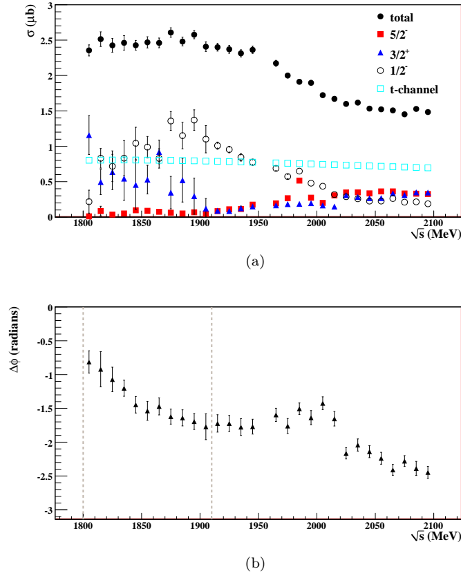
Figure 9.18: Intensities and phase differences from fit with 5/2^-, 3/2^+, 1/2^- waves: 1.80 \text{ GeV} \leq \sqrt{s} < 2.1 \text{ GeV} . Plot (a) shows the intensities from each wave in the fit. Plot (b) shows the phase difference between the 3/2^+ and 1/2^- waves. The vertical dashed lines show the region of overlap between 3/2^+ and 1/2^- intensities.
