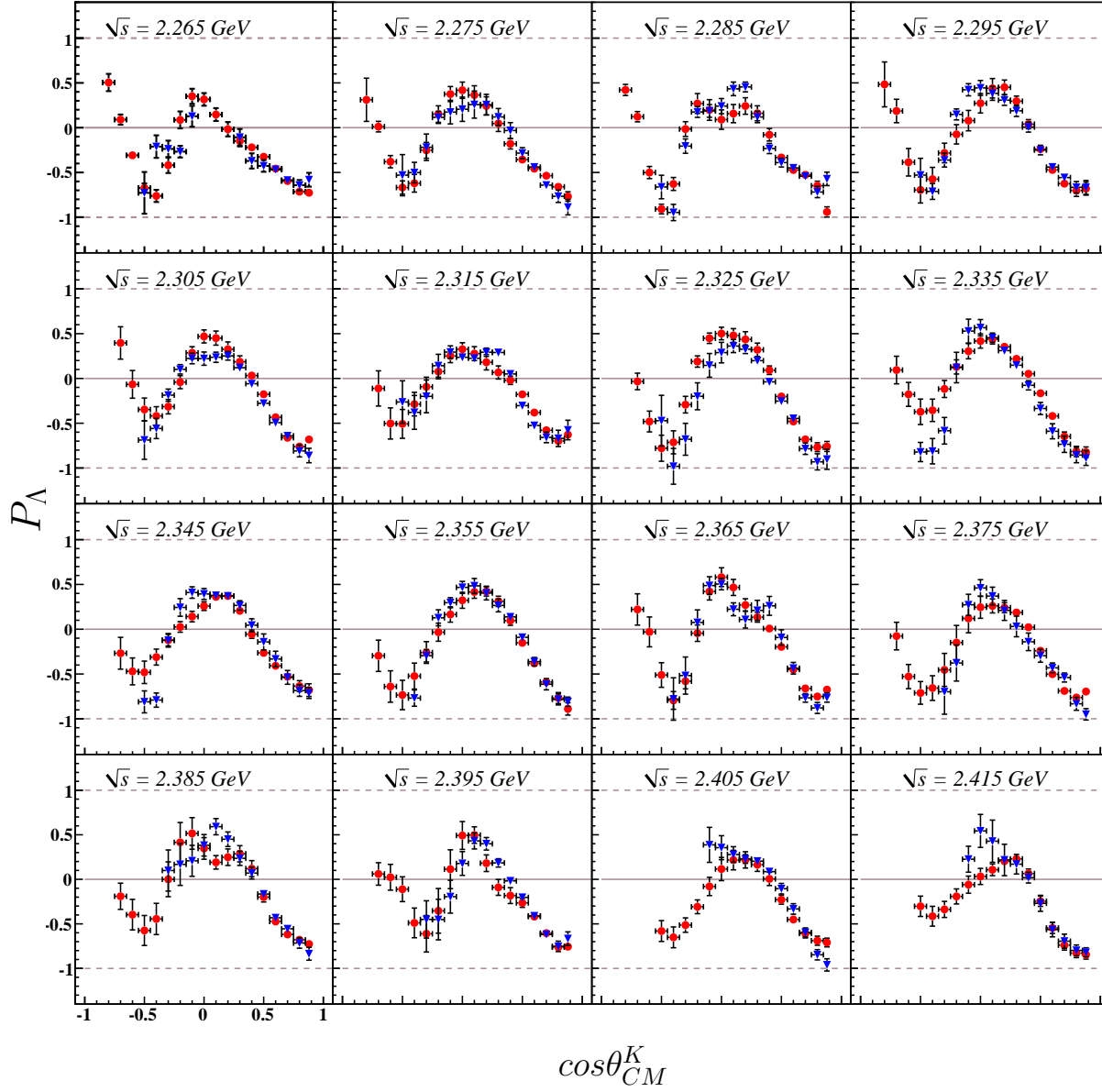
Figure 7.17: P_\Lambda v. \cos\theta_{CM}^K : \Lambda recoil polarization results v. \cos\theta_{CM}^{K^+} for the energy range 2.26 \text{ GeV} \leq \sqrt{s} < 2.42 \text{ GeV} . Results from the three-track analysis are shown in blue (triangles), those of the two-track analysis in red (circles). Uncertainties displayed are estimated from the scatter of results (see text).
