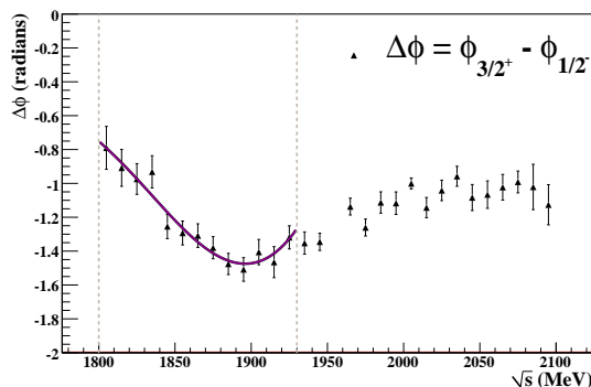
Figure 9.16: Shown above are the phase differences \Delta\phi = \phi_{\frac{3}{2}^+} - \phi_{\frac{1}{2}^-} from fits with \frac{3}{2}^+ and \frac{1}{2}^- s -channel waves and the non-resonant model. Vertical dashed lines indicate the \sqrt{s} range over which both waves show appreciable intensity. The magenta curve shows a fit of a theoretical Breit-Wigner phase difference.
