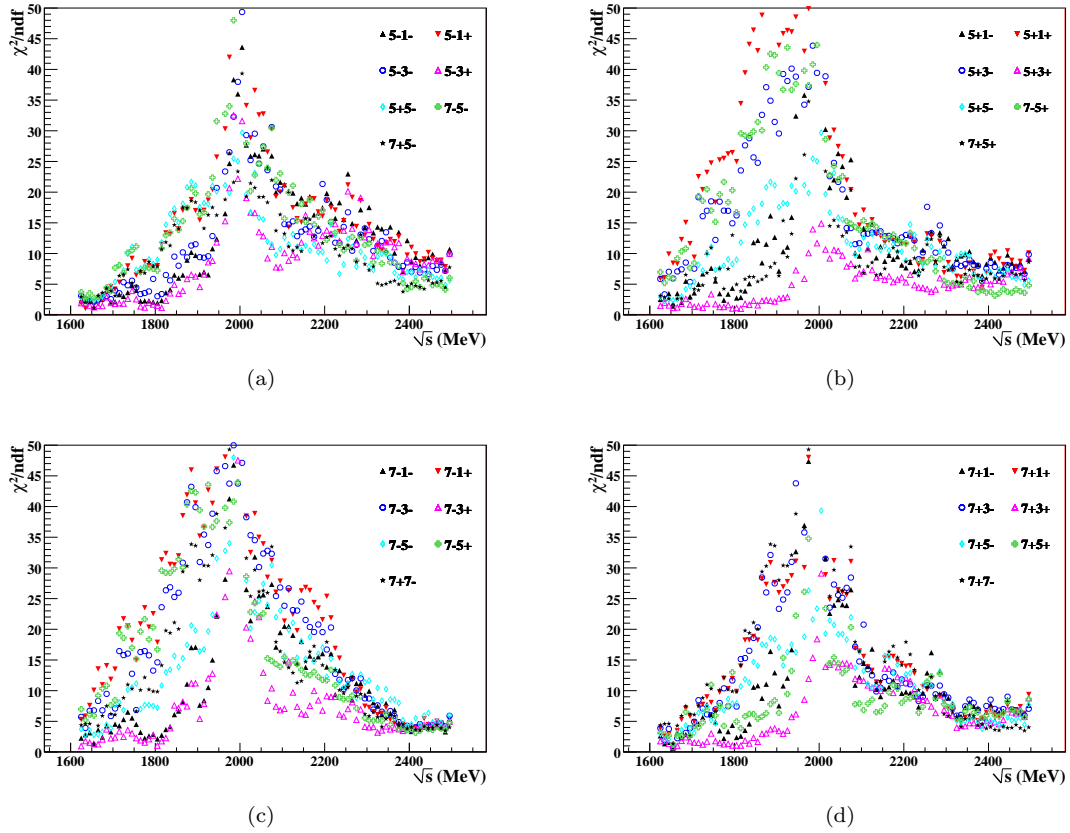
Figure 9.7: Shown above are the \chi^2/ndf in each \sqrt{s} bin for each two-wave scan. Each plot shows all fits involving a certain partial wave. Plots (a), (b), (c), and (d) show all fits that include the \frac{5}{2}^- , \frac{5}{2}^+ , \frac{7}{2}^- , and \frac{7}{2}^+ waves, respectively.
