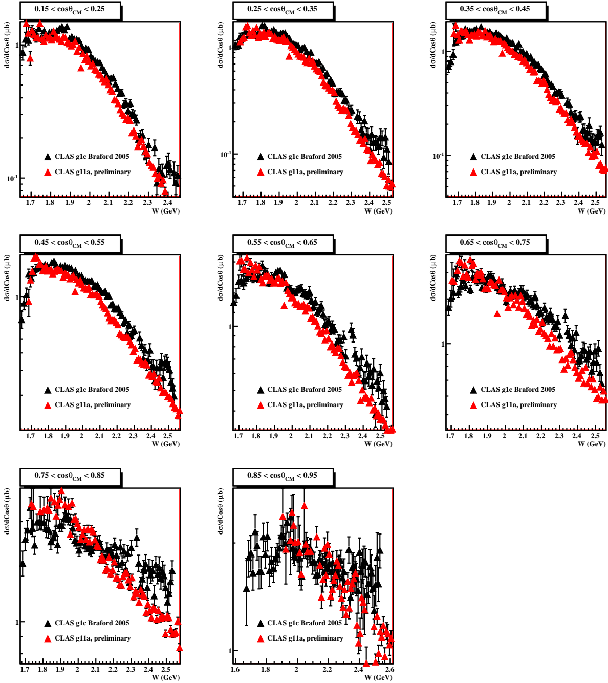
Figure 8.1: Comparison of g_{1c} and preliminary g_{11a} \frac{d\sigma}{d\cos\theta} for forward K^+ angles. \frac{d\sigma}{d\cos\theta} is shown above in bins of \cos\theta_{CM}^K versus \sqrt{s} . The preliminary g_{11a} result is systematically lower than the g_{1c} result in most angles for most values of \sqrt{s} . In the very forward direction, the g_{11a} d\sigma decreases more strongly with \sqrt{s} than the g_{1c} result.
