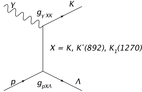
Figure 9.1: The diagram shown represents t -channel exchange of particle type X = K, K^*(892), K_1(1270) . The amplitudes could be parametrized by individual coupling factors, g , for each vertex. Each process considered in this analysis, however, has at least one experimentally undetermined vertex (see text). (Image produced by [76].)
