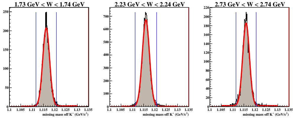
Figure 4.12: Shown above are missing mass of K^+ distributions after all cuts have been applied in several \sqrt{s} bins. Fits to a Gaussian and linear background (shown in red) yield a mean and width for each distribution. The \pm 2.5\sigma cut boundaries are shown in blue.
