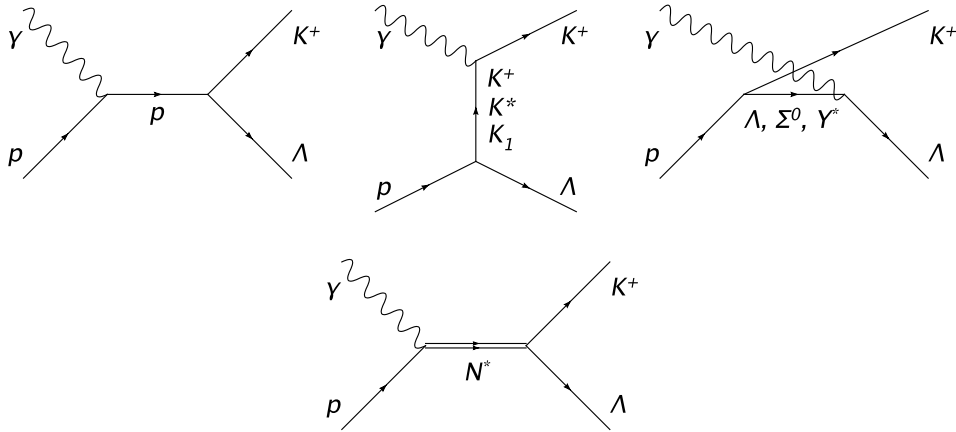
Figure 2.10: Shown above are the Feynman diagrams typical of isobar models (for example [24] or [25]). The top row shows (from left to right) the non-resonant s -, t -, and u -channel diagrams. The diagram at bottom shows s -channel production through an excited nucleon state.
