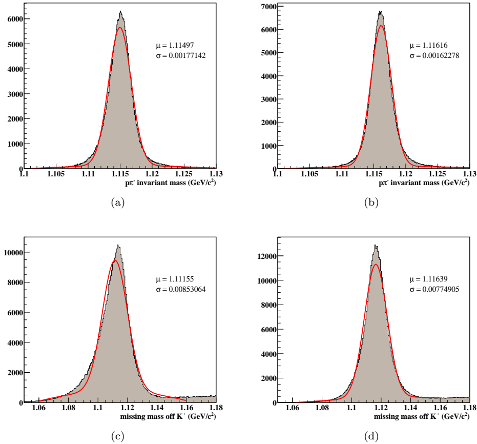
Figure 4.2: Plots showing the effects of energy-loss and momentum corrections on missing mass off K^+ and invariant mass of p\pi^- system. Histograms (a) and (b) show the p\pi^- invariant mass before and after energy and momentum corrections, respectively. Mean ( \mu ) and variance ( \sigma ) of the distributions are from fits (shown in red) to Gaussian and 2^{nd} -order polynomial background. The difference is minimal due to the small break-up momentum of the \Lambda . Histograms (c) and (d) show the missing mass off K^+ before and after corrections, respectively. Fitting of the distributions is performed as in (a) and (b). Here, the effect of the corrections is noticeable. The fit demonstrates how the non-Gaussian shape of the distribution is tamed by the corrections.
