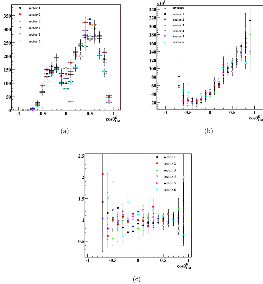
Figure 5.6: The plots above show steps in the acceptance uncertainty calculation for the \sqrt{s} = 2.005 GeV bin. Plot (a) shows the sector-dependent data yields, whereas plot (b) shows these yields after acceptance correction along with the mean acceptance-corrected yield. Plot (c) shows the ratios of each sector's acceptance corrected yield to the mean.
