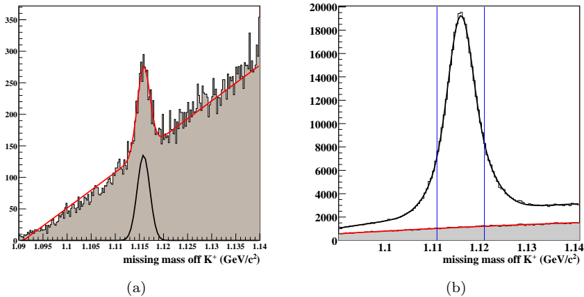
Figure 4.10: Plot (a) shows the missing mass off K^+ distribution for events removed by PID cuts in the three-track analysis. The signal peak is apparent and an estimate is made by fitting with a Gaussian and linear functions. Plot (b) shows the distribution for all two-track events in runs 43810-43819 (unshaded histogram) and a fit to a double Gaussian and quadratic background in black. The shaded histogram shows the missing mass off K^+ for events removed by the PID cuts. No signal peak is apparent. Shown in red is a fit with a quadratic function. The blue lines indicate the range considered for the application the Feldman-Cousins method (see text).
