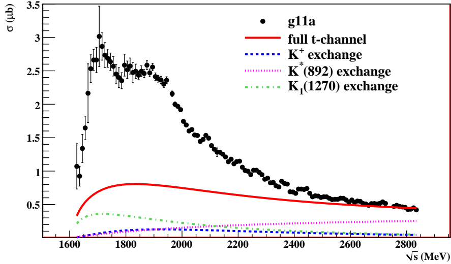
Figure 9.3: Shown above are comparisons of the total cross section (black) and projections of the full non-resonant model (red) and its component production mechanisms.
