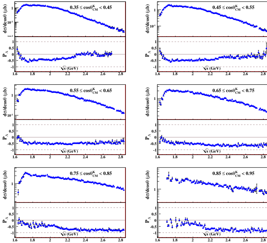
Figure 7.23: Weighted mean d\sigma/d\cos\theta_{CM}^K and P_\Lambda results v. \sqrt{s} for forward production angles. Differential cross sections are plotted above recoil polarizations from the indicated \cos\theta_{CM}^K bin. Errors displayed are statistical.
