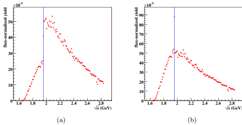
Figure 5.8: Shown above are the flux-normalized yields v. \sqrt{s} before (a) and after (b) the untriggered T-counter correction. The correction restores rough continuity to the trend of the yields versus \sqrt{s} . The blue line in each plot marks the energy of the trigger cut-off, \sqrt{s} \approx 1.955 GeV.
