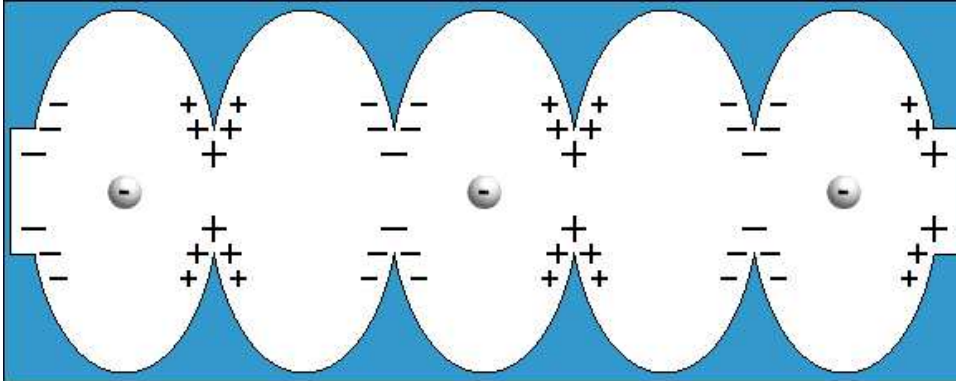
Figure 3.4: A schematic diagram of the superconducting RF cavity. Accelerating fields are established by charge accumulated on the inner tangs of the RF cavity (shown in diagram). These excess charges are the result of standing RF waves in the cavity. The phase of the waves follows the position of the electron bunch in the cavity, ensuring a positive force on the electrons at all times. Image source: [38].
