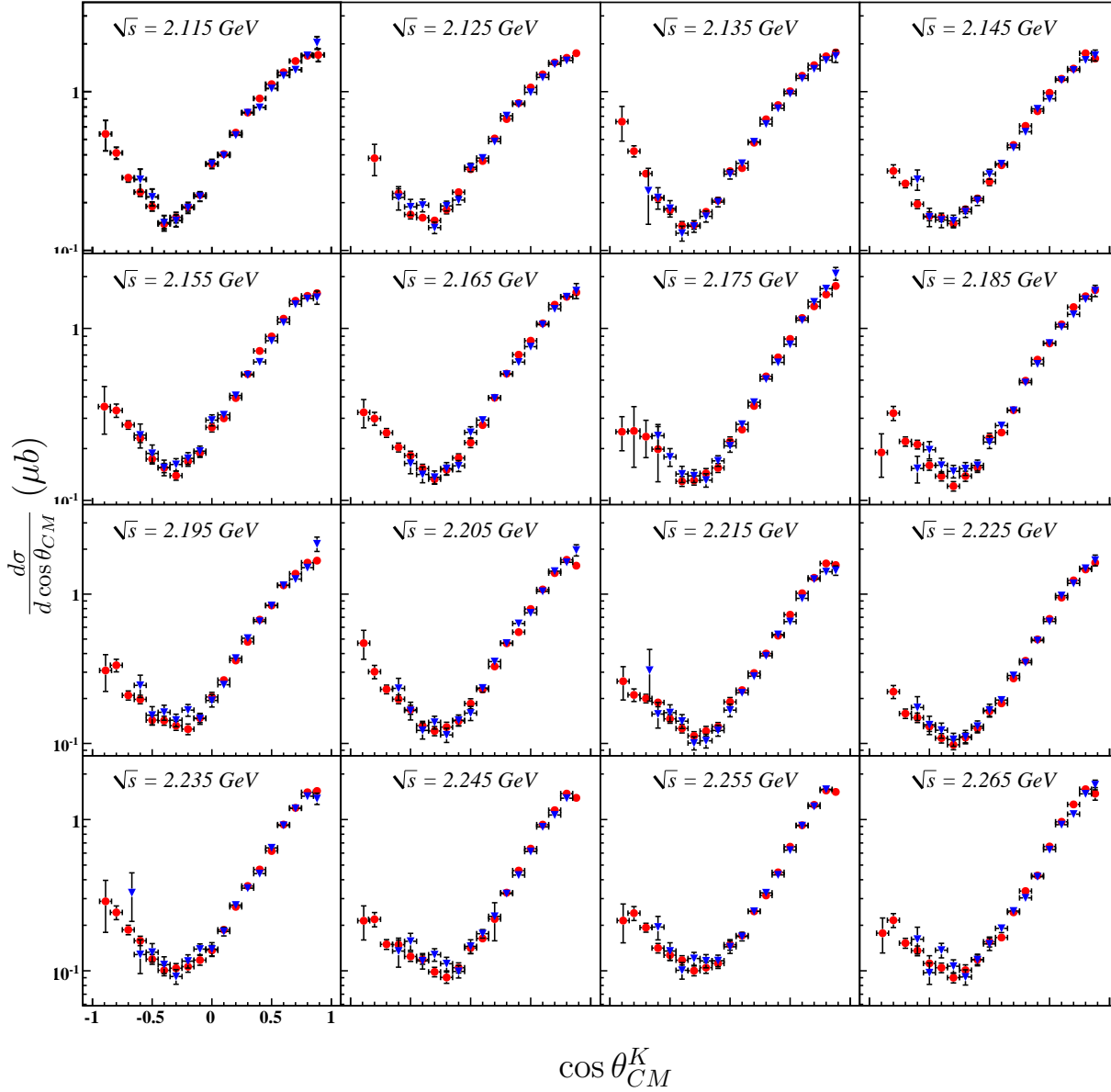
Figure 7.6: d\sigma/d\cos\theta_{CM}^K ( \mu b ) v. \cos\theta_{CM}^K : Differential cross section results for the energy range 2.11 \text{ GeV} \leq \sqrt{s} < 2.27 \text{ GeV} . Results from the three-track analysis are shown in blue (triangles), those of the two-track analysis in red (circles). All plots have the same \cos\theta_{CM}^K -axis range and vertical axis ranges are the same for the four plots in each row. Vertical axes are logarithmic scale.
