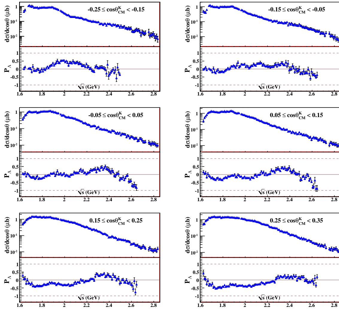
Figure 7.22: Weighted mean d\sigma/d\cos\theta_{CM}^K and P_{\Lambda} results v. \sqrt{s} for middle production angles. Differential cross sections are plotted above recoil polarizations from the indicated \cos\theta_{CM}^K bin. Errors displayed are statistical.
