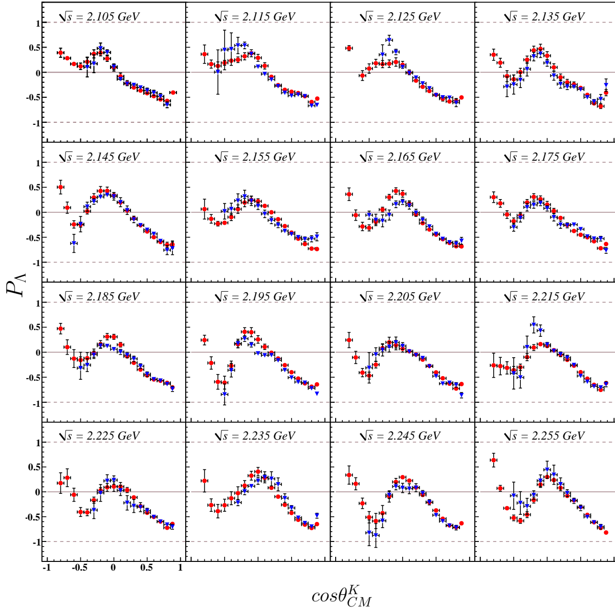
Figure 7.16: P_\Lambda v. \cos\theta_{CM}^K : \Lambda recoil polarization results v. \cos\theta_{CM}^{K^+} for the energy range 2.10 \text{ GeV} \leq \sqrt{s} < 2.26 \text{ GeV} . Results from the three-track analysis are shown in blue (triangles), those of the two-track analysis in red (circles). Uncertainties displayed are estimated from the scatter of results (see text).
