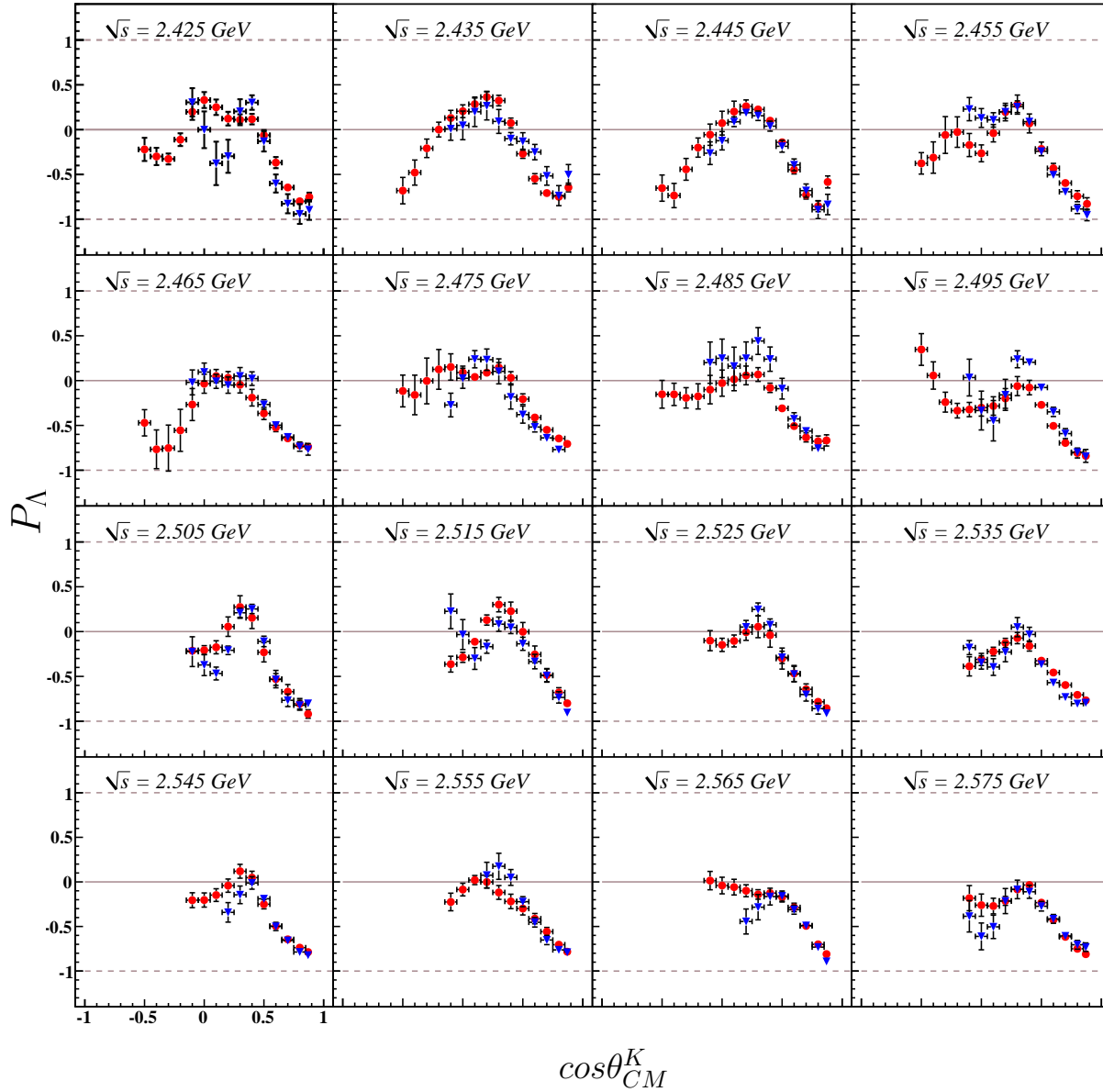
Figure 7.18: P_\Lambda v. \cos\theta_{CM}^{K^+} : \Lambda recoil polarization results v. \cos\theta_{CM}^{K^+} for the energy range 2.42 \text{ GeV} \leq \sqrt{s} < 2.58 \text{ GeV} . Results from the three-track analysis are shown in blue (triangles), those of the two-track analysis in red (circles). Uncertainties displayed are estimated from the scatter of results (see text).
