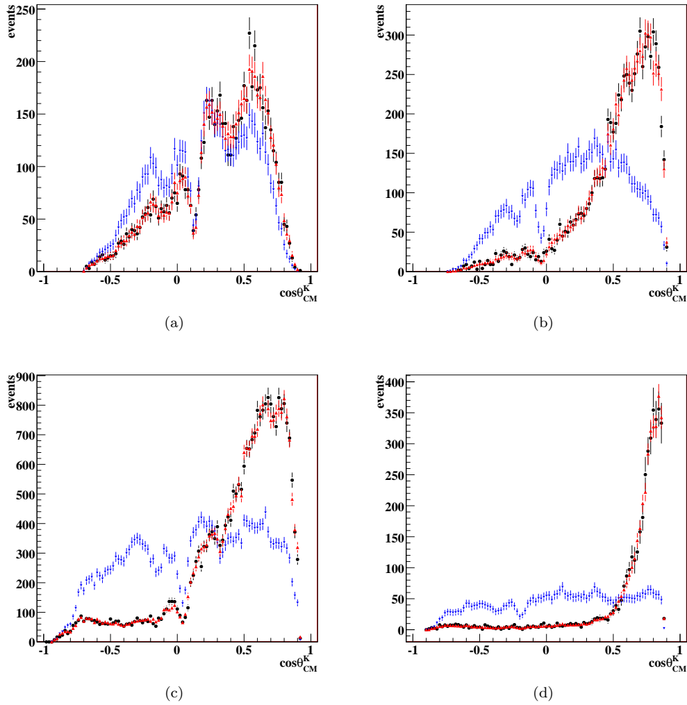
Figure 7.1: Shown above are \cos\theta_{CM}^K yields for the data (black) and Monte Carlo before (blue) and after (red) fit weighting. The top plots show the distributions for the three-track topology in the (a) \sqrt{s} = 1.905 GeV and (b) \sqrt{s} = 2.305 GeV bins. The bottom plots represent the two-track topology distributions for the (c) \sqrt{s} = 2.105 GeV and (d) \sqrt{s} = 2.705 GeV bins. Overall agreement between data and weighted accepted MC is very good.
