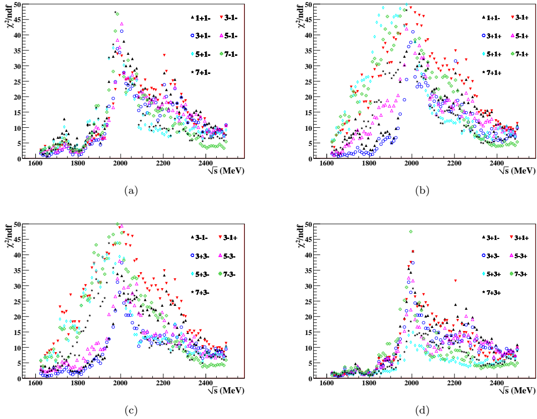
Figure 9.6: Shown above are the \chi^2/ndf in each \sqrt{s} bin for each two-wave scan. Each plot shows all fits involving a certain partial wave. Plots (a), (b), (c), and (d) show all fits that include the \frac{1}{2}^- , \frac{1}{2}^+ , \frac{3}{2}^- , and \frac{3}{2}^+ waves, respectively.
