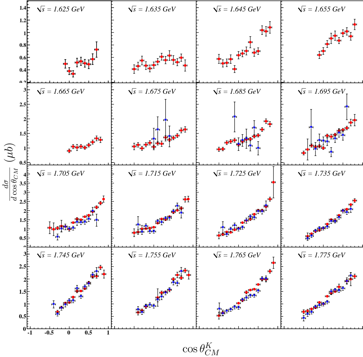
Figure 7.3: d\sigma/d\cos\theta_{CM}^K ( \mu\text{b} ) v. \cos\theta_{CM}^K : Differential cross section results for the energy range 1.62\text{ GeV} \leq \sqrt{s} < 1.78\text{ GeV} . Results from the three-track analysis are shown in blue (triangles), those of the two-track analysis in red (circles). All plots have the same \cos\theta_{CM}^K -axis range and vertical axis ranges are the same for the four plots in each row.
