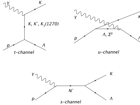
Figure 6.1: Shown above are diagrams characterizing the \gamma p \rightarrow K^+ \Lambda production mechanisms considered in this analysis. (Image produced by [76].)
