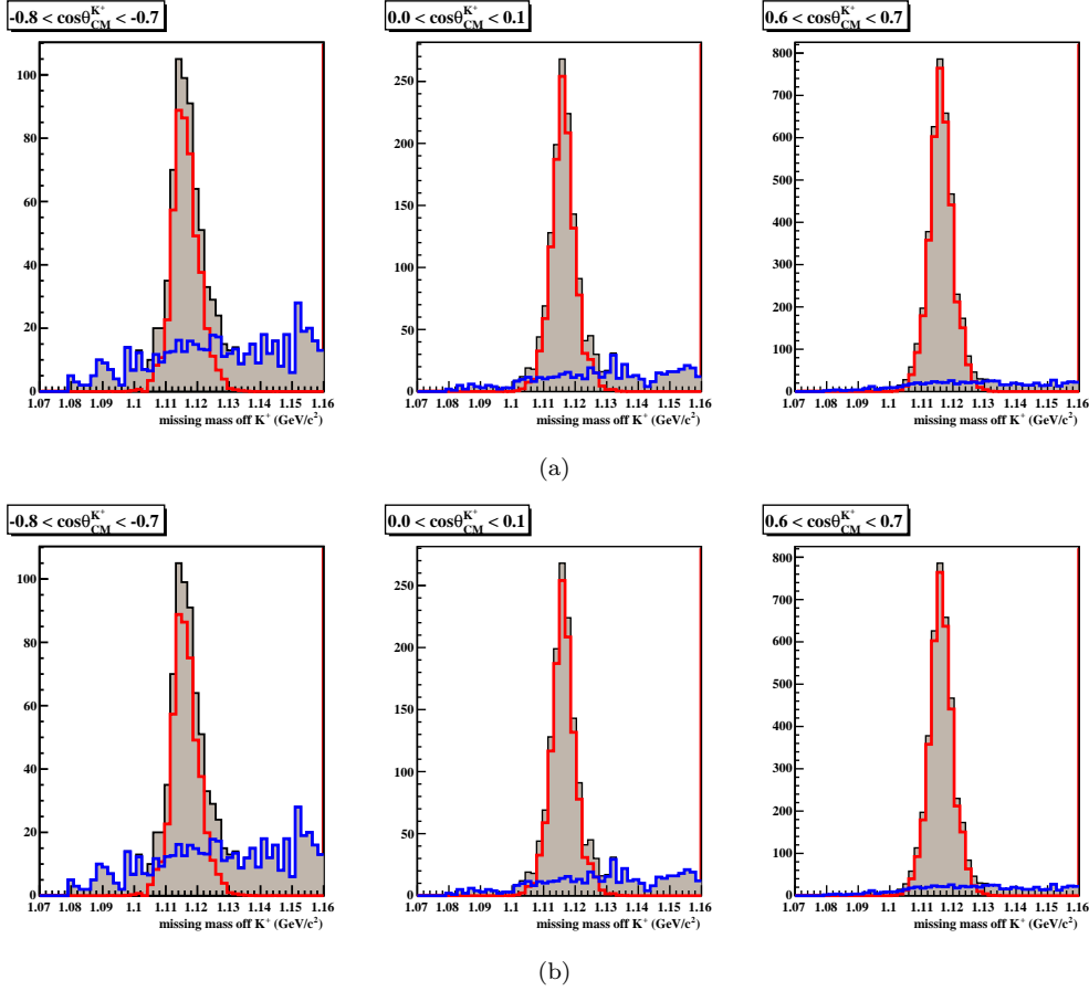
Figure 4.13: Shown above are the effects of the background subtraction method in three \cos\theta_{CM}^{K^+} bins in (a) \sqrt{s} = 2.005 GeV and (b) \sqrt{s} = 2.605 GeV bins for the g11a pK^+ topology. The full missing mass off K^+ distributions are shown as shaded histograms. Signal is shown in red and background is shown in blue.
