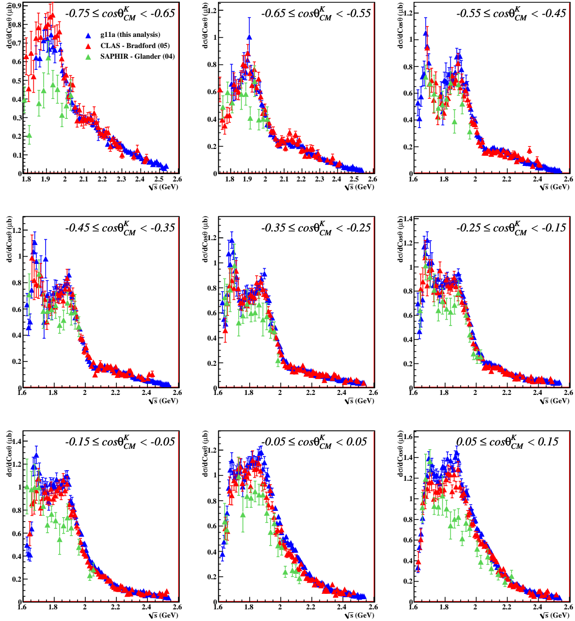
Figure 7.24: Comparison of d\sigma/d\cos\theta_{CM}^K measurements: SAPHIR 2004, CLAS g1c , g11a . The plots above show differential cross section measurements from the CLAS g1c (red), SAPHIR 2004 (green), and this analysis (blue) versus center-of-mass energy in bins of production angle.
