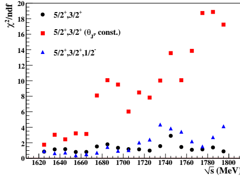
Figure 9.11: The plot above shows \chi^2/ndf for each of the indicated fit schemes. The fit with \frac{5}{2}^+ and \frac{3}{2}^+ waves with multipole couplings free (black circles) produces a fair \chi^2/ndf . Constraining the multipole parameter for both of these waves (red squares) reduces their ability to describe the data. Also shown is the fit with \frac{5}{2}^+ , \frac{3}{2}^+ , and \frac{1}{2}^- waves with \theta_{\frac{5}{2}^+} and \theta_{\frac{3}{2}^+} constrained.
