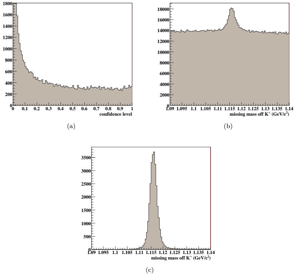
Figure 4.3: The above plots show the results of a kinematic fit to \gamma p \rightarrow K^+ p \pi^- for events in run 43815. Plot (a) shows the confidence levels from all events. The confidence level distribution is fairly flat above 0.4. Plot (b) show the missing mass off K^+ for all events in the run. There is a large amount of background, however, the \Lambda peak can be seen. Plot (c) shows the missing mass off K^+ distribution for events passing the 1% confidence level cut. The effect of the cut is dramatic.
