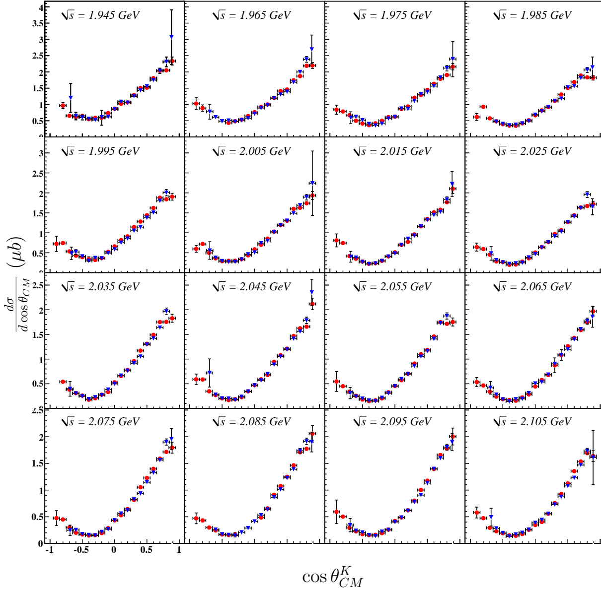
Figure 7.5: d\sigma/d\cos\theta_{CM}^K ( \mu\text{b} ) v. \cos\theta_{CM}^K : Differential cross section results for the energy range 1.94\text{ GeV} \leq \sqrt{s} < 2.11\text{ GeV} . Results from the three-track analysis are shown in blue (triangles), those of the two-track analysis in red (circles). All plots have the same \cos\theta_{CM}^K -axis range and vertical axis ranges are the same for the four plots in each row.
