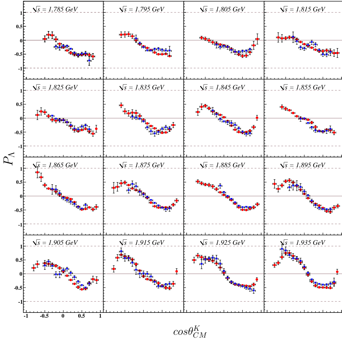
Figure 7.14: P_{\Lambda} v. \cos\theta_{CM}^K : \Lambda recoil polarization results v. \cos\theta_{CM}^{K^+} for the energy range 1.78 \text{ GeV} \leq \sqrt{s} < 1.94 \text{ GeV} . Results from the three-track analysis are shown in blue (triangles), those of the two-track analysis in red (circles). Uncertainties displayed are estimated from the scatter of results (see text).
