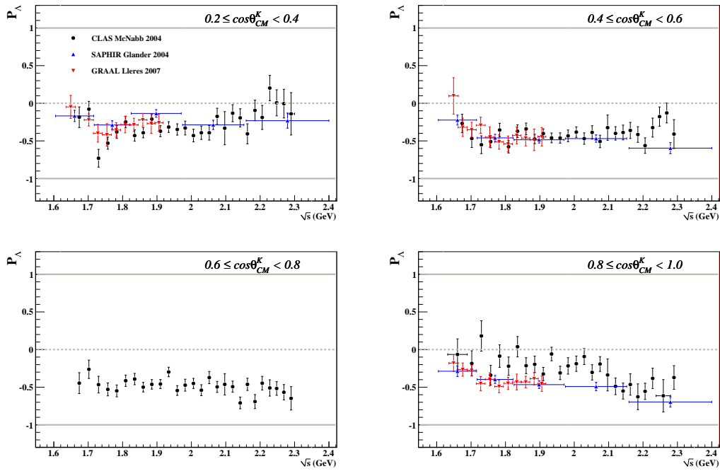
Figure 2.7: Shown above are P_\Lambda results from previous analyses of \gamma p \rightarrow K^+ \Lambda at forward production angles. Each plot represents data in the 0.2-unit-wide \cos \theta_{CM}^K range indicated. Marker convention is given at top left and is the same for all plots.
