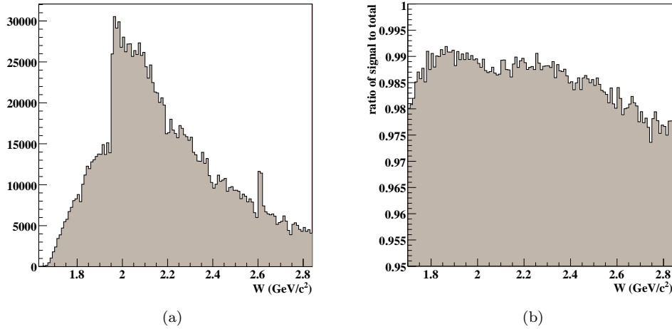
Figure 4.4: Plots above show (a) yields and (b) ratio of signal to total yield from the three-track skim of \gamma p \rightarrow K^+ p \pi^- from g11a . Signal was calculated by fitting missing mass off K^+ distribution in each 10 MeV-wide \sqrt{s} bin to a Gaussian and linear background. Signal and background functions were then integrated over the range \mu \pm 3\sigma , where \mu and \sigma are the mean and width from the fit in each bin. The skim is remarkably clean, with signal making up \approx 98\% of the yield in each bin. Ratios are not shown for bins with \sqrt{s} < 1.7 GeV because low statistics limited reliable fits.
