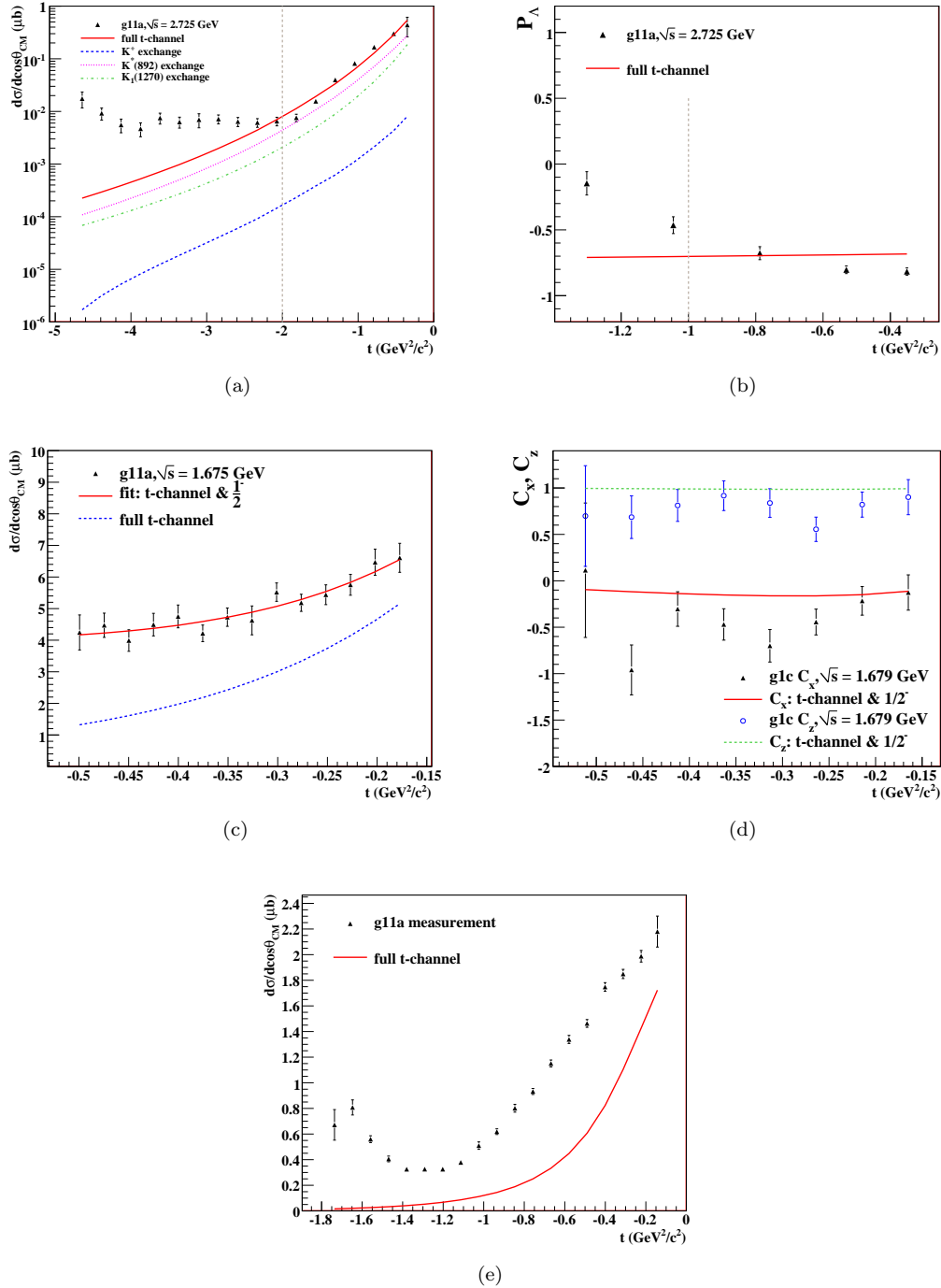
Figure 9.2: Results of the non-resonant model fits. Plot (a) shows the differential cross section data (black) and fit (solid red) for the \sqrt{s} = 2.725 GeV bin. The strengths of the individual t -channel diagrams are shown as well. Points included in the fit are those to the right of the dashed vertical line ( t > -2.0 ). Plot (b) shows the P_\Lambda data (black) and fit result (red) in the \sqrt{s} = 2.725 GeV bin. Plot (c) shows the differential cross section data (black), total fit (red), and t -channel contribution in the \sqrt{s} = 1.675 GeV bin. Plot (d) shows the fit to C_x and C_z in the \sqrt{s} = 1.675 GeV bin. Differential cross section data (black) and t -channel contributions (red) projected into the \sqrt{s} = 2.005 GeV bin are shown in Plot (e).
