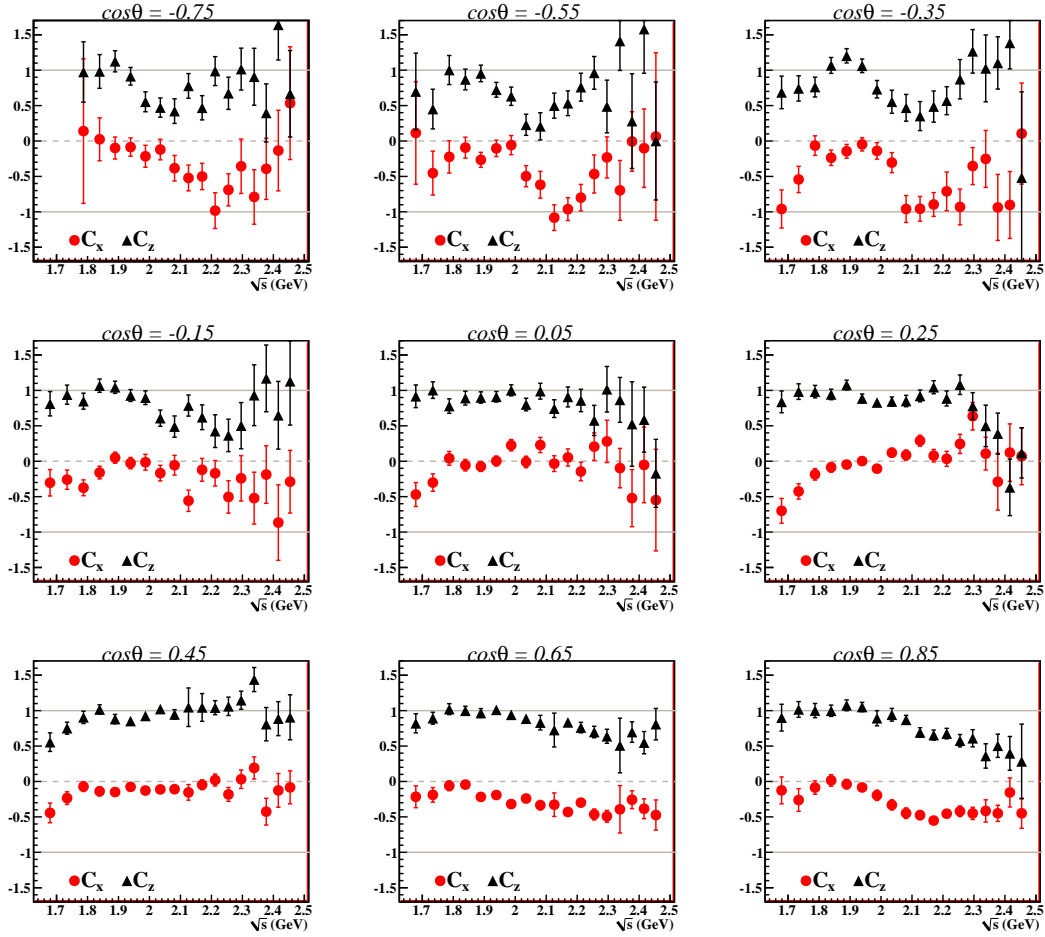
Figure 2.8: The plots above show the beam-recoil polarization transfer results published by the CLAS Collaboration in 2005 [84]. Each plot shows results at a fixed \cos\theta_{CM}^K value (indicated above each plot) versus \sqrt{s} . C_x is shown in red circles and C_z is shown in black triangles.
