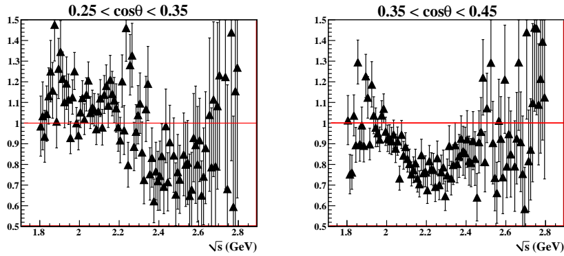
Figure 8.7: The plots above show the ratios of d\sigma/d\cos\theta_{CM}^K values from sector 5 to those from sectors 1, 2, 3, 4, and 6 (combined). Shown are the 0.25 \leq \cos\theta_{CM}^K < 0.35 (left) and 0.35 \leq \cos\theta_{CM}^K < 0.45 (right) bins. The dip in the sector 5 cross section is apparent in both angular bins over a significant \sqrt{s} range.
