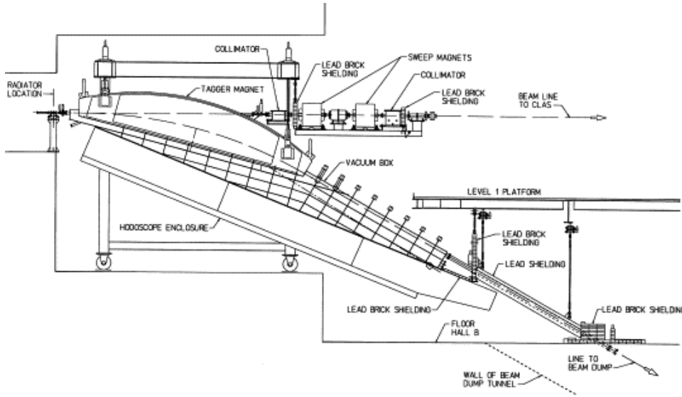
Figure 3.5: A schematic diagram of the Hall B photon tagging system. The Hall B photon tagger allows indirect measurement of photon energy. The energy of a recoil electron is measured by the tagger spectrometer (tagger magnet and hodoscope). The energy of the associated bremsstrahlung photon is then ascertained from energy conservation. The bremsstrahlung beam is then collimated and passed to the CLAS detector. Image source: [42].
