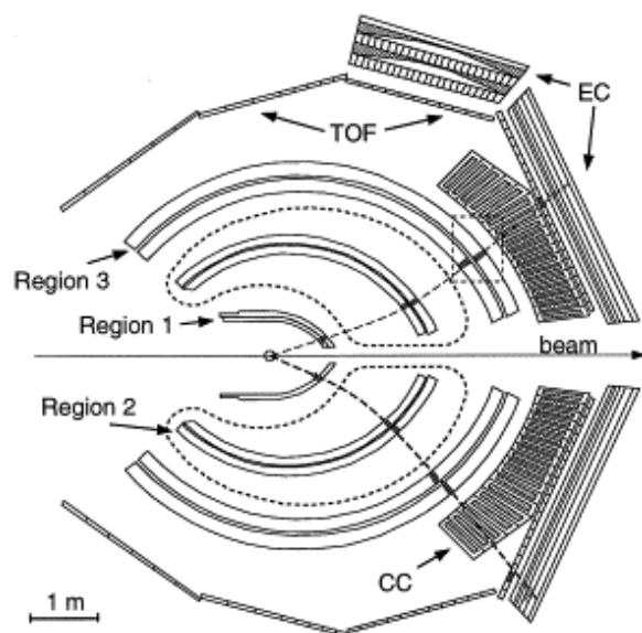
Figure 3.13: Diagram of the CLAS Detector Subsystems (cutaway). This image shows the locations of several detector subsystems inside of CLAS. Toroidal magnet coils are represented by the kidney-shaped dashed lines. The three different drift chamber regions are labeled. Shown are two positively-charged tracks being bent by the magnetic field in the volume between Regions 1 and 3. Image source: [48].
