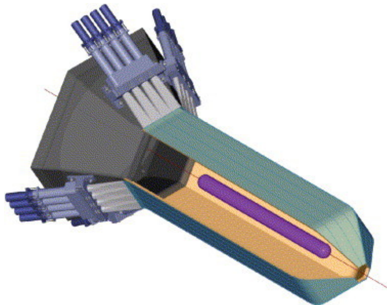
Figure 3.11: A schematic diagram of the CLAS Start Counter. The start counter used for the g11a run period is a six-sector scintillator detector. Each sector is composed of four independently-instrumented scintillator strips. Image source: [46].
