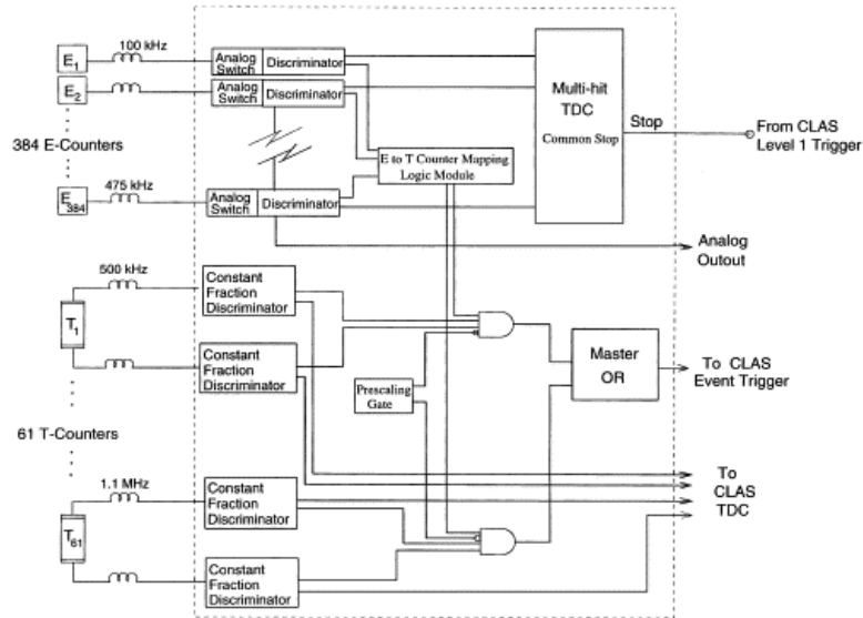
Figure 3.7: A schematic diagram of the Tagger instrumentation logic. Individual T- and E-counters are shown on the left-side of the diagram. T-counter hits are used to set the event trigger. The CLAS Level 1 trigger then provides a common stop to the E-counter TDC array. Image source: [42].
