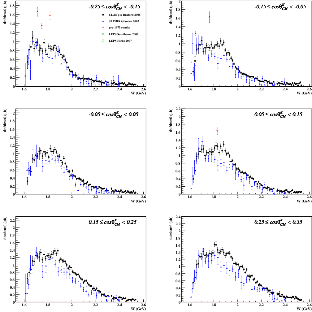
Figure 2.4: Shown above are previous measurements of the \gamma p \rightarrow K^+ \Lambda differential cross section at middle angles. Each plot displays data in a 0.1-unit-wide \cos\theta_{CM} range versus \sqrt{s} . The legend at top left indicates the convention for all plots.
