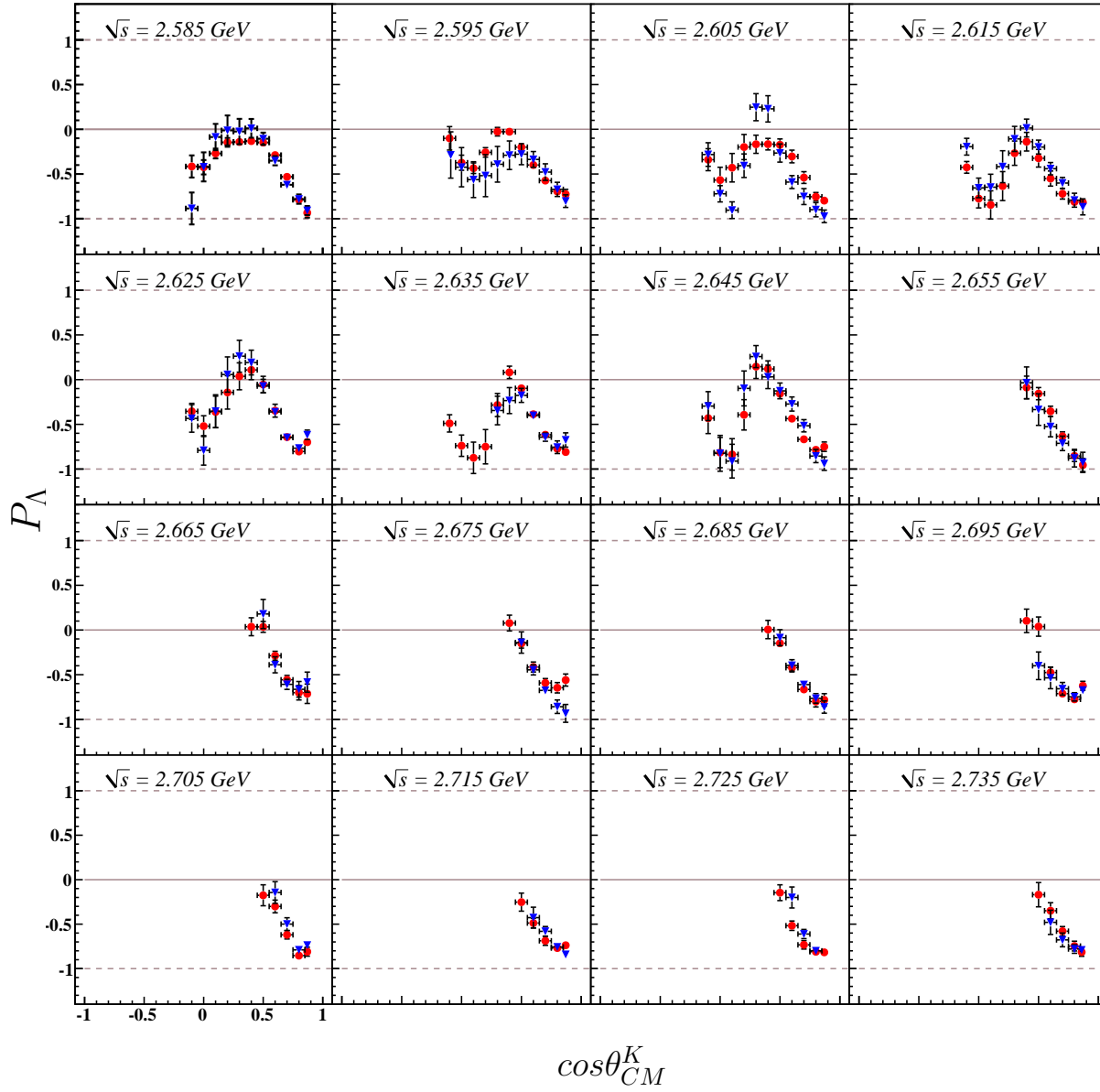
Figure 7.19: P_\Lambda v. \cos\theta_{CM}^K : \Lambda recoil polarization results v. \cos\theta_{CM}^{K^+} for the energy range 2.58 \text{ GeV} \leq \sqrt{s} < 2.74 \text{ GeV} . Results from the three-track analysis are shown in blue (triangles), those of the two-track analysis in red (circles). Uncertainties displayed are estimated from the scatter of results (see text).
