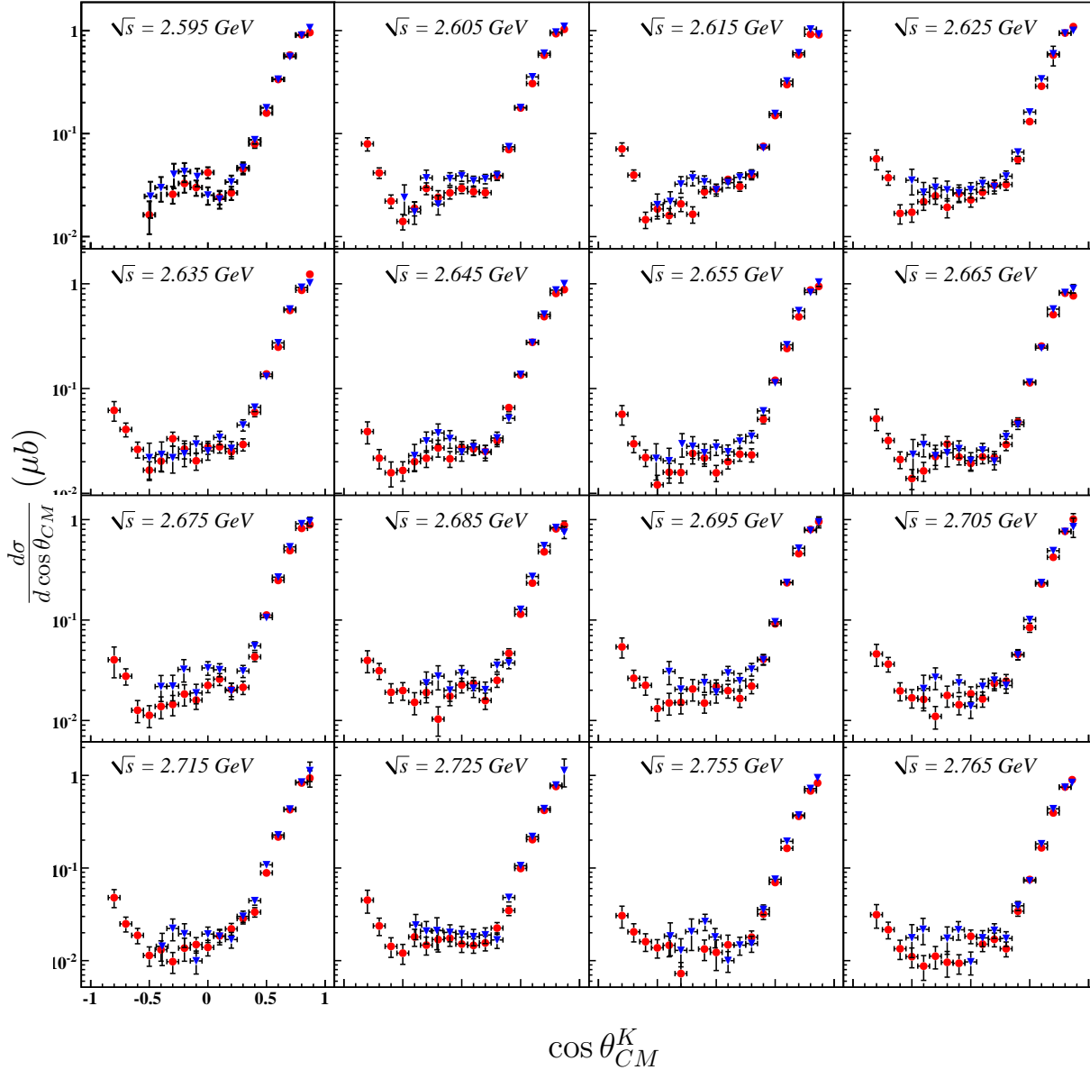
Figure 7.9: d\sigma/d\cos\theta_{CM}^K ( \mu b ) v. \cos\theta_{CM}^K : Differential cross section results for the energy range 2.59\text{ GeV} \leq \sqrt{s} < 2.77\text{ GeV} . Results from the three-track analysis are shown in blue (triangles), those of the two-track analysis in red (circles). All plots have the same \cos\theta_{CM}^K -axis range and vertical axis ranges are the same for the four plots in each row. Vertical axes are logarithmic scale.
