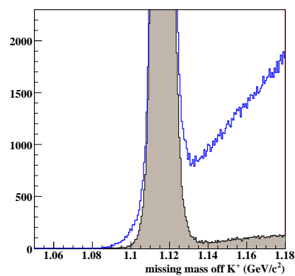
Figure 4.8: The figure above shows the effect of the calculated-mass particle-identification cut on the missing mass off K^+ distribution from the three-track analysis. Missing mass off K^+ for all events is shown in blue. The distribution after the PID cut is shaded.
