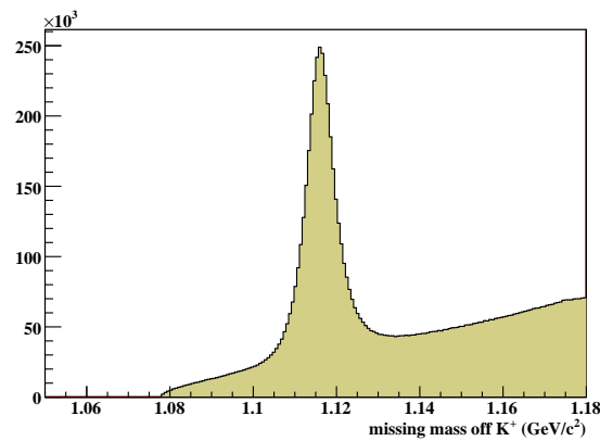
Figure 4.5: Shown above is the missing mass off K^+ distribution for all events in the K^+ p skim of g11a . The less restrictive 1C kinematic fit allows more background to pass the skim than did the 4C fit on the K^+ p \pi^- topology.
