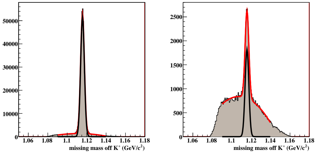
Figure 5.5: Plot (a) above shows the missing mass off K^+ distribution of all Monte Carlo events with \sqrt{s} < 1.66 GeV. Fit to a Gaussian and quadratic background show that there are roughly 3.87 \times 10^5 events in the signal peak. Plot (b) shows the distribution of events cut by particle identification. Fitting reveals 13400 events in this peak, only 3.4% of the total.
