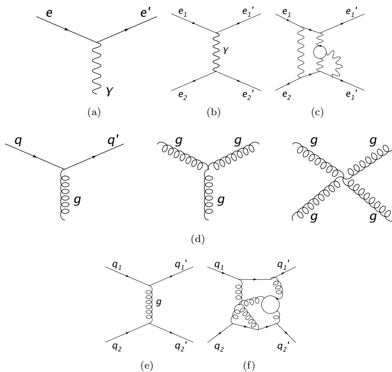
Figure 2.1: Figure (a) shows the possible QED vertex representing the emission or absorption of a photon (wavy line) by the charged particle e (straight line). Figures (b) and (c) both represent contributions to the Coulomb interaction between particles e_1 and e_2 composed of the vertex in (a). The diagrams in (d) are those allowed by QCD: emission or absorption of a gluon by a quark and the three- and four-gluon vertices. Figures (e) and (f) show diagrams representing strong interaction between two quarks.
