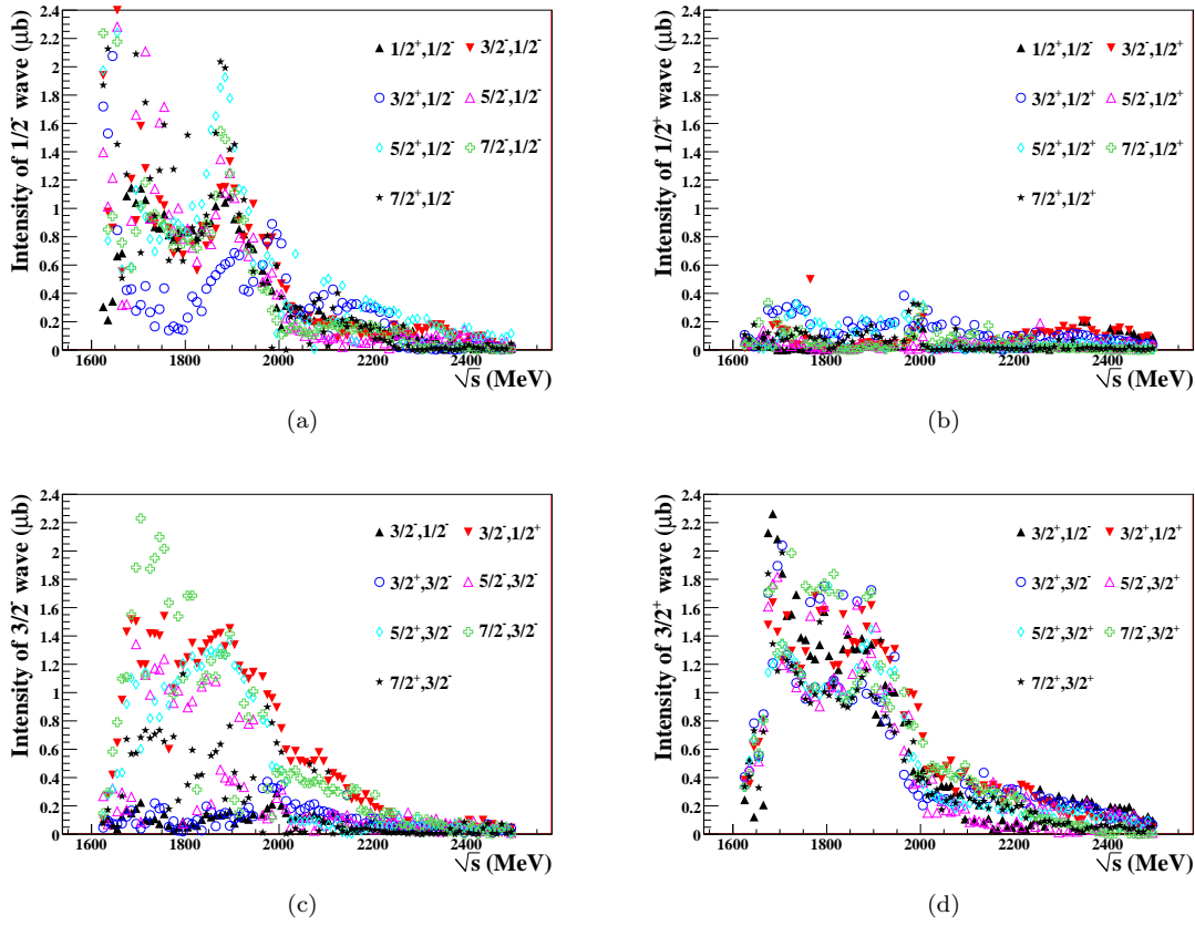
Figure 9.8: Shown above are the intensities of individual s -channel waves when fit with the wave combinations indicated. For example, plot (a) shows the intensity of the \frac{1}{2}^- partial wave when fit with each of the other waves indicated. From this plot, we see that the \frac{1}{2}^- wave has a sizable intensity at \sqrt{s} = 1.9 GeV in all fits, but its intensity is the least when paired with the \frac{3}{2}^+ partial wave. Shown are the J^P = \frac{1}{2}^- (a), \frac{1}{2}^+ (b), \frac{3}{2}^- (c), and \frac{3}{2}^+ (d) partial waves.
