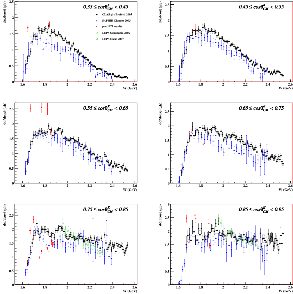
Figure 2.5: Shown above are previous measurements of the \gamma p \rightarrow K^+ \Lambda differential cross section at forward angles. Each plot displays data in a 0.1-unit-wide \cos \theta_{CM} range versus \sqrt{s} . The legend at top left indicates the convention for all plots.
