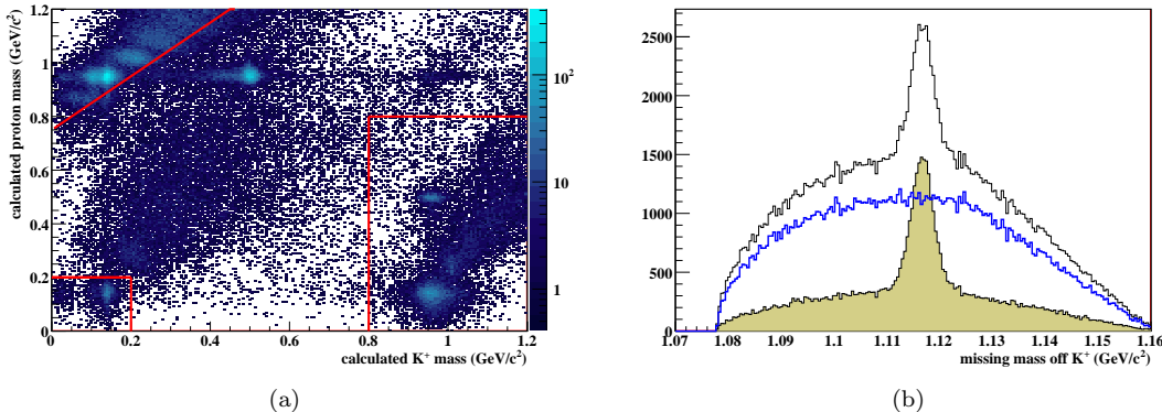
Figure 4.9: Plot (a) shows the calculated mass plane for events in the g11a two-track topology with \sqrt{s} < 1.660 GeV. Cuts are defined in the text and displayed on the plot in red. Plot (b) shows the effect of these cuts on the missing mass off K^+ distribution. The unshaded histogram is filled with all events in the skim (with \sqrt{s} < 1.660 GeV). The blue histogram shows events removed by PID cuts and the shaded histogram shows events that pass the cuts.
