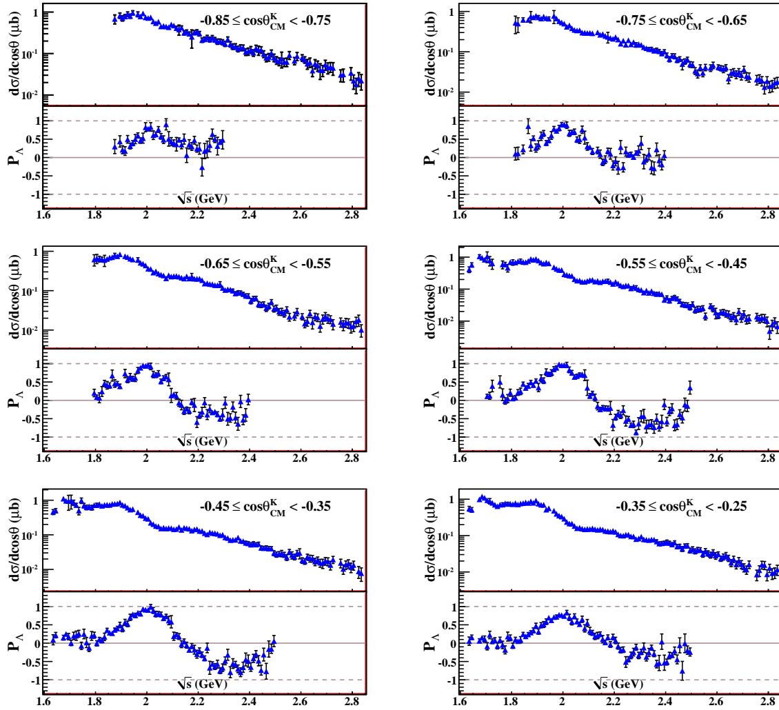
Figure 7.21: Weighted mean d\sigma/d\cos\theta_{CM}^K and P_\Lambda results v. \sqrt{s} for backward production angles. Differential cross sections are plotted above recoil polarizations from the indicated \cos\theta_{CM}^K bin. Errors displayed are statistical.
