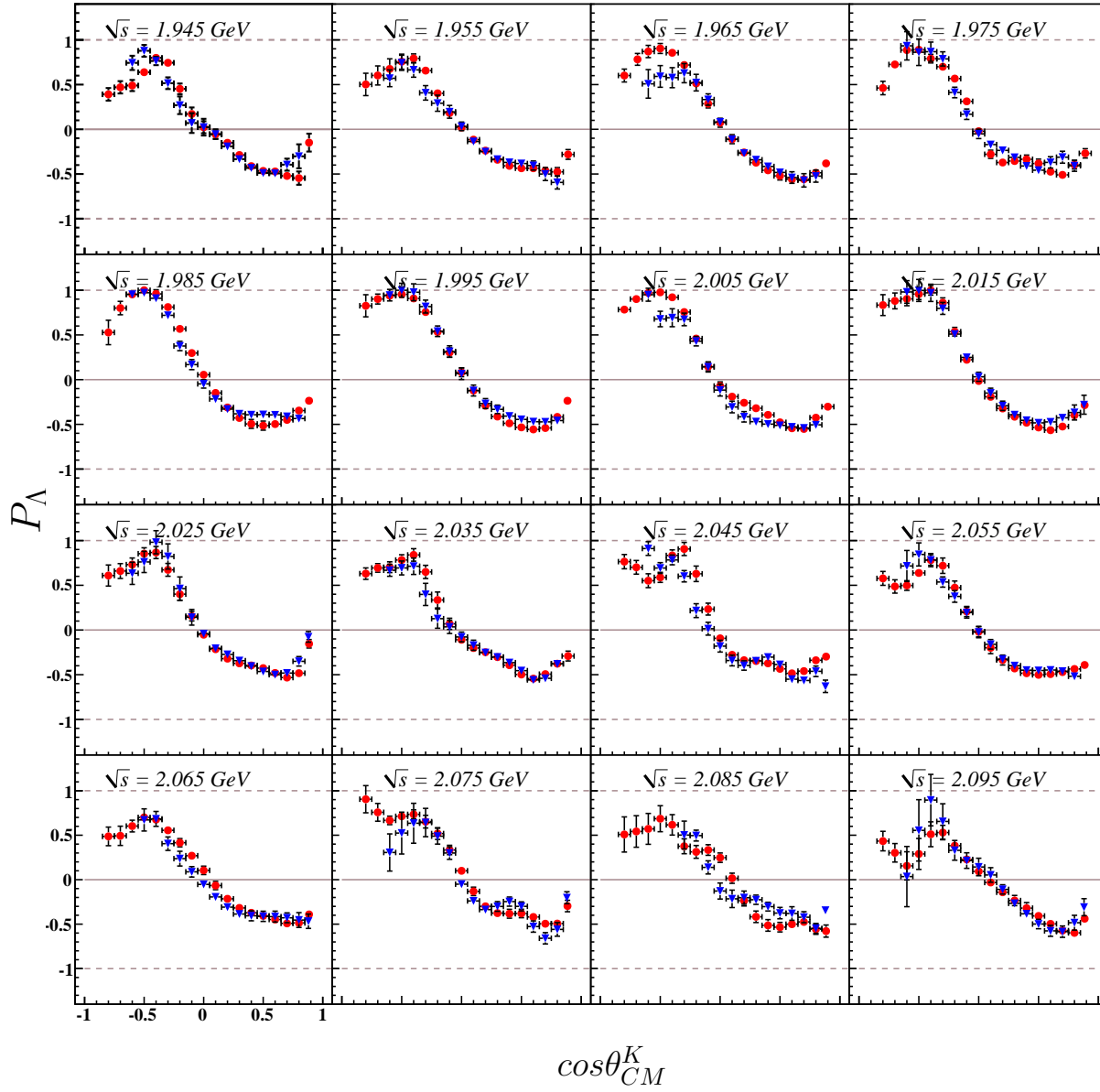
Figure 7.15: P_\Lambda v. \cos\theta_{CM}^K : \Lambda recoil polarization results v. \cos\theta_{CM}^{K^+} for the energy range 1.94 \text{ GeV} \leq \sqrt{s} < 2.10 \text{ GeV} . Results from the three-track analysis are shown in blue (triangles), those of the two-track analysis in red (circles). Uncertainties displayed are estimated from the scatter of results (see text).
