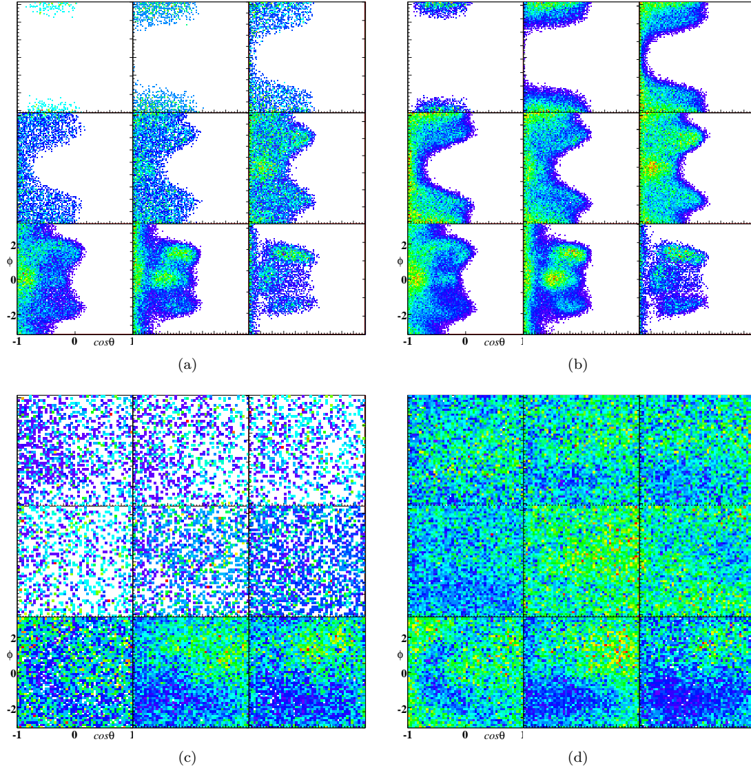
Figure 7.2: Shown above are plots of \phi_{\Lambda HF}^p v. \cos\theta_{\Lambda HF}^p for data and weighted accepted Monte Carlo in bins of \cos\theta_{CM}^K . Plots (a) and (b) show the data and Monte Carlo events (respectively) in the range 2.000 \text{ GeV} \leq \sqrt{s} < 2.050 \text{ GeV} from the three-track final-state topology. Plots (c) and (d) show the data and Monte Carlo events in the range 2.500 \text{ GeV} \leq \sqrt{s} < 2.550 \text{ GeV} from the two-track final-state topology. In each figure, each of the nine plots represents a 0.2-unit-wide bin in \cos\theta_{CM}^K , from backward angles at top left to forward angles at bottom right. The axes in all plots show the same ranges ( -\pi \leq \phi \leq \pi , -1.0 \leq \cos\theta \leq 1.0 ). All correlations present in the data are represented in the weighted Monte Carlo.
