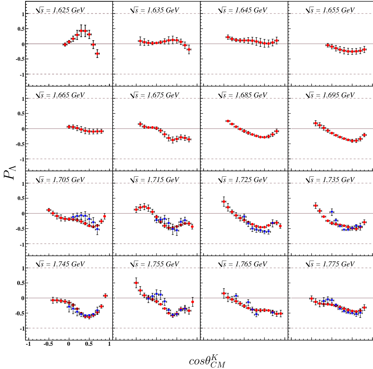
Figure 7.13: P_\Lambda v. \cos\theta_{CM}^K : \Lambda recoil polarization results v. \cos\theta_{CM}^{K^+} for the energy range 1.62 \text{ GeV} \leq \sqrt{s} < 1.78 \text{ GeV} . Results from the three-track analysis are shown in blue (triangles), those of the two-track analysis in red (circles). Uncertainties displayed are estimated from the scatter of results (see text).
