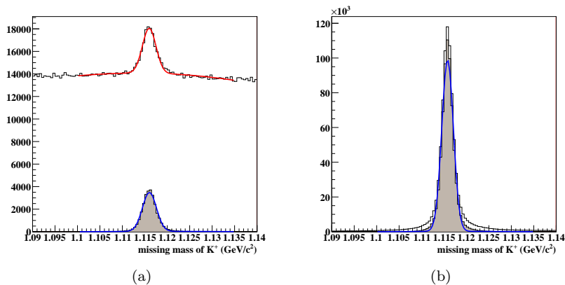
Figure 5.3: The histograms in (a) show the missing mass off K^+ distribution for all events in runs 4381-43819 of g11a before (unshaded) and after (shaded) a 1% confidence level cut is applied. Fits to a Gaussian and fourth-order background are shown in blue and red. The histograms in (b) show Monte Carlo events before and after the confidence level cut. A fit to a Gaussian is displayed in blue.
