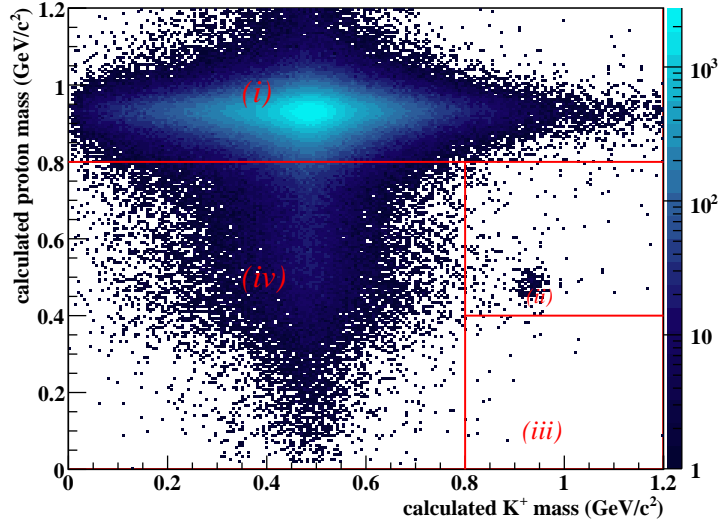
Figure 5.4: Shown above is the calculated proton mass versus calculated K^+ mass distribution for all Monte Carlo events. The number of events in regions (ii) and (iii) , those cut by our particle identification cuts, is very small.
