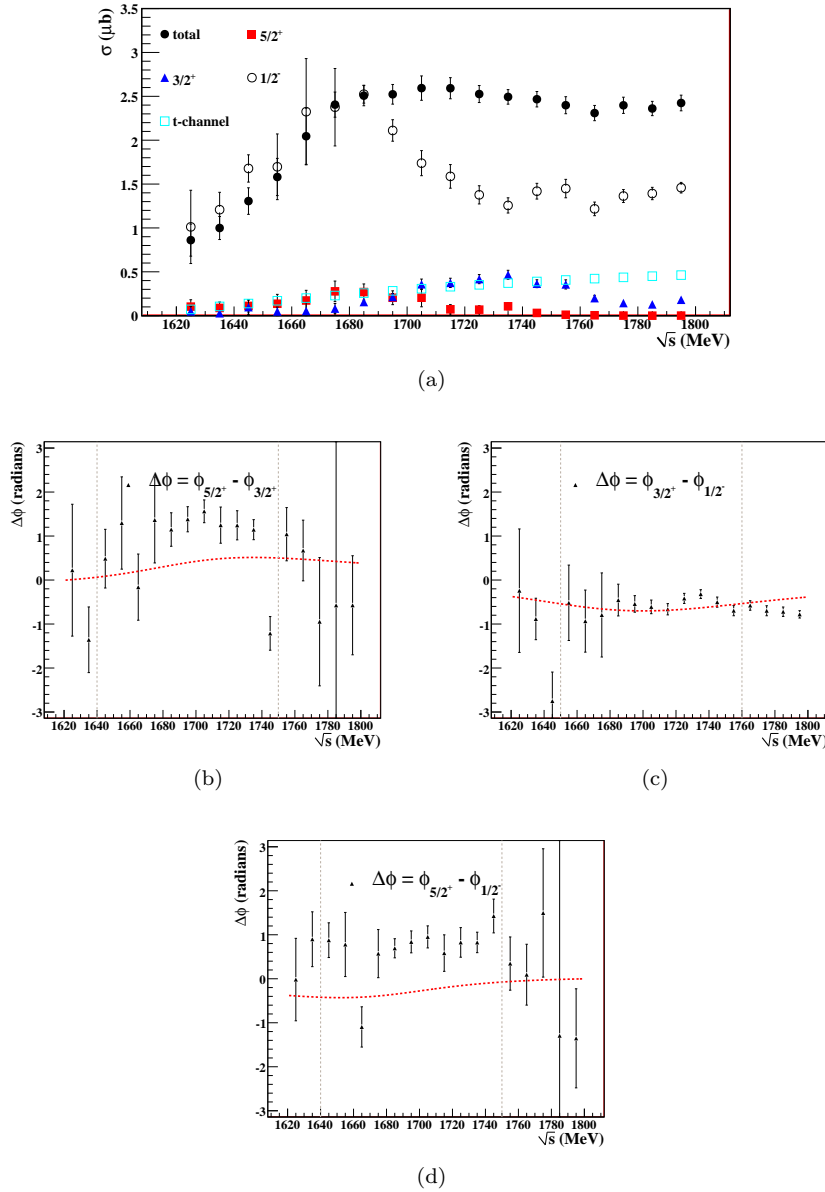
Figure 9.21: Shown above are the intensities (a) and phase differences (b-d) from the three-wave fit with alternate non-resonant model. In plots of phase differences, the vertical dashed lines indicate \sqrt{s} regions considered in the previous fit. Dashed red curves indicate the theoretical phase motion given by PDG average values.
