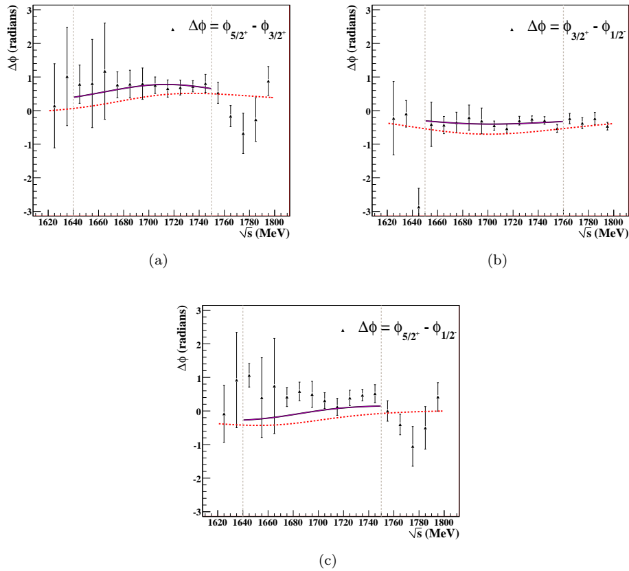
Figure 9.13: Shown above are the phase differences for each pair of s -channel waves in the fit with \frac{5}{2}^+ , \frac{3}{2}^+ , and \frac{1}{2}^- . The relevant waves are listed on each plot. Dashed red curves represent the theoretical phase motion using PDG average mass and width parameters. The solid magenta curves represent a fit of the theoretical phase motion allowing mass and width parameters within PDG limits.
