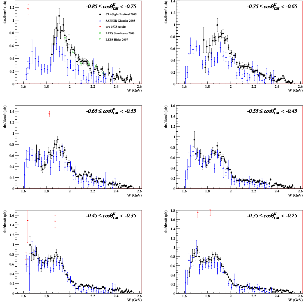
Figure 2.3: Shown above are previous measurements of the \gamma p \rightarrow K^+ \Lambda differential cross section at backward angles. Each plot displays data in a 0.1-unit-wide \cos \theta_{CM} range versus \sqrt{s} . The legend at top left indicates the convention for all plots.
