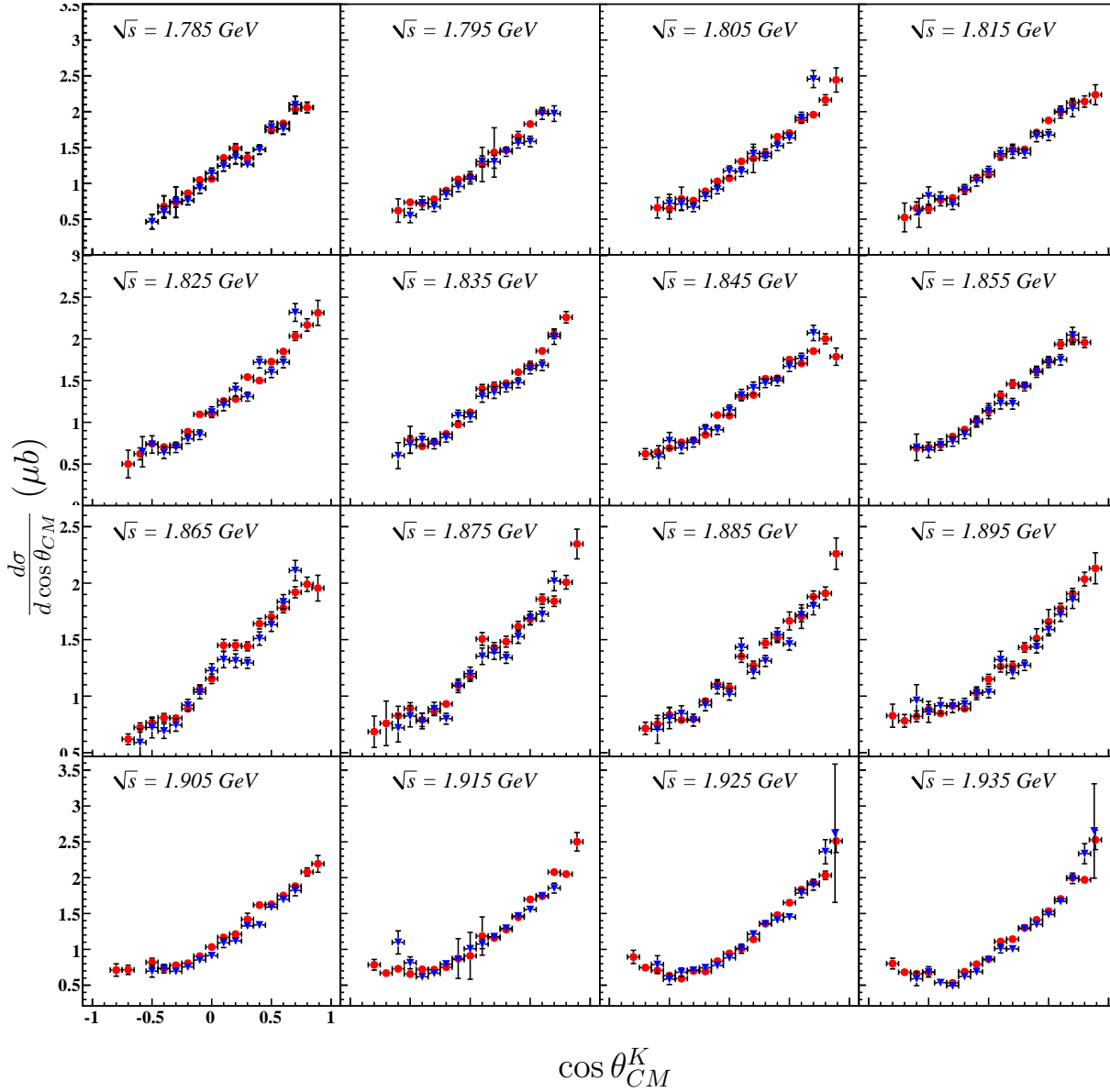
Figure 7.4: d\sigma/d\cos\theta_{CM}^K ( \mu\text{b} ) v. \cos\theta_{CM}^K : Differential cross section results for the energy range 1.78\text{ GeV} \leq \sqrt{s} < 1.94\text{ GeV} . Results from the three-track analysis are shown in blue (triangles), those of the two-track analysis in red (circles). All plots have the same \cos\theta_{CM}^K -axis range and vertical axis ranges are the same for the four plots in each row.
