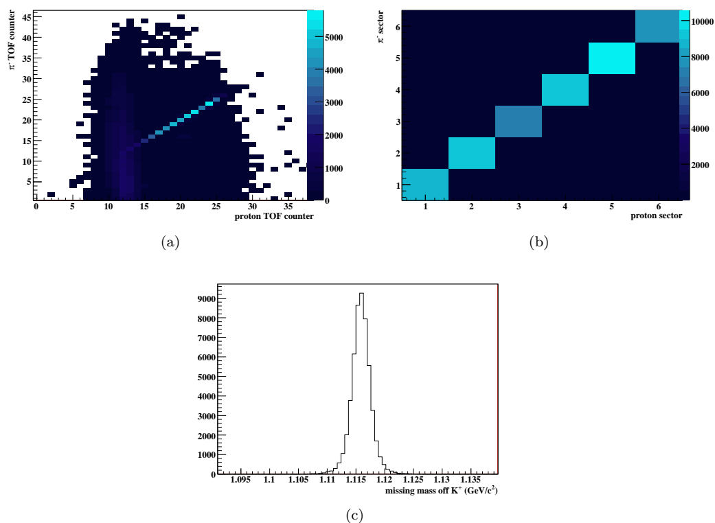
Figure 4.7: The plots above show (a) \pi^- TOF counter v. proton TOF counter, (b) \pi^- sector v. proton sector, and (c) the missing mass off K^+ distribution for events in region (iv) of the calculated mass plane (see Fig 4.6). The skewed proton calculated mass in this region is due to the proton and \pi^- hitting the same TOF paddle.
