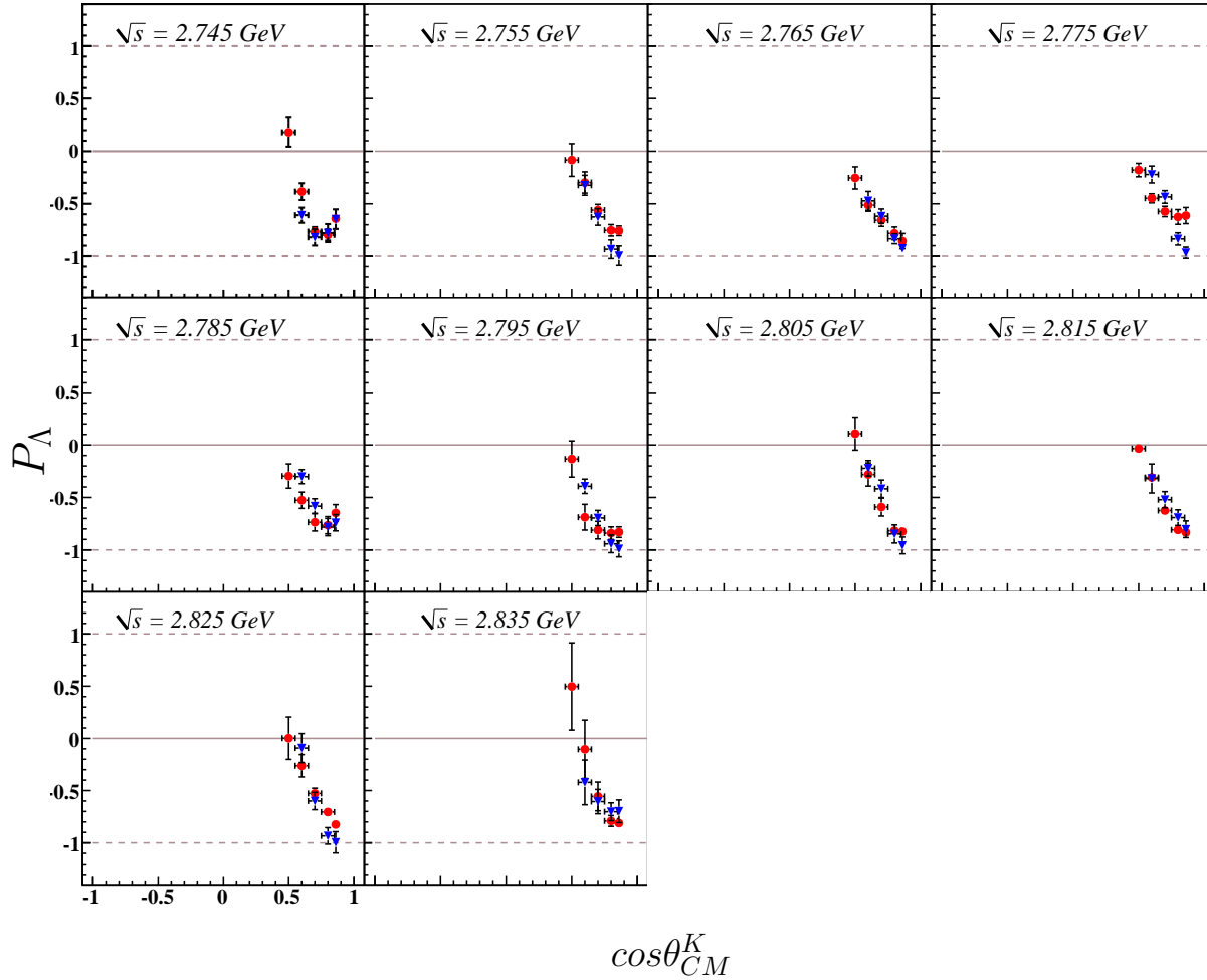
Figure 7.20: P_\Lambda v. \cos\theta_{CM}^K : \Lambda recoil polarization results v. \cos\theta_{CM}^{K^+} for the energy range 2.74 \text{ GeV} \leq \sqrt{s} < 2.84 \text{ GeV} . Results from the three-track analysis are shown in blue (triangles), those of the two-track analysis in red (circles). Uncertainties displayed are estimated from the scatter of results (see text).
