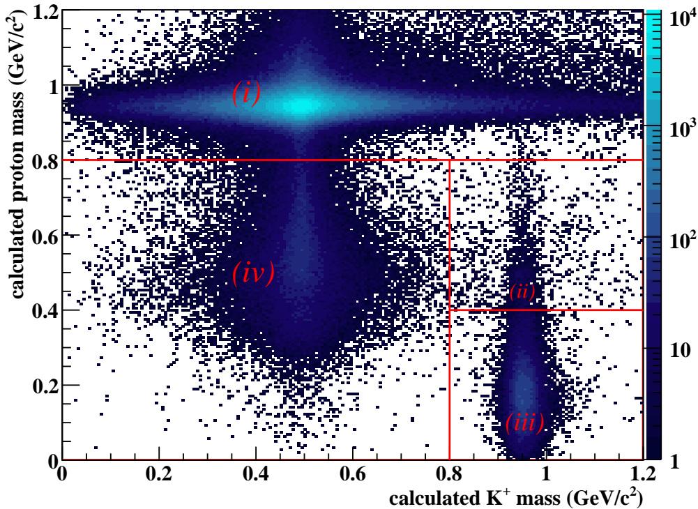
Figure 4.6: This plot shows the calculated mass for proton tracks versus the calculated mass for K^+ tracks for events in our K^+p\pi^- skim of g11a . The plane is broken into four regions described in the text.
