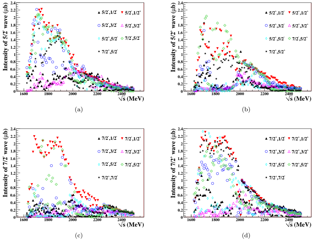
Figure 9.9: Shown above are the intensities of individual s -channel waves when fit with the wave combinations indicated. For example, plot (b) shows the intensity of the \frac{5}{2}^+ partial wave when fit with each of the other waves indicated. From this plot, we see that the \frac{5}{2}^+ wave displays a significant intensity at \sqrt{s} = 2.0 GeV in all fits, but its intensity is lowest when paired with the \frac{5}{2}^- partial wave. Shown are the J^P = \frac{5}{2}^- (a), \frac{5}{2}^+ (b), \frac{7}{2}^- (c), and \frac{7}{2}^+ (d) partial waves.
