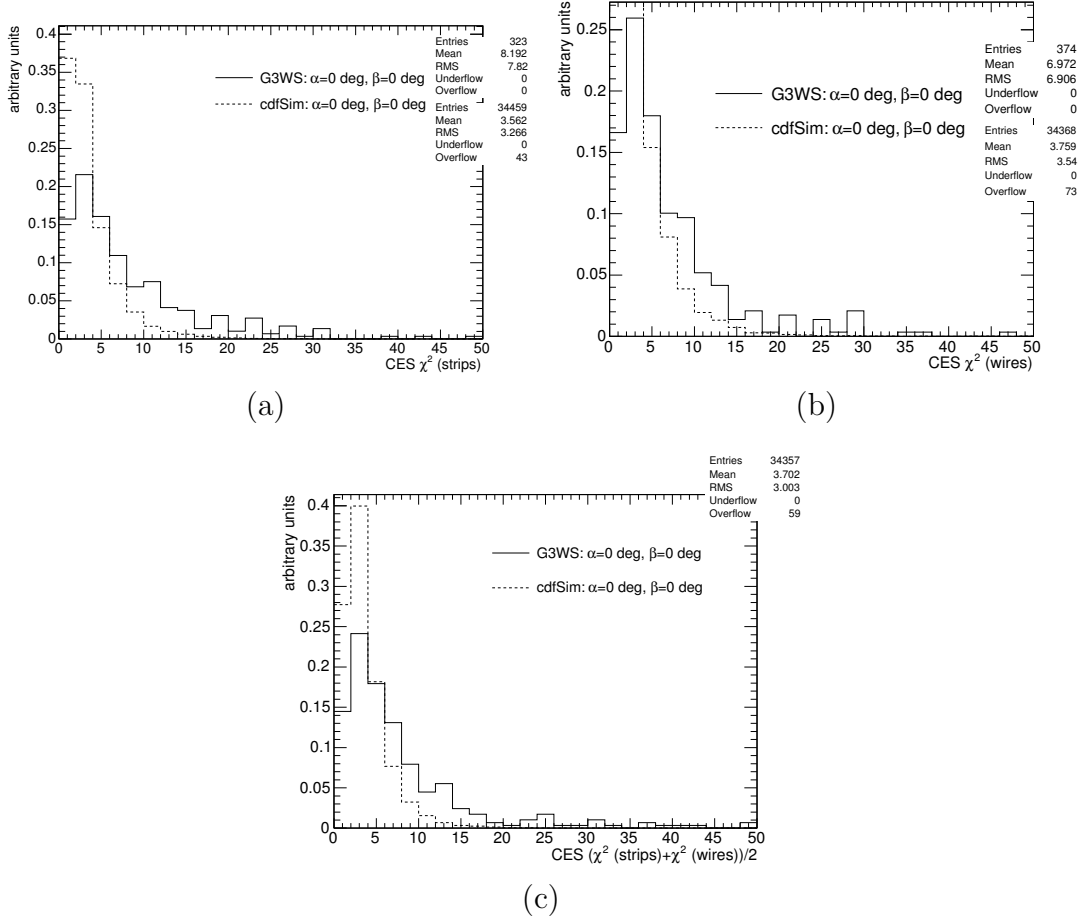
Figure 24: A comparison of the \text{CES } \chi^2 distributions for a photon of energy 50 GeV that propagates from a fixed vertex into a fixed tower in the CEM (wedge 0, tower 1) at 0^\circ incident angle, simulated with G3WS, and the distribution from the CDF MC separately for strips (a), wires (b) and combined (c). If simulated correctly, both should yield the same distributions, however, there is clearly a mismatch, in particular in the strips. This leads to an overestimate of the combined \chi^2 and to an underestimate of the \chi^2 efficiency for G3WS.
