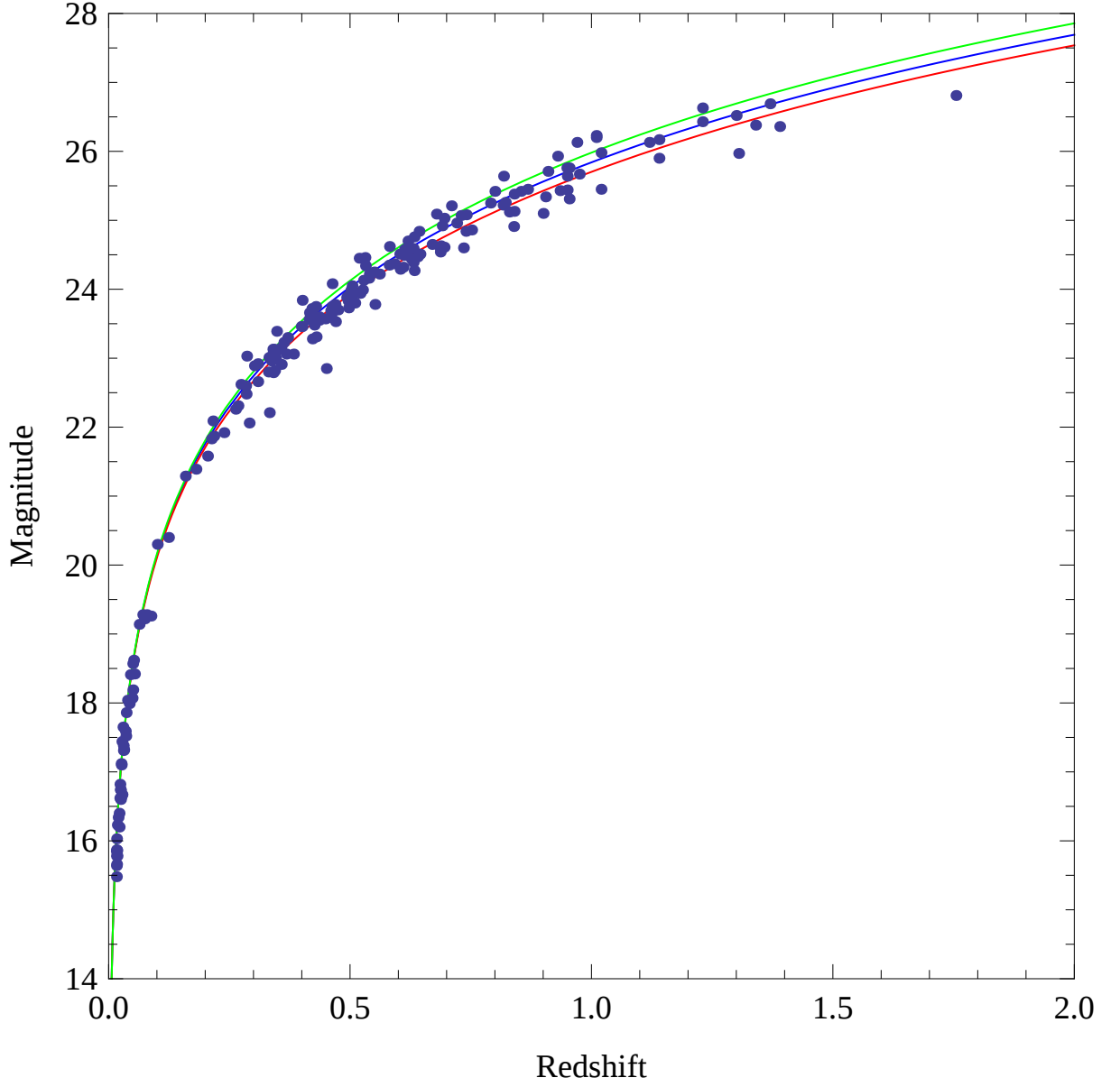
Figure 3.3: Plot of magnitude vs. redshift for (from top to bottom curve) \Lambda CDM (green), DGP (blue) and the AC model (with \alpha = 0.702 , \beta = 0.702 ) (red), along with the ESSENCE supernova redshift data. \Omega_m = 0.27 .
