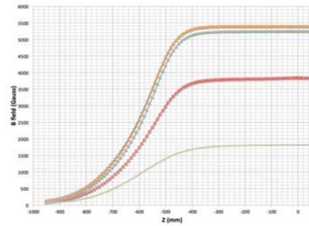
(b) Longitudinal scan of the magnetic field at different transverse positions.
