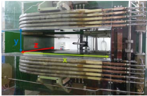
(a) Picture of the PADME dipole. The used coordinate system is also indicated.
