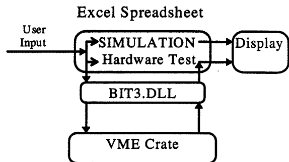
Fig. 1. Functional diagram of Test System. Simulation and hardware test occur in the Excel Spreadsheet, the BIT3.DLL drives the Bit3 hardware. The VME crate contains the system under test.
