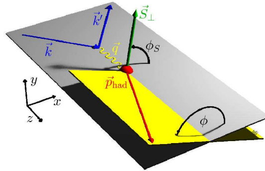
Fig. 2. Definition of the angles: the angle \phi ( \phi_S ) is the azimuthal angle of the scattered hadron (the target spin vector) around the virtual photon with respect to the lepton scattering plane.
