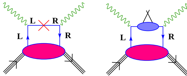
Fig. 1. Left-hand side: the chirality flip is forbidden by chirality conservation. Right-hand side: a chiral odd object preserves chirality.
