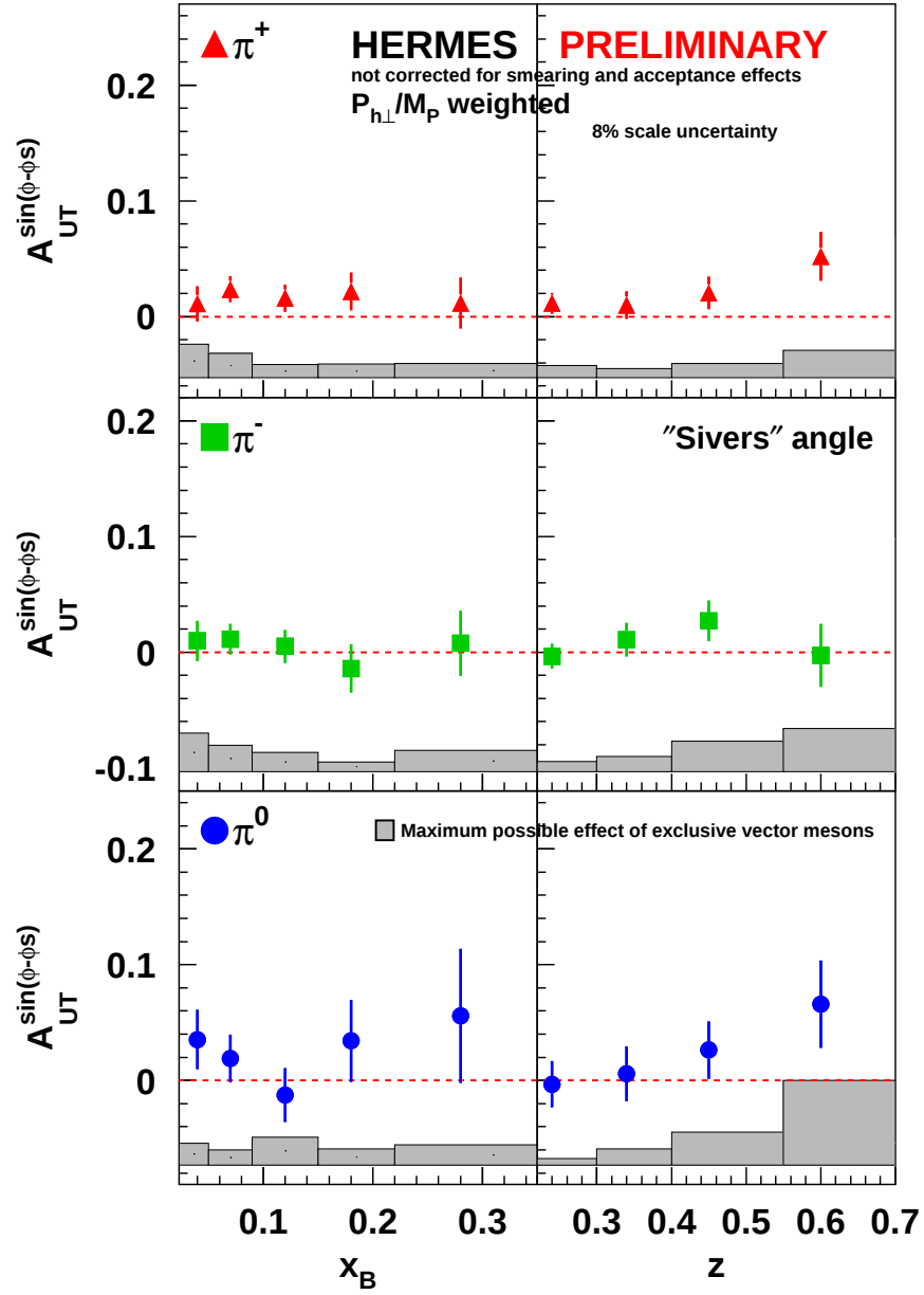
Fig. 4. Sivers asymmetries A_{UT}^{\sin(\phi-\phi_S)} for \pi^+ , \pi^- and \pi^0 as a function of x and z . Notations are as in Fig. 3.
