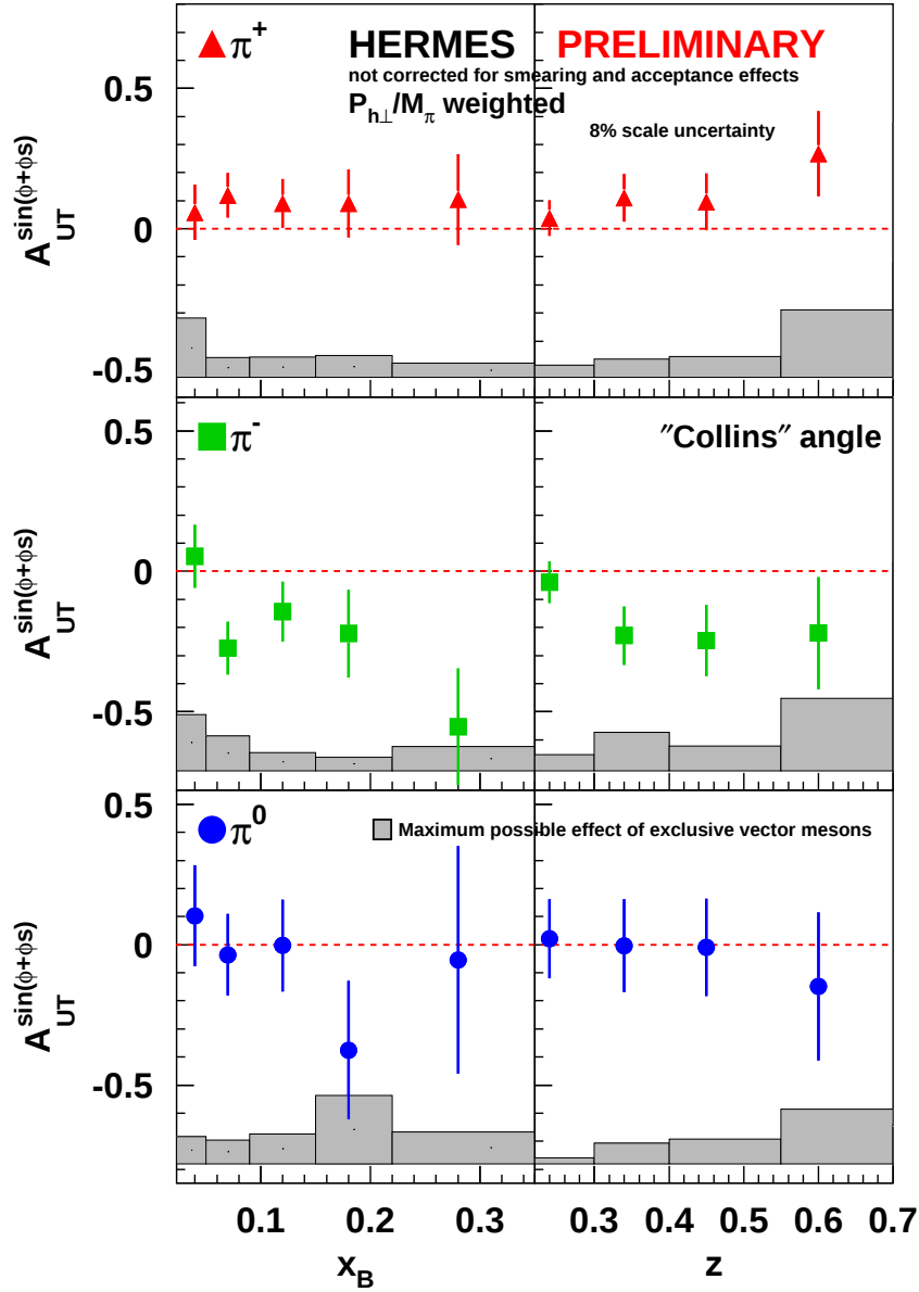
Fig. 3. Collins Asymmetries A_{UT}^{\sin(\phi+\phi_S)} for \pi^+ , \pi^- and \pi^0 as a function of x and z ( z is the energy fraction of the detected hadron w.r.t. the energy of the real photon). The error bars represent the statistical uncertainties, while the lower bands represent the possible interpretive uncertainties from diffractive vector meson production.
