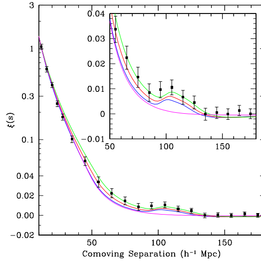
Figure 1.3: The correlation function for SDSS luminous red galaxies with the BAO peak at r \sim 110h^{-1}\text{Mpc} (Eisenstein et al., 2005). The lines show different cosmologies with \Omega_{\text{m}}h^2 = 0.12 (top line), 0.13 (second line) and 0.14 (third line) with \Omega_{\text{b}}h^2 = 0.024 and n_s = 0.98 in all cases. The bottom line represents a pure cold dark matter model \Omega_{\text{m}}h^2 = 0.105 with no acoustic peak.
