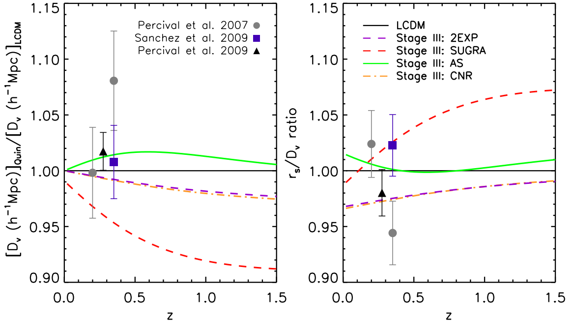
Figure 3.15: The ratio of the distance measure D_v(z) (left panel) and the ratio of r_s(z_d)/D_v (right panel) for four quintessence models compared to \Lambda CDM as indicated by the key in the right hand panel. The grey circles are estimate points from Percival et al. (2007) at z = 0.2 and z = 0.35 measured using the observed scale of BAO calculated from the SDSS and 2dFGRS main galaxy samples. Sánchez et al. (2009) combined CMB data with information on the shape of the redshift space correlation function using a larger LRG dataset and found D_v(z = 0.35) = 1300 \pm 31 Mpc and r_s(z_d)/D_v = 0.1185 \pm 0.0032 at z = 0.35 (blue squares). The data points from Percival et al. (2010) for D_v and r_s(z_d)/D_v at z = 0.275 using WMAP 5 year data + SDSS DR7 are plotted as black triangles.
