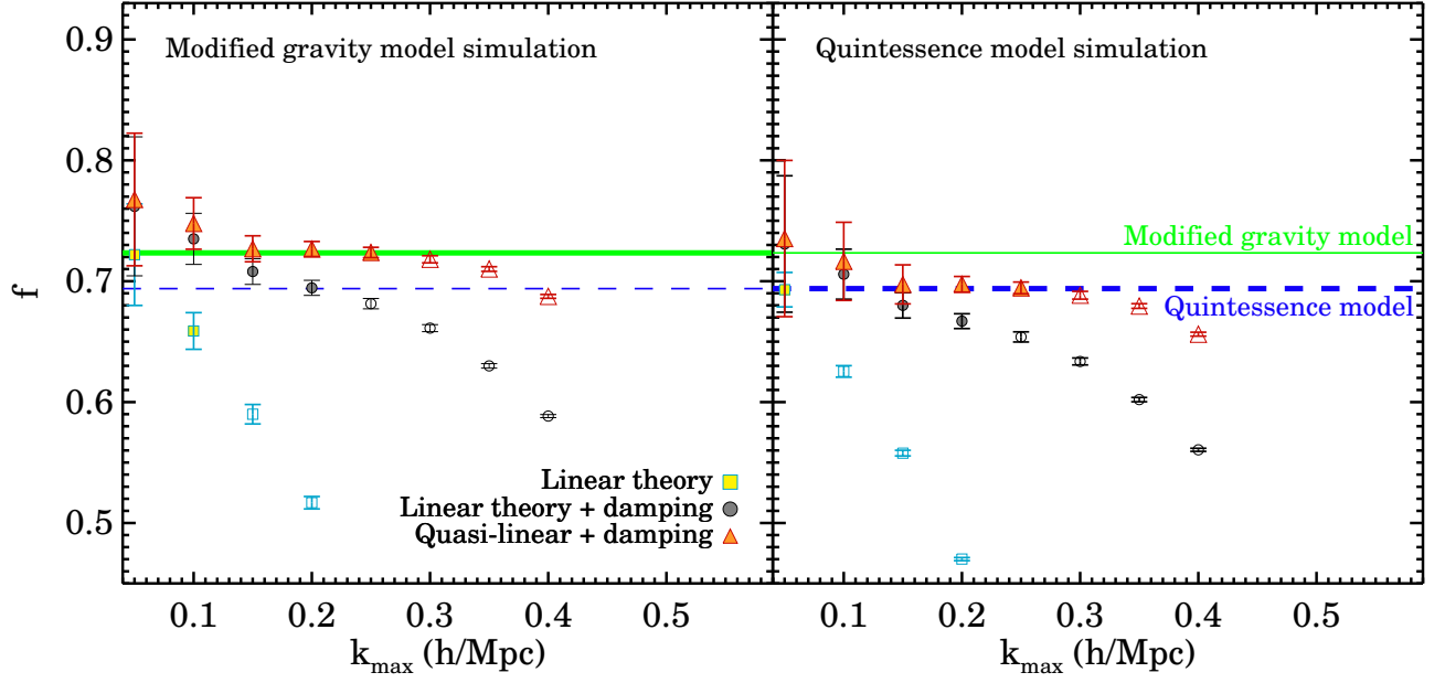
Figure 5.6: Measurements of the linear growth rate of cosmic structure, f . The results are plotted as a function of the maximum wavenumber, k_{\text{max}} (h/Mpc), used in the fit. The different symbols show the results of fitting to P_2/P_0 at z = 0.5 (see Fig. 5.3) using different models: linear theory - squares, linear theory plus damping - circles, quasi-linear plus damping - triangles. The symbols are filled in for scales over which the model is a good description of the measured ratio. The error bars represent the 1\sigma uncertainty in the fit. In the left hand panel we fit to the modified gravity model and aim to recover the true growth factor shown by the thick green horizontal line. In the right panel we fit to the ratio measured from the quintessence model, in which case the target growth factor is shown by the thick blue dashed line. The quasi-linear plus damping model performs best, recovering the correct growth factor in each case over the widest range of wavenumbers. This model is an accurate model of the simulation results up to k_{\text{max}} = 0.3h/\text{Mpc} . The linear and linear plus damping models are less successful, and only recover the correct answer over a very limited range of wavenumbers. Their application over a wider range of scales would lead to a systematic error in the growth factor similar to or larger than the difference in the growth factors between the two models.
