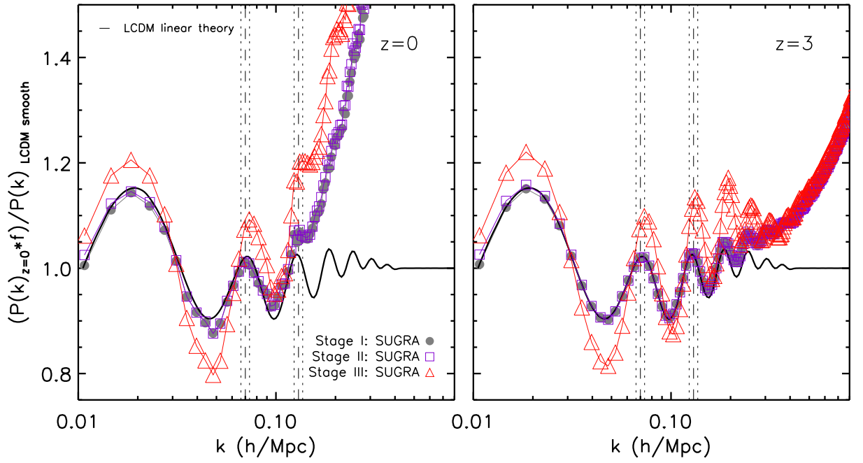
Figure 3.17: The real space power spectrum for the SUGRA model on large scales at z = 0 and z = 3 . All power spectra have been divided by a smoothed linear theory P(k) for \Lambda\text{CDM} . Stage I in our simulation is represented by grey circles, Stage II is represented by open purple squares and Stage III results are shown as red triangles. The black solid line represent the linear theory power spectrum in \Lambda\text{CDM} divided by the smooth reference spectrum. The vertical dashed (dotted) lines show the position of the first two acoustic peaks (positions \pm 5\% ) for a \Lambda\text{CDM} cosmology.
