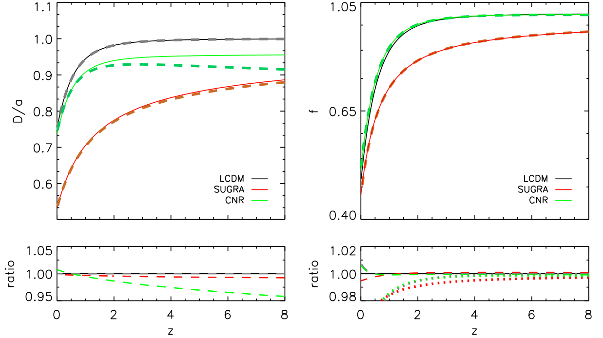
Figure 4.1: Left panel: The linear growth factor divided by the scale factor as a function of redshift for the SUGRA and CNR quintessence models and \Lambda CDM, as indicated by the key. Right panel: The linear growth rate, f = d\ln D/d\ln a , for the two dark energy models and \Lambda CDM as a function of redshift. In both the left and right main panels, solid lines represent the exact solution for the linear growth factor and growth rate and dashed lines show the fitting formula given in Eq. 4.1. Note in the right main panel the \Lambda CDM grey dashed line has been omitted for clarity. The lower left hand panel shows the formula for D(a)/a given by Linder (2005) divided by the exact solution as a function of redshift. The ratio of the formula in Eq. 4.1 for the growth rate, f , to the exact solution is shown in the lower right hand panel. Also in the lower right panel the dotted lines show the ratio of the fitting formula f = \Omega_m^{0.6} to the exact solution for each of the dark energy models plotted as a function of redshift.
