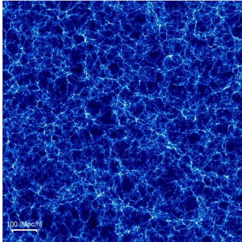
Figure 2.2: The dark matter distribution in a 100 \text{ Mpc}/h thick slice from a simulation using 646^3 particles to represent the dark matter distribution in box of 1500h^{-1}\text{Mpc} on a side at redshift z = 0 .
