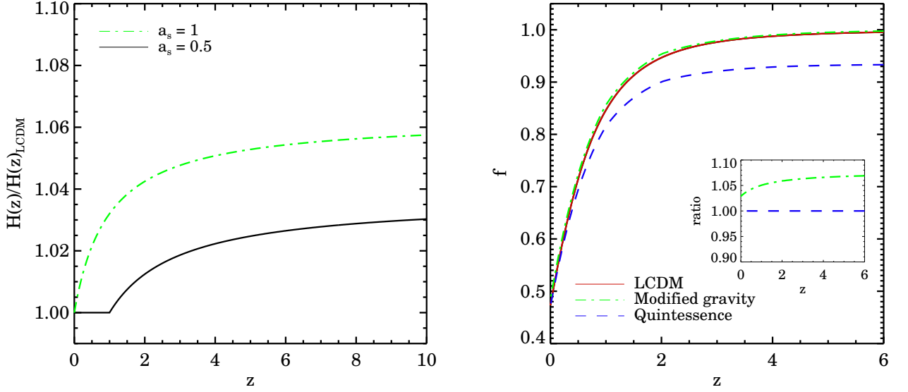
Figure 5.1: Left panel: The two different lines show the ratio of the expansion rate, H(z) , for two modified gravity models to the expansion rate in \Lambda CDM. In the left panel we plot the expansion history for a modified gravity model with parameters a_s = 1 ( a_s = 0.5 ), divided by H(z) for \Lambda CDM, as a green dot dashed (black solid) line. Right panel: The linear growth rate, f , as a function of redshift for \Lambda CDM, a modified gravity cosmology and a quintessence model. In the right panel, the linear theory growth rate is plotted as a function of time for a modified gravity model with a_s = 1 and \mu_0^2 = 1.13 in Eq. 5.8 (green dot dashed line). The growth rate for a quintessence model, which has the same expansion history as the modified gravity model, is plotted as a blue dashed line. The growth rate for \Lambda CDM is shown as a red solid line. The inset panel shows the ratio of f for the modified gravity model to the quintessence model as a function of redshift (green dot dashed line).
