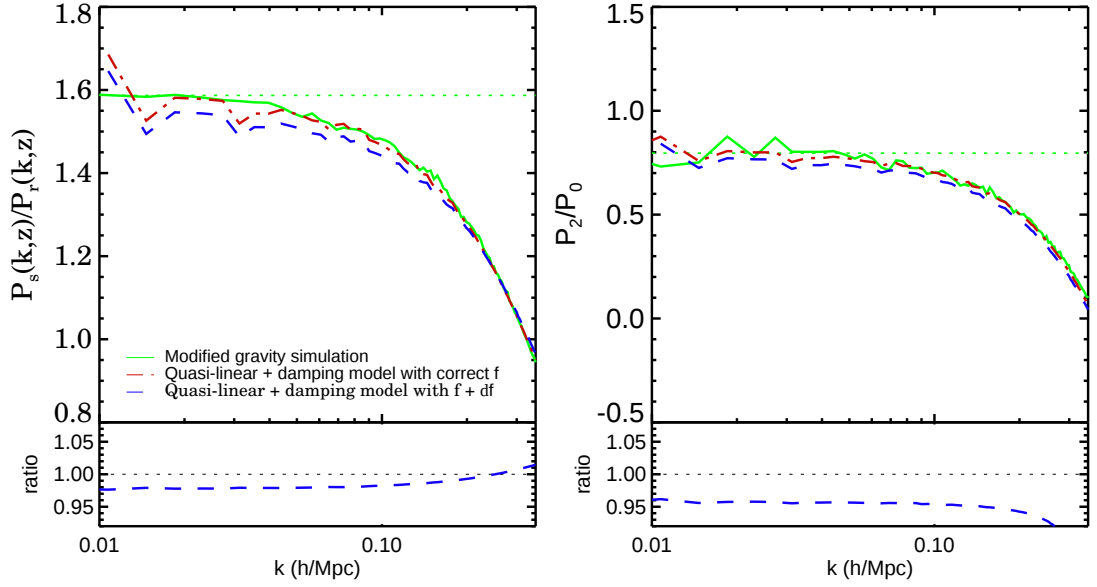
Figure 5.5: Left panel: The ratio of the monopole of the redshift space power spectrum to the real space power spectrum at z = 0.5 , as a function of wavenumber, k(h/\text{Mpc}) . Right panel: The ratio of the quadrupole to monopole moment of the redshift space P(k) at z = 0.5 , as a function of wavenumber. Both panels show the quasi-linear plus damping model for the ratios using different values for the linear growth rate, f . In both panels we plot the quasi-linear plus damping model using f = f_{\text{TRUE}} (red dot dashed) and f = 1.05f_{\text{TRUE}} (blue dashed), using the best fit value for \sigma_v in the range 0.01 \leq k(h/\text{Mpc}) \leq 0.25 . The blue dashed line in the bottom left and right panels show the ratio of the quasi-linear plus damping model using f = 1.05f_{\text{TRUE}} to the same model using f = f_{\text{TRUE}} for P_2^s/P_0^s and P_0^s/P_r respectively.
