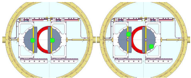
Figure 5: Possible positions of the two pairs of radiation monitors in green (not to scale). Both layouts meet the criteria well, with the rightmost design allowing a greater cross-sectional area to be sampled, but a more complex cabling system must be used. The coaxial cables that connect to the detectors can be connected to the white frame and fed out via the four way flanges. The pre-amplifiers can be mounted inside the vessel (beige outer ring) inside the vacuum.
