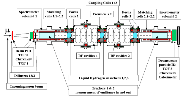
Figure 1: Schematic of the International Muon Ionisation Cooling Experiment (MICE), with the beam entering from the left.
