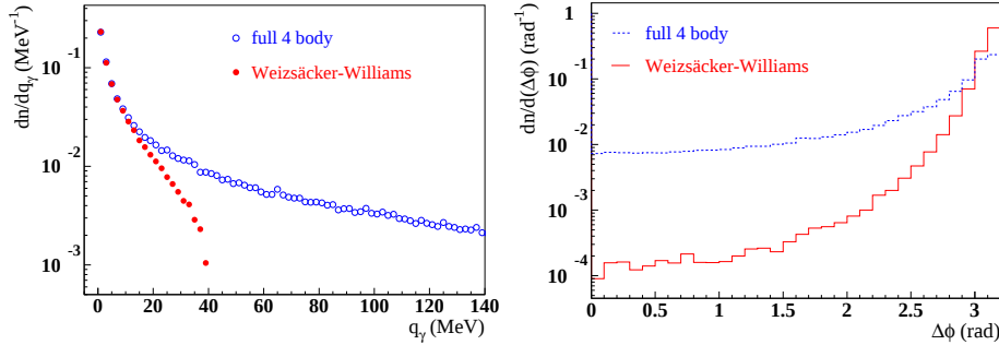
Fig. 1. Comparison between the full 4 body and the Weizsäcker–Williams evaluations for e^+e^- \rightarrow e^+e^-\pi^0\pi^0 , in the virtual photon momentum (left) and in the azimuth difference of the two pions (right).
