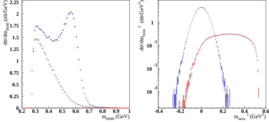
Fig. 3. Comparison between e^+e^- \rightarrow e^+e^-\pi^0\pi^0 (lighter histogram) and e^+e^- \rightarrow \omega\pi^0 \rightarrow \pi^0\pi^0\gamma (darker histogram) in the \pi\pi invariant mass (left) and in the missing mass (right).
