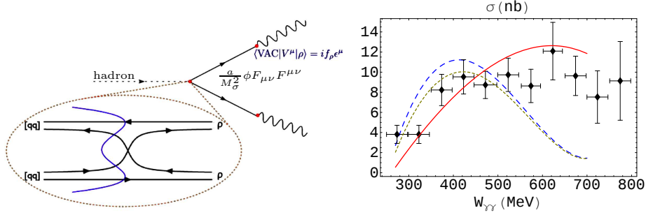
Fig. 2. A schematic view of the \gamma\gamma \rightarrow \sigma transition (left). Comparison of the Crystal Ball \sigma_{\gamma\gamma \rightarrow \pi^0\pi^0} data points with predictions from ChPT (solid), Breit-Wigner with (dotted) and without (dashed) the Adler zero (right).
