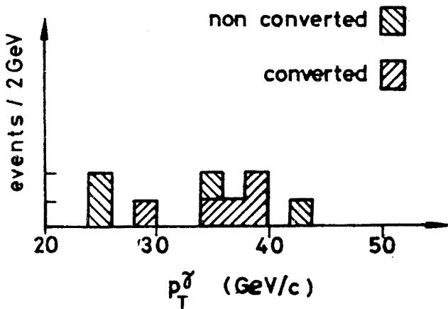
Fig. 3. \not{p}_T -spectrum of the monophoton candidates. For interpretation see text
