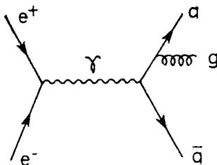
Fig. 5. An O(\alpha_s) diagram for the gluon bremsstrahlung process e^+e^- \rightarrow q\bar{q}g
