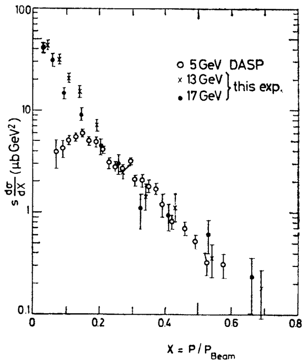
Fig. 4. Comparison [4] of x -distributions of charged particles at Q = 5, 13 and 17 GeV
