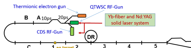
Figure 1: Layout of Linac.
