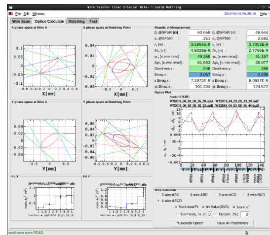
Figure 7: Wire scan measurement of 5 sector.
