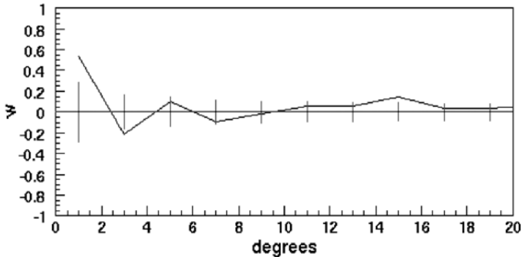
Fig.10. The two point autocorrelation function for the stereo data. w(\theta) = N(\theta)/N_{MC}(\theta) - 1 . The error bars on the w = 0 line represent the size of 1\sigma fluctuations.
