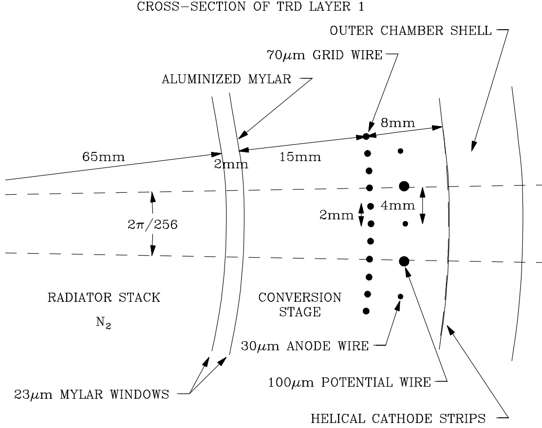
Figure 3.5: A cross section of the TRD.
