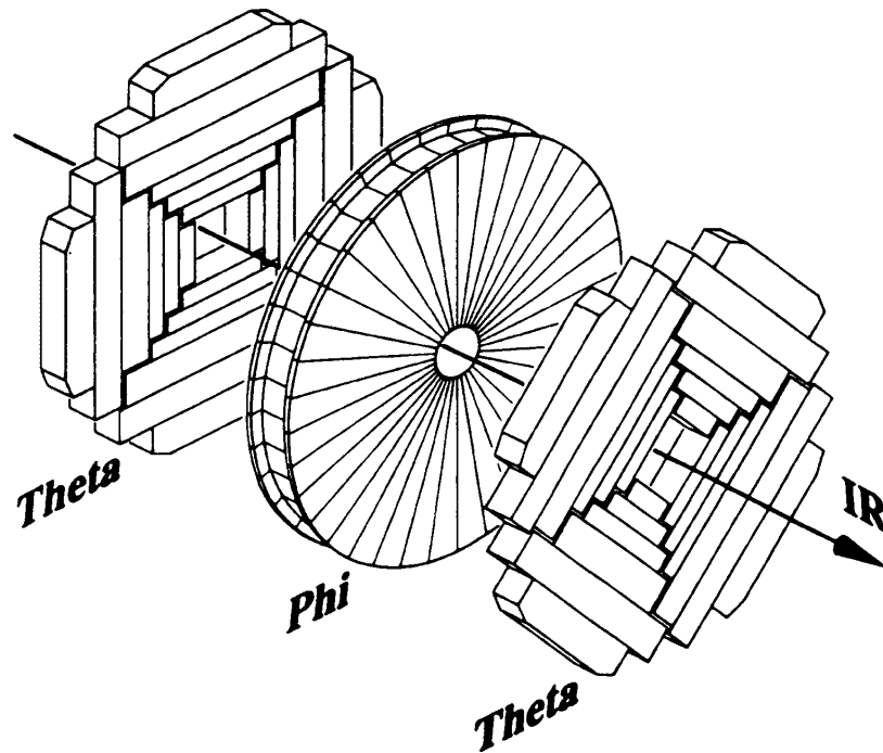
Figure 3.7: Exploded view of one of the forward drift chambers.
