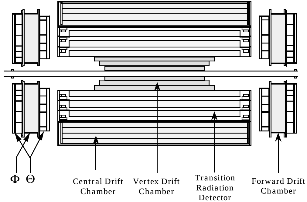
Figure 3.3: The four systems that comprise the central detector.
