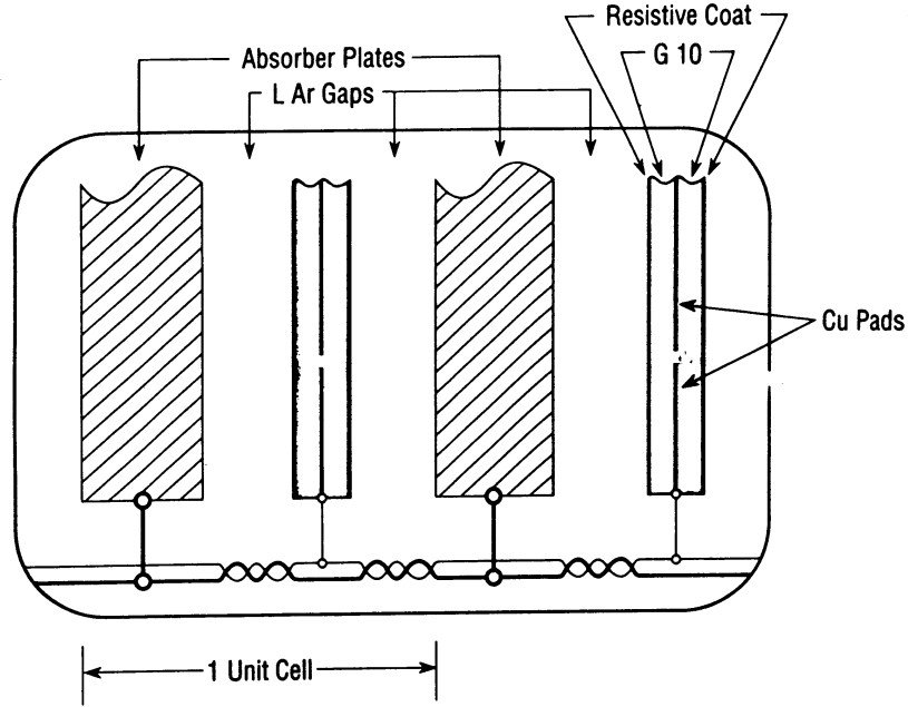
Figure 3.9: Schematic view of a typical uranium liquid argon readout cell.
