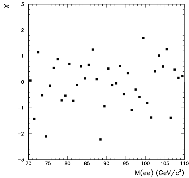
Figure 6.8: The comparison of the data and Monte Carlo versus the invariant mass. The variable \chi is equal to number of events minus the number of Monte Carlo events over the square root of the number of data events.
