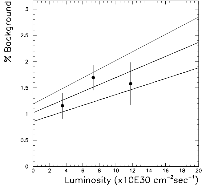
Figure 7.11: The QCD background as a function of the luminosity. The luminosity bins are 0-5, 5-10, and 10+ in units of 10^{30} \text{ cm}^{-2} \text{ sec}^{-1} .
