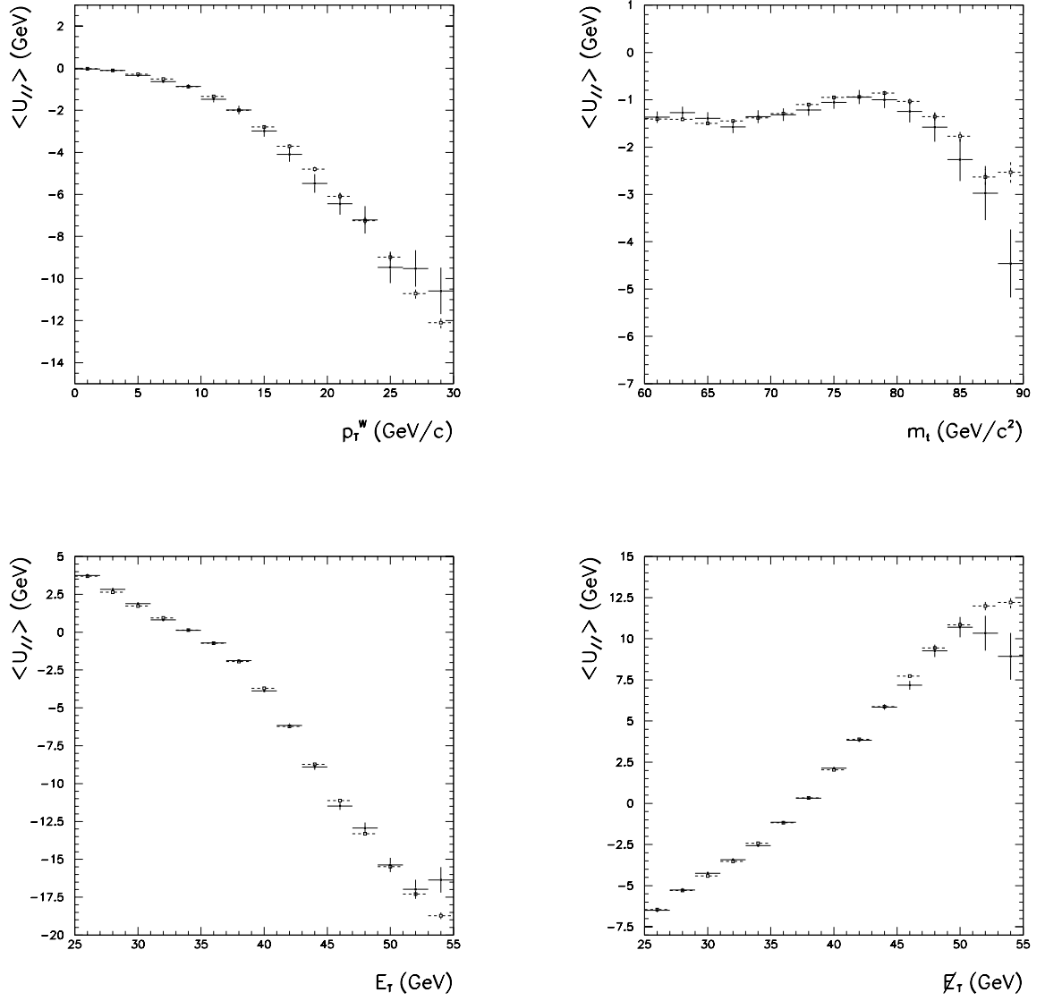
Figure 5.16: The mean U_{\parallel} versus the p_T^W , m_t , E_T , and E_T for the CC W boson events. The solid dots are the data and the open dots are the Monte Carlo simulation.
