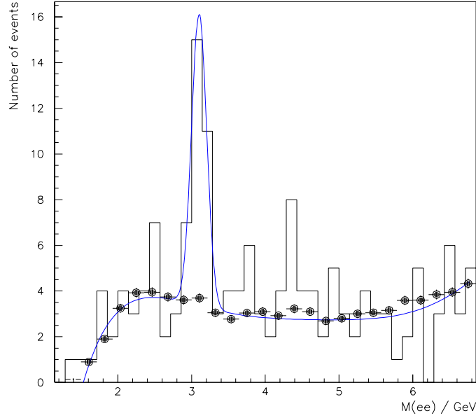
Figure 6.3: The dielectron mass distribution for the J/\psi events. The histogram is the data and the dots are the expected background. The solid line is the fit to the peak plus the background shape.
