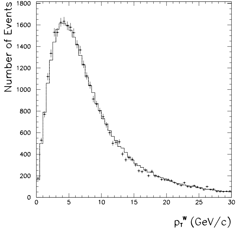
Figure 5.14: The solid points the are data and the histogram is the Monte Carlo for the recoil vector in the W boson events.
