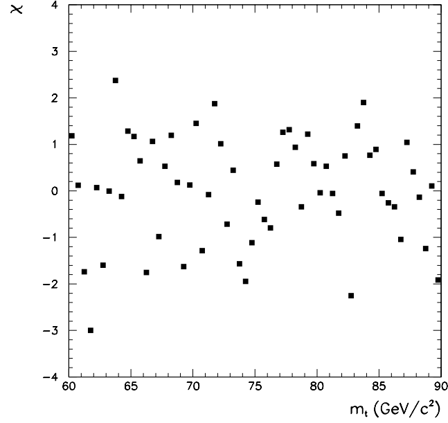
Figure 7.3: The comparison between the Monte Carlo and data as a function of the transverse mass.
