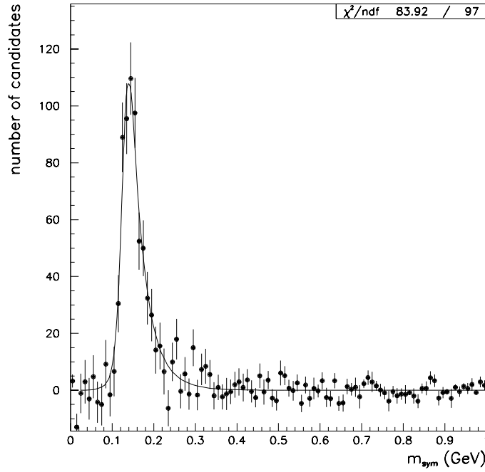
Figure 6.2: The background subtracted symmetric mass distribution from the \pi^0 decays. The dots are the data and the solid line the Monte Carlo simulation.
