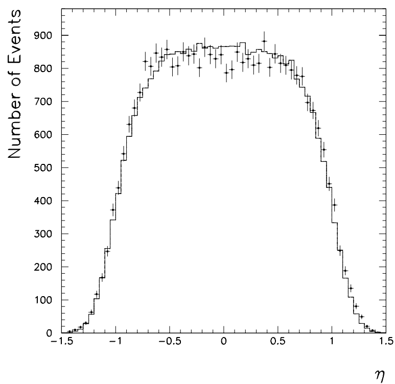
Figure 5.17: The rapidity distribution of the electron in CC W boson events. The histogram is the Monte Carlo and the dots are the data.
