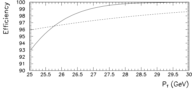
Figure 5.13: The electron and missing p_T trigger turn on curves. The solid line is the electron turn on curve and the dashed line is the missing p_T turn on curve.
