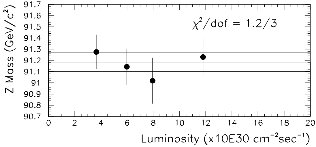
Figure 7.15: The Z boson mass as a function of the luminosity. The central line in the fit is the mean value of the four data points and the two outer lines the statistical error.
