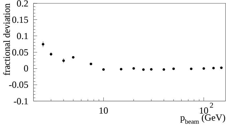
Figure 6.1: Fractional deviation of the electron energy versus the momentum from the test beam. The deviation is from the function given in equation 6.3 where E^{True} is equal to p_{beam} . The response is linear in the region of p_{beam} > 10 GeV/c and only deviates at low momentum.
