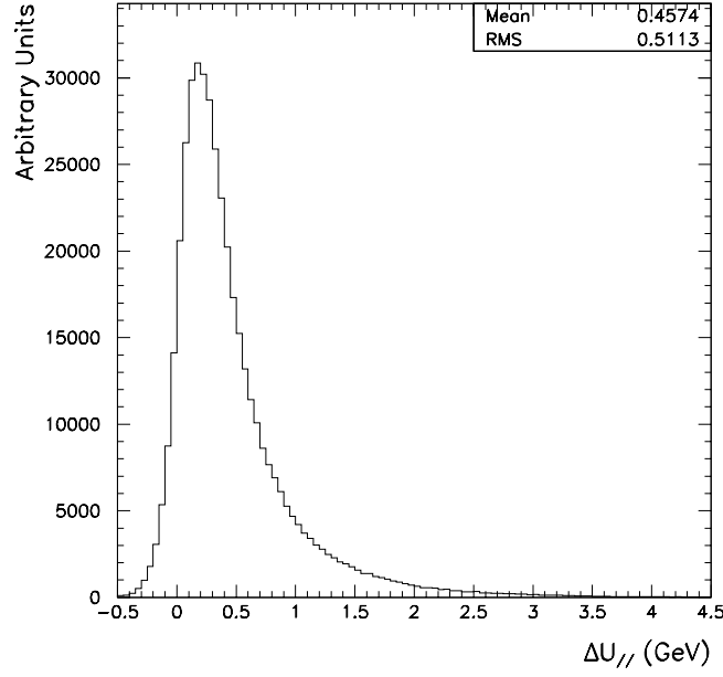
Figure 5.12: The distribution of \Delta U_{||} used in the Monte Carlo.
