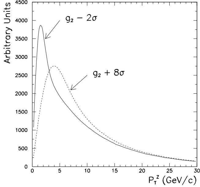
Figure 7.6: The variation of the p_T^Z distribution for two large excursions of the g_2 parameter.
