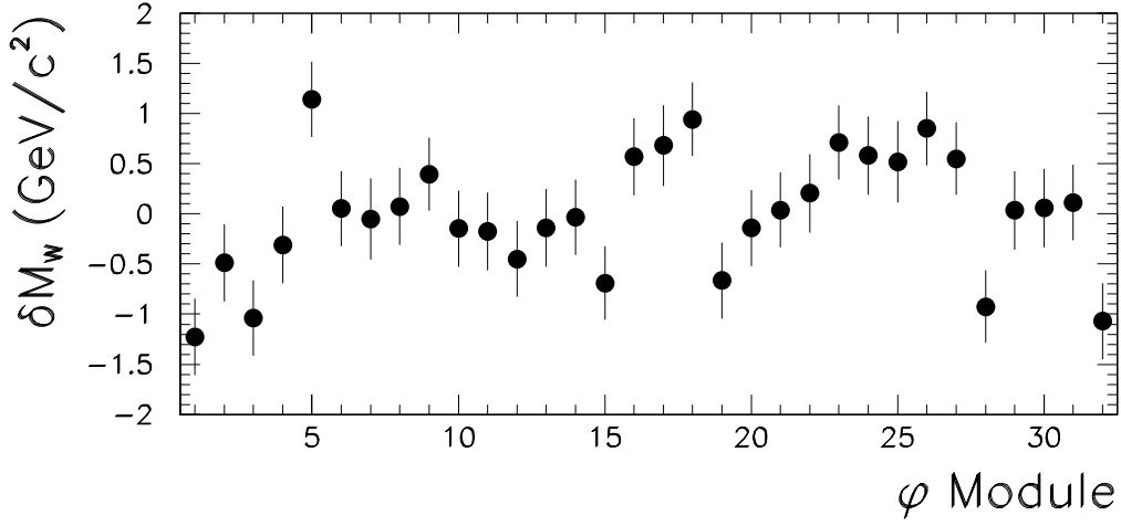
Figure 7.13: The variation of the W boson mass as a function of the \phi module of the central calorimeter.
