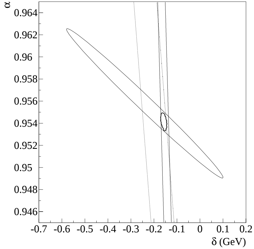
Figure 6.4: In the \alpha_{EM} - \delta_{EM} plane the 1\sigma contours for the three data sets. The solid ellipse lying on its side is the contour from the Z data. The thin, nearly vertical, solid ellipse is the contour for the \pi^0 data. The dotted ellipse is the contour for the J/\psi data. The small thick contour is the combination of all three data sets.
