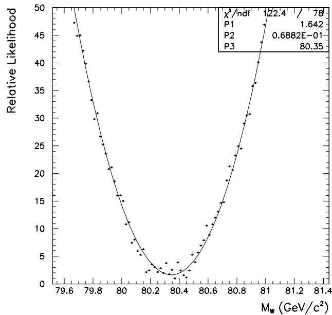
Figure 7.2: The relative likelihood distribution as a function of the W boson mass. The fit is a second order polynomial where P2 is the error and P3 the fitted mass.
