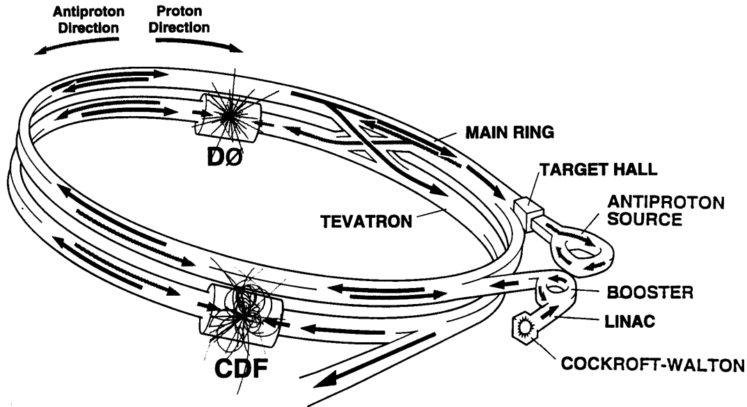
Figure 3.1: The Fermilab accelerators and experimental hall locations.
