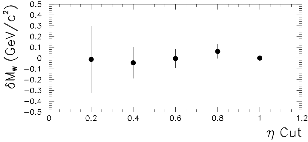
Figure 7.14: The variation of the W boson mass as a function of the lepton rapidity cut.
