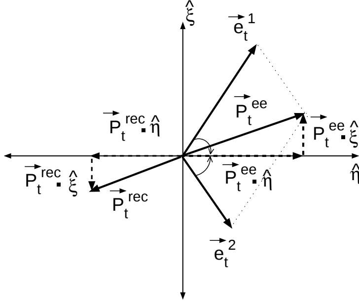
Figure 4.3: Definition of the useful axis and projections in a Z boson event. The \eta axis is the bisector of the electrons in the transverse plane and the \xi axis is perpendicular to the \eta axis.
