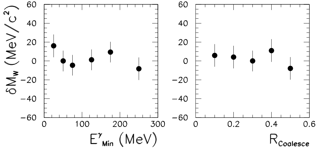
Figure 7.7: The variation of the W boson mass as a function of \gamma_{Min} (left) and R_{Coalesce} (right).
