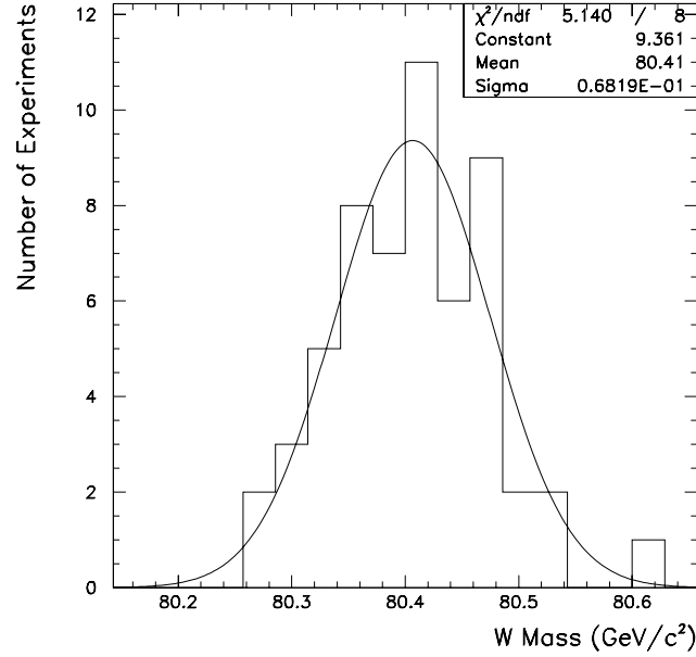
Figure 7.5: The distribution of fitted W boson masses for 56 experiments containing 30,000 events.
