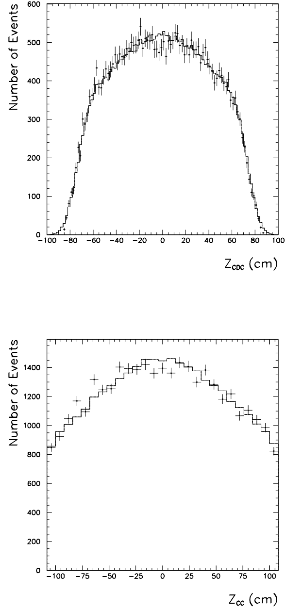
Figure 5.18: The distribution of the Z positions in the CDC (upper plot) and the calorimeter (lower plot).
