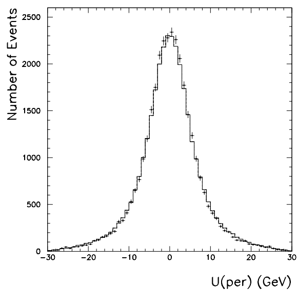
Figure 5.15: The comparison between the Monte Carlo and data for the U_{\parallel} and U_{\perp} distributions. Table 5.8 summarizes the mean and RMS values for the U_{\parallel} and U_{\perp} distributions.
