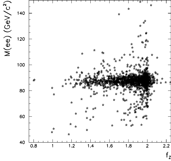
Figure 6.5: The invariant mass versus f_Z for the CC-CC Z boson events.
