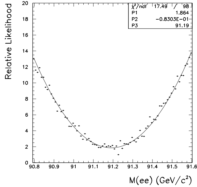
Figure 6.7: The relative likelihood distribution for the fit to the CC-CC Z boson events.
