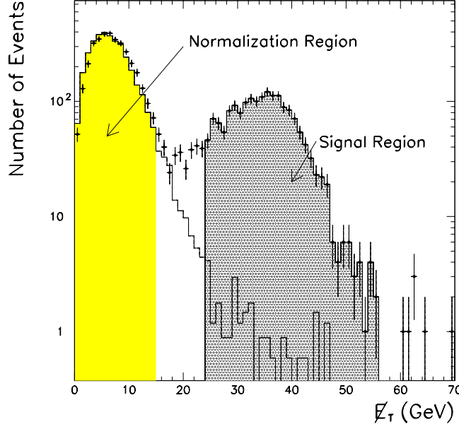
Figure 7.10: The \cancel{E}_T distribution of the good (dots) and bad (solid histogram) events. The two samples are normalized in the low \cancel{E}_T region. The amount of background is the ratio of the number of events in the signal region.
