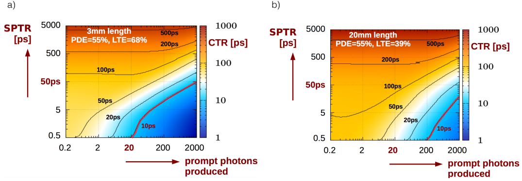
Figure 1. Cramér-Rao lower bound calculations for CTR using a LSO:Ce scintillator of (a) 3 mm and (b) 20 mm length as function of SPTR and number of prompt photons.
